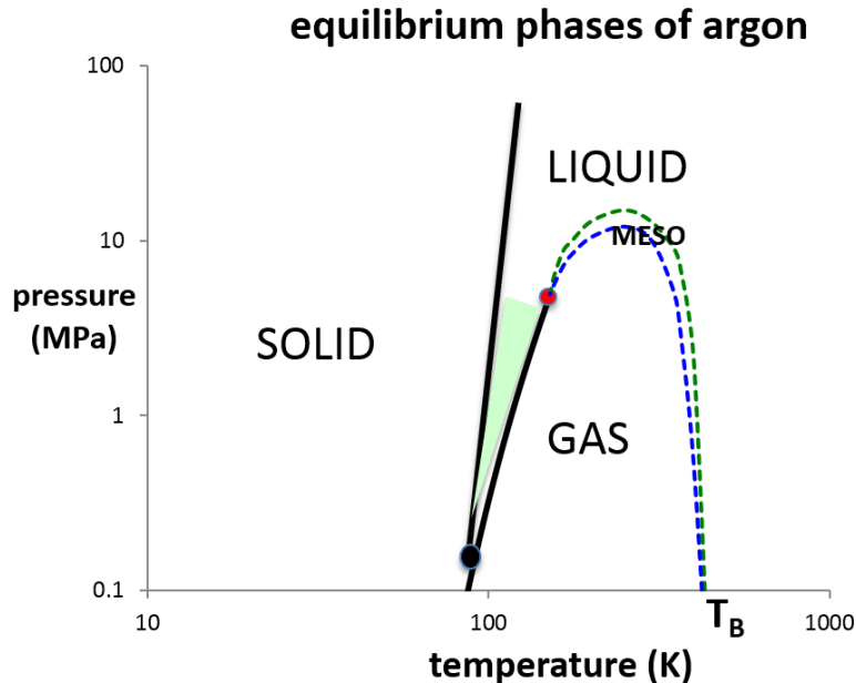
Fig. 12. Postulated p - T phase diagram for fluid argon showing the supercritical mesophase: the blue and green dashed lines are the gas and liquid supercritical state bounds; the red circle is the critical point black circle triple point; the tiny light green shaded area is generally referred to as liquid “state” but the liquid “phase” appears to extend to high temperatures and to exist above the critical temperature, and at all pressures above the Boyle temperature ( T_B )
