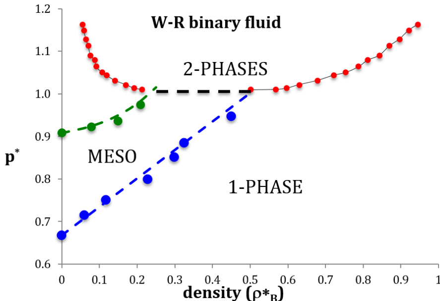
Fig. 6. Phase diagram of the W-R binary fluid in the pressure-density projection: p_{PE}^* (blue) and p_{PA}^* (green) are the percolation transition pressure data points from MD simulations showing the ideal gas percolation pressures at \rho_B^* = 0 ; two-phase coexistence pressure points are red circles; the dashed black line is the critical divide
