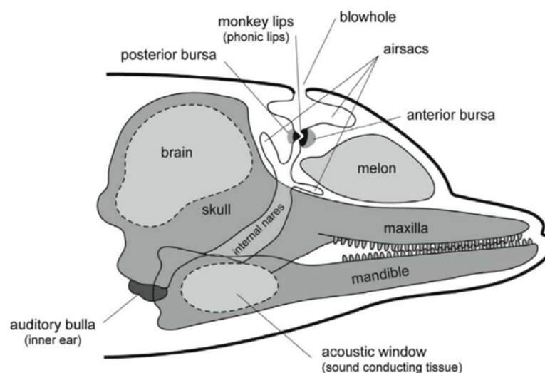
Figure 1.3. Illustration of a dolphin head showing the position of the melon and associated sound-producing structure. (Modified and adapted from Cranford et al. 1996).
