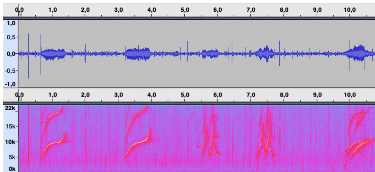
Figure 1.4. Spectrogram (below) and waveform (above) of common bottlenose dolphin ( Tursiops truncatus ) whistles recorded by Bottlenose Dolphin Research Institute.
