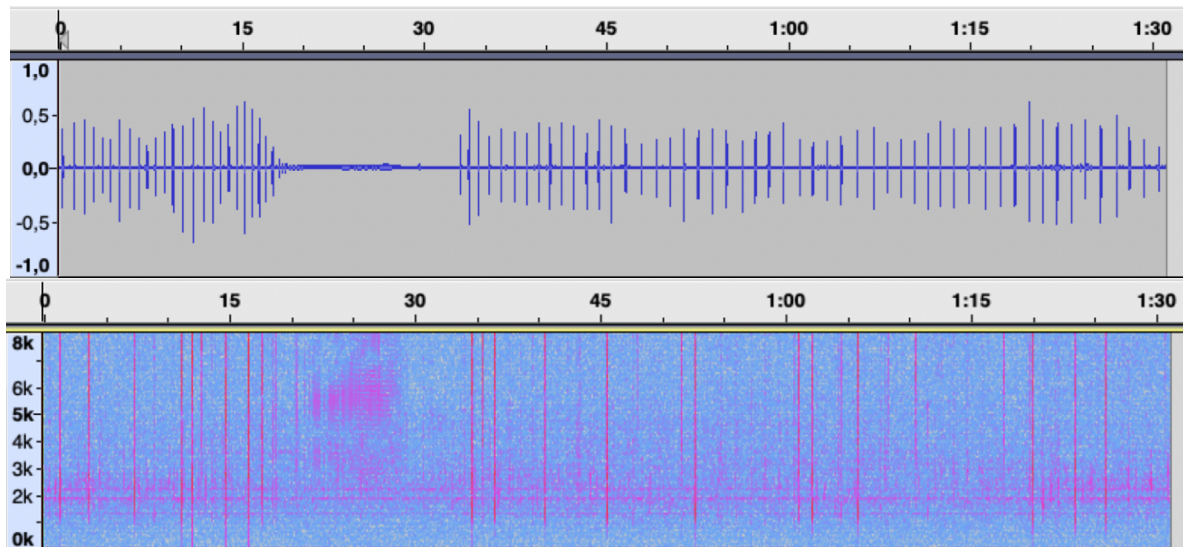
Figure 1.5. Spectrogram (below) and waveform (above) of sperm whale ( Physeter macrocephalus ) clicks recorded by Bottlenose Dolphin Research Institute.
