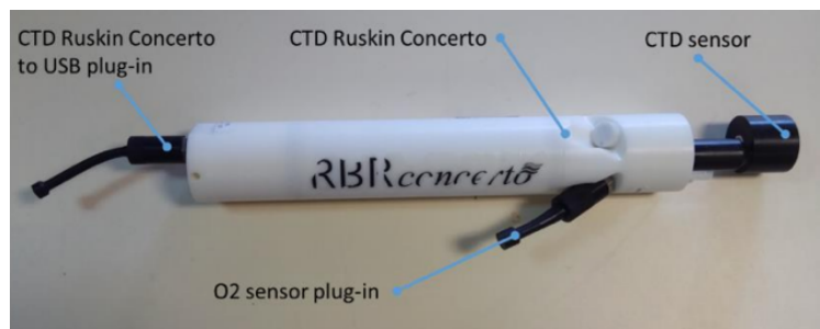
Figure 3.3 CTD Ruskin Concerto part description.
