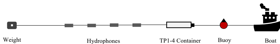
Figure 4.1 Deployment scheme.
