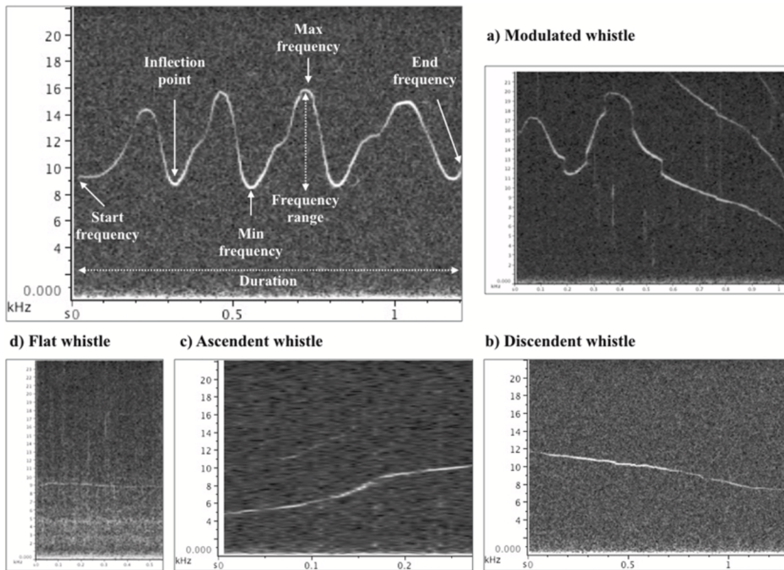
Figure 1.6. Whistle parameters measured from the contour and whistle type. Spectrogram extracted from Raven Pro 1.4 software (1024 point fast Fourier transform (FFT) and 512 window size, Hamming window, 50 % overlap). (from Rako-Gospić et al. 2021)
