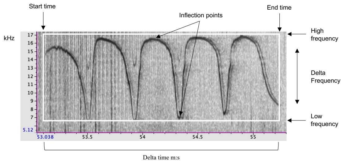
Figure 2.2. Spectrogram of a bottlenose dolphin's whistle recorded in Algarve (Portugal) indicating the seven variables analyzed. Fast Fourier transform (FFT)= 1024, frame duration = 2 ms.
