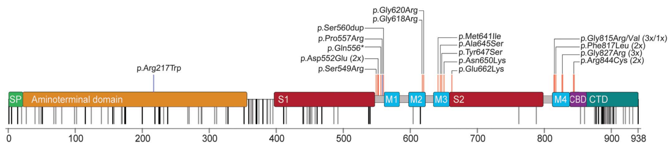
Figure 1 Domains of GRIN1 and distribution of variants
