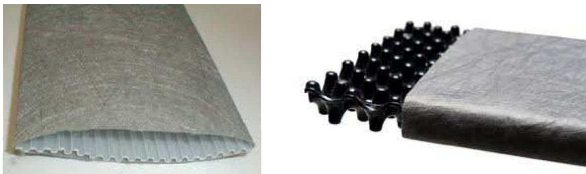
Fig.15 – Diversas formas do núcleo central constituente de um PVD (imagens retiradas em Outubro de 2014) de: http://www.geoengineer.org/education/web-based-class-projects/select-topics-in-ground-improvement/prefabricated-vertical-drains , à esquerda http://www.verticalwickdrain.com/Strip+Drains+Vertical+Wick+Drain+17707.html , à direita
