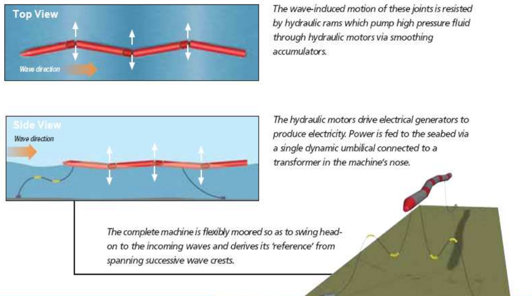
Fig 21. Basic movement made by Pelamis device. (Source: www.pelamiswave.com/ )
