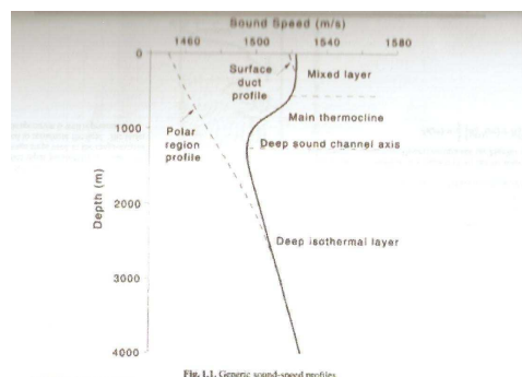
Fig 7. Generic sound speed profile within the ocean water column. (Source: Jensen & Kuperman, 1994)
