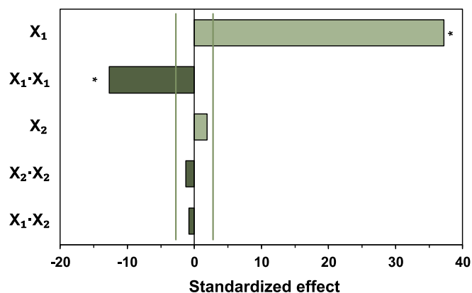
Fig. 4. Pareto chart of the standardized effects obtained from the full factorial design analysis for the \zeta -potential of modified lignins. X_1 : temperature, X_2 : molar ratio. The vertical line represents 95 % of confidence: values above this threshold are statistically significant and are marked with *.
