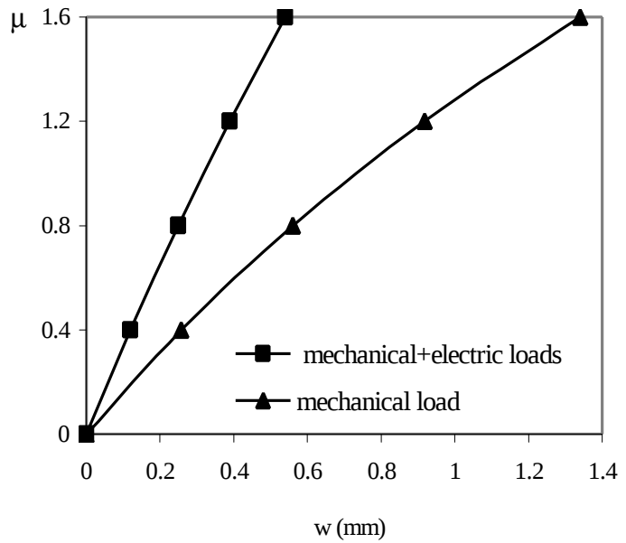
Figure 5. Load-displacement curves.
