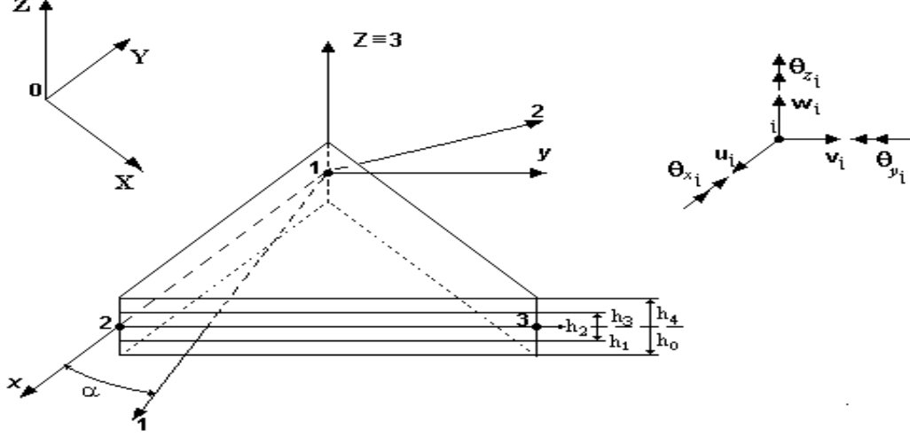
Figure 1. Three node triangular finite element with material (1,2,3) and geometric (x,y,z) coordinate
