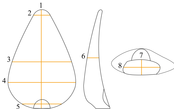
Figure 4.1: Registered measurements scheme fordebitage products and cores. Legend: 1- Maximum length; 2- Distal width; 3- Mesial width; 4- Maximum width; 5- Proximal width; 6- Mesial thickness; 7- Platform thickness; 8- Platform width.
