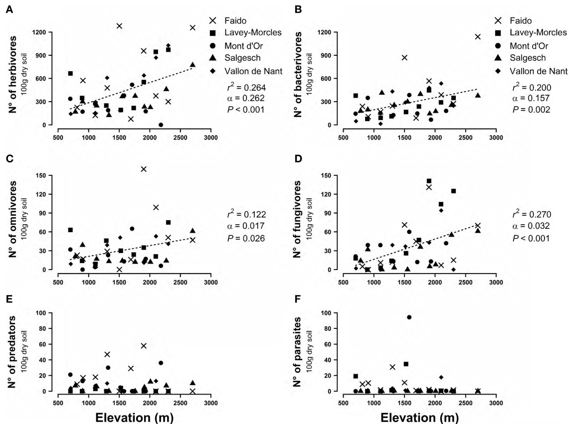
FIGURE 2 | Effect of elevation on the abundance of nematode's trophic group, (A) herbivores, (B) bacterivores, (C) omnivores, (D) fungivores, (E) predators, (F) parasites (i.e., entomopathogenic nematodes). Shown are the sampling sites belonging to five mountain transects as shown in Figure S1. When the mixed linear model is significant, the dashed lines represent the predictions of the models. r^2 , coefficient of determination; \alpha , regression slope; P , significance of the regression slope.
