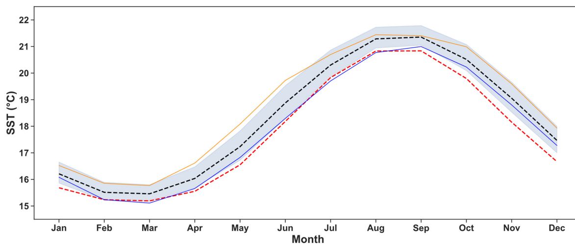
Figure 5. Time series analysis for the entire regional domain. The shaded region represents the 95% confidence interval of the monthly means for each year from 1982 to 2021. The monthly mean baseline from 1982 to 2012 is shown in black and the monthly mean baseline from 1951 to 1981 is shown in red. The year with the maximum SST from the 1982–2021 period (2017) is shown in orange and minimum SST (1986) is shown in blue.
