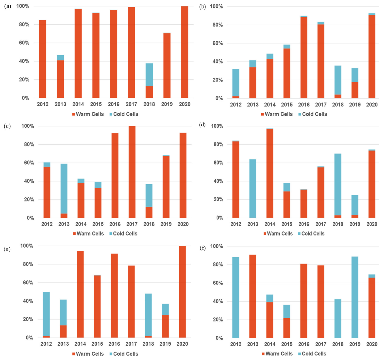
Figure 8. Warming cooling cell percentages for (a) Canary offshore, (b) Canary nearshore, (c) West Iberia offshore, (d) West Iberia nearshore, (e) SW Iberia offshore, and (f) SW Iberia nearshore. Red cells are those with an SST ( ^{\circ}\text{C} ) anomaly higher than the standard deviation relative to the 1982–2012 baseline. Blue cells are those with an SST ( ^{\circ}\text{C} ) anomaly lower than the standard deviation relative to the 1982–2012 baseline.
