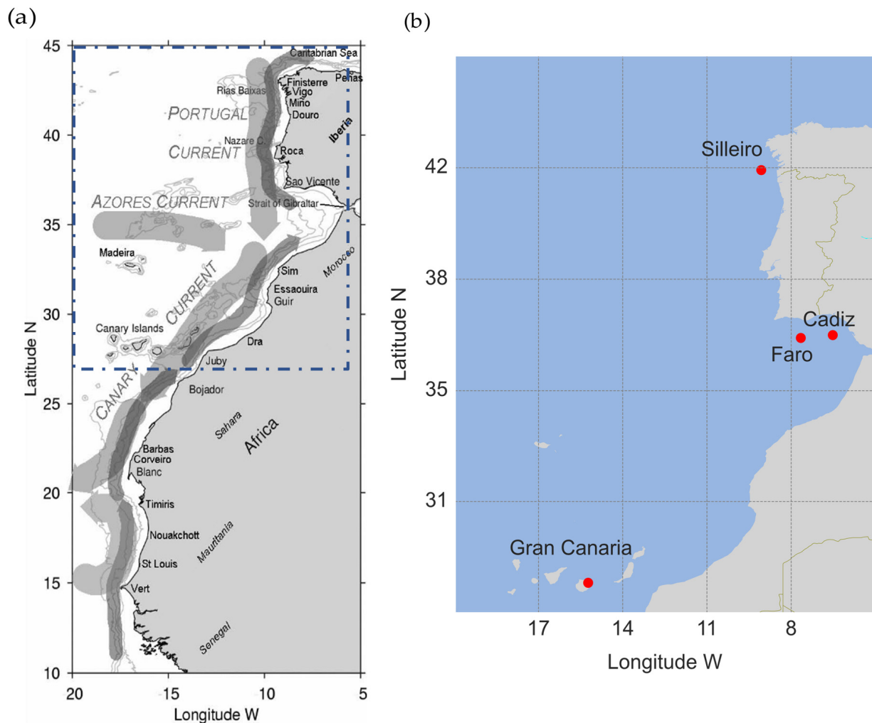
Figure 1. (a) Map of the study area outlining the Eastward North Atlantic Iberian and NW African margin. The 200, 1000, 2000 and 3000 m isobaths are shown. A schematic summer current regime is shown with broad lightly shaded arrows representing surface flows and narrow darkly shaded arrows representing the poleward slope undercurrent. Adapted from [17]. (b) Time series locations to compare results from the 4 mooring buoy stations with the corresponding locations of the satellite product.
