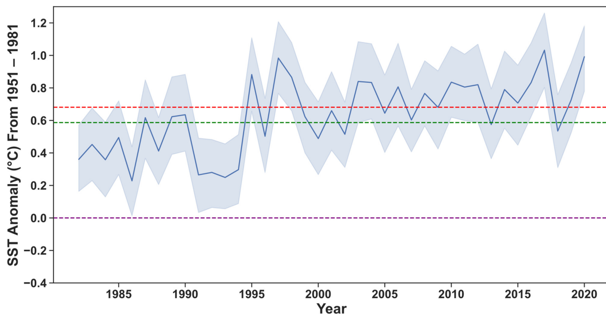
Figure 9. SST anomaly yearly times series from the baseline period 1951–1981. The purple dashed line represents the 1951–1981 baseline period. The blue line is equivalent to the SST of each year subtracted by the 1951–1981 baseline. The shaded regions represent the 95% confidence interval for each yearly SST anomaly. The 1982–2012 baseline at 0.59 °C is shown in green and represents the difference in average SST between 1951–1981 and 1982–2012. The 1991–2020 baseline at 0.68 °C is shown in red and represents the difference in average SST between 1951–1981 and 1991–2020.
