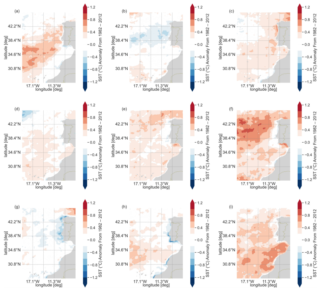
Figure 6. Anomaly maps representing the differences in SST (°C) between each year and the 1982–2012 baseline for (a) 2012, (b) 2013, (c) 2014, (d) 2015, (e) 2016, (f) 2017, (g) 2018, (h) 2019 and (i) 2020. Red areas indicate an increase in SST, blue areas indicate a decrease in SST, and white indicate no significant change.
