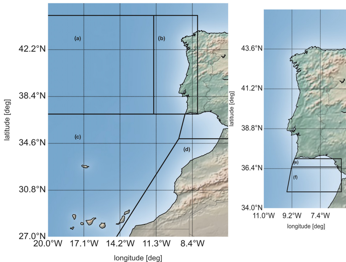
Figure 2. Locations used for the nearshore and offshore analysis: (a) West Iberia offshore, (b) West Iberia nearshore, (c) Canary offshore, (d) Canary nearshore, (e) SW Iberia nearshore, (f) SW Iberia offshore.
