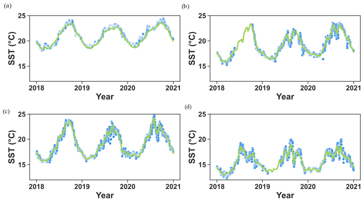
Figure 3. Time series graphs to validate the satellite product (green) with in situ observations (blue) at the following mooring buoy stations (blue): Gran Canaria (a), Faro (b), Gulf of Cadiz (c), Cabo Silleiro (d).
