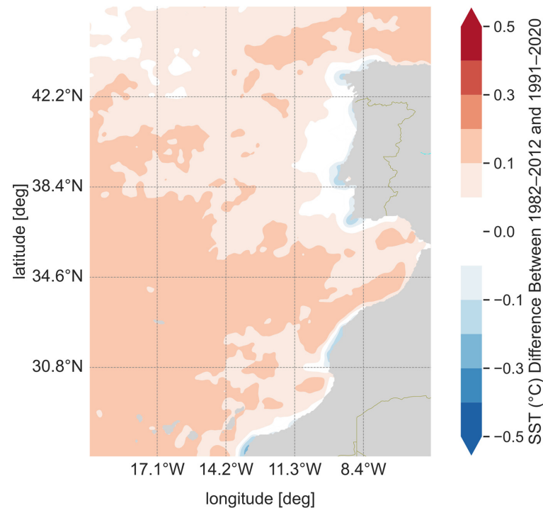
Figure 12. Difference in SST ( ^{\circ}\text{C} ) between the 1982–2012 baseline and the 1991–2020 baseline. Areas in light red indicate increases in SST whereas areas in light blue indicate decreases in SST. The white area represents areas in between \pm\text{STD} ( 0.043^{\circ}\text{C} ) and indicate no significant change.
