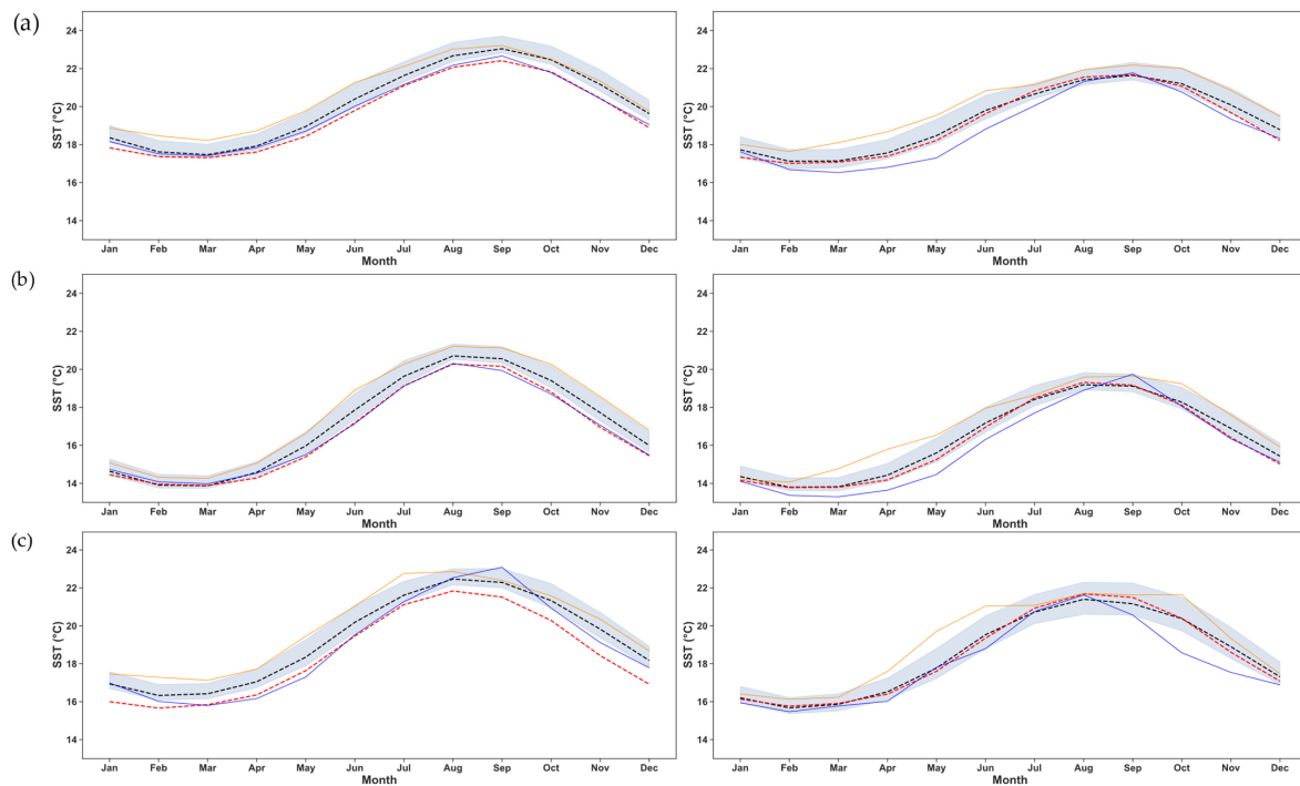
Figure 11. Monthly time series for (a) Canary offshore (left) and Canary nearshore (right), (b) West Iberia offshore (left) and West Iberia nearshore (right), (c) SW Iberia offshore (left) and SW Iberia nearshore (right). The 1982–2012 SST ( ^{\circ}\text{C} ) mean is shown in black and 1951–1981 mean is shown in red. The shaded region represents the 95% confidence of the monthly means for each year for the 1982–2021 dataset. The year with the highest SST ( ^{\circ}\text{C} ) is highlighted in orange and the year with the lowest SST is highlighted in blue.
