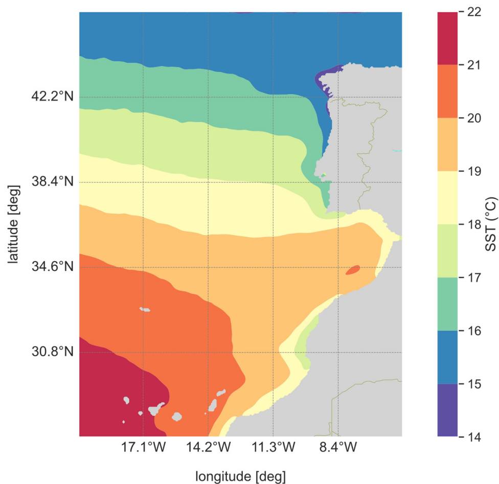
Figure 4. Spatial distribution for the climatological normal in mean SST for the baseline period 1982–2012.
