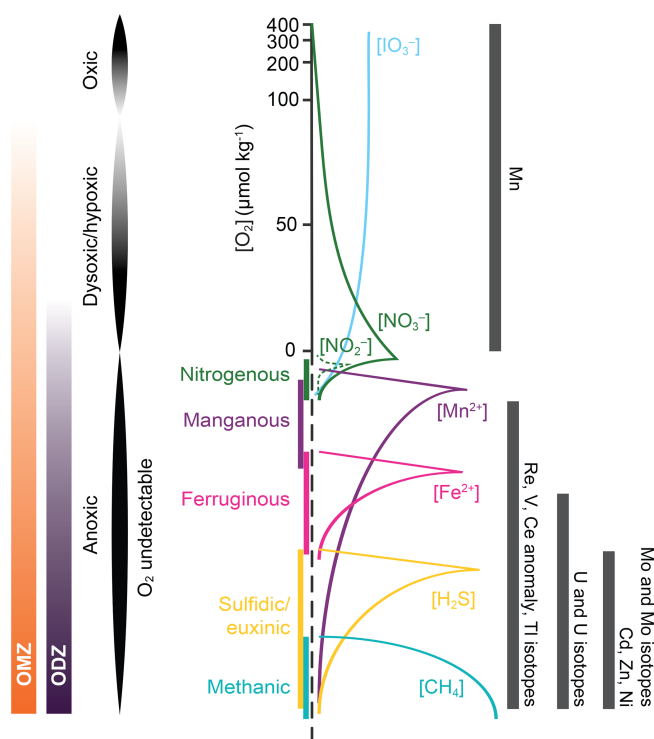
Figure 3. Redox ladder (modified from Fig. 1 in the Introduction) and redox-sensitive trace metals and metal isotopes discussed in this section. Dissolved oxygen ranges for OMZs, ODZs, anoxia, and dysoxia/hypoxia (low oxygen) are labelled in the figure. The redox ladder is modified from Canfield and Thamdrup (2009). The oxygen/redox potential range for the use of each redox-sensitive metal and metal isotope redox proxy is shown with the bars on the right.
