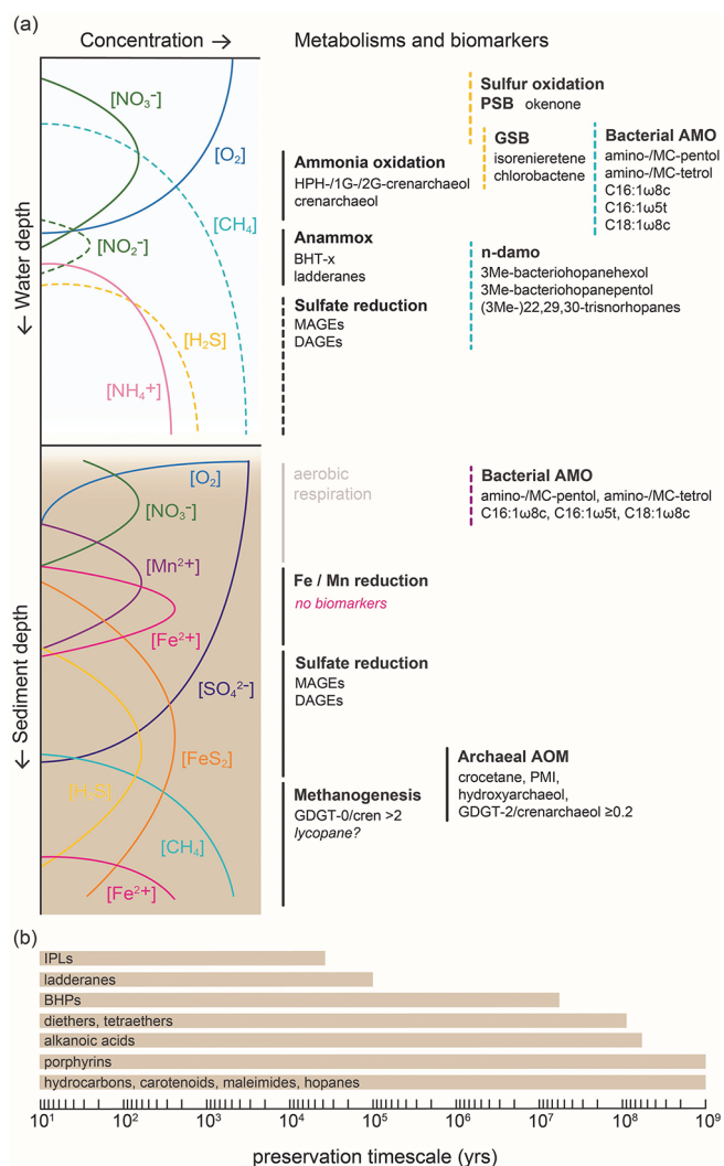
Figure 6. (a) Idealized water column and sediment redox zonation and associated metabolisms and their biomarker signatures discussed in the text. The dashed lines indicate species and metabolisms that may be present in specific settings. (b) Biomarker preservation timescale. The solid lines indicate timescales on which distinct compound classes are preserved. Note that observations are less frequent where the scale extends to the oldest known record.
