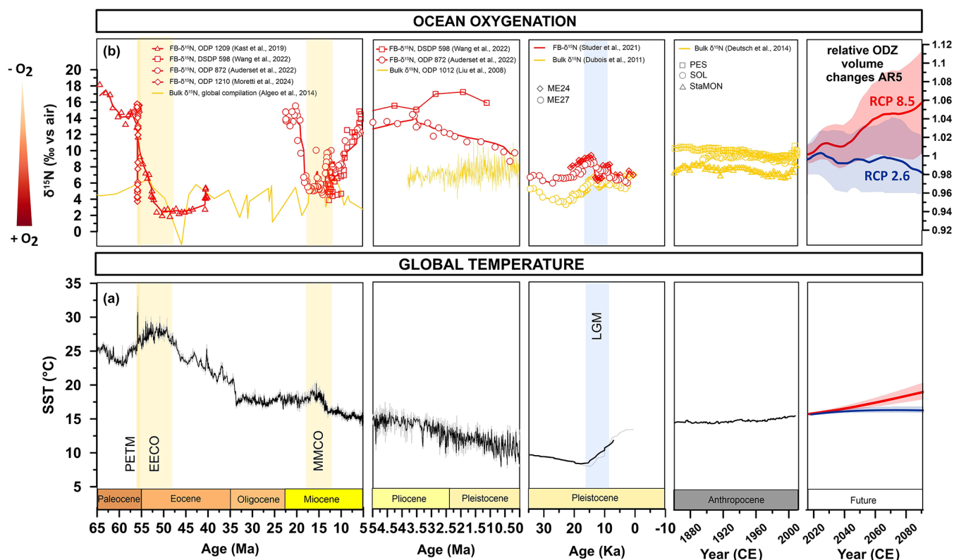
Figure 7. Compilation of proxy reconstructions of equatorial Pacific anoxia from (FB)- \delta^{15}\text{N} . From left to right: the time spans 65–5 Myr, 5–0 Myr, 35–0 kyr, and 1860–2010 CE and the simulated global ODZ volume for RCP2.6 and RCP8.5 projections for 2020–2100 from IPCC AR5 (Bindoff et al., 2019). (a) Sea surface temperature compilation by Hansen et al. (2013). (b) Analyses of \delta^{15}\text{N} in bulk sediment (yellow) and foraminifera-bound (FB) organics (pink) in Pacific sedimentary archives. \delta^{15}\text{N} is used as a qualitative oxygen-sensitive proxy due to the strong isotopic fractions of denitrification by ODZ-dwelling bacteria. Data were compiled from the following sources: ODP 1209 (Kast et al., 2019); DSDP 598 (Wang et al., 2022b); ODP 872 (Auderset et al., 2022); ODP 1012 (Liu et al., 2008); ME24 and ME27 (Studer et al., 2021; Dubois et al., 2011); PES, SOL, and StaMON (Deutsch et al., 2014); the global Paleocene–Miocene compilation from Algeo et al. (2014); and the Paleocene–Eocene Thermal Maximum (PETM; Moretti et al., 2024).
