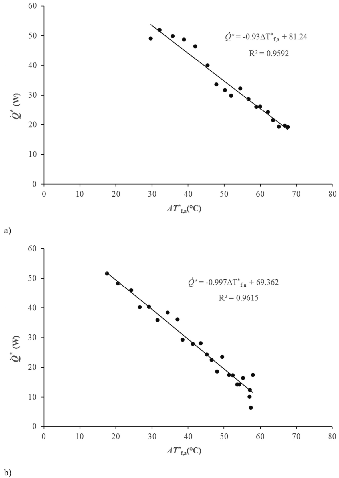
Fig. 9. Coking power curve as a function of temperature difference for the tests performed with water: a) on 13/6/2022 with glass enclosure and b) on 17/7/2023 pro1 with plastic bag.
