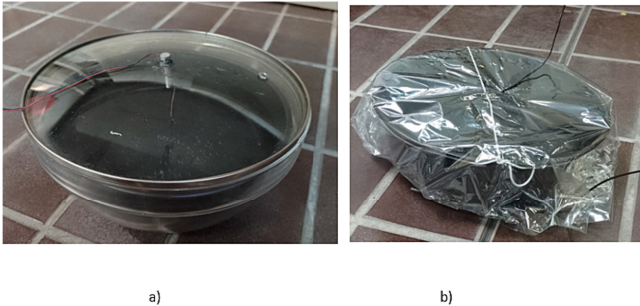
Fig. 4. Cooking pot with: a) a glass enclosure and b) a plastic enclosure.
