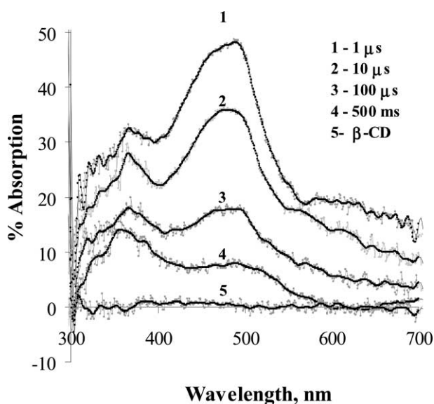
Fig. 5 Time-resolved absorption spectra for a benzil/β-cyclodextrin sample with a 1 : 1 guest : host molar ratio. ( \lambda_{\text{exc}} = 355 nm).
