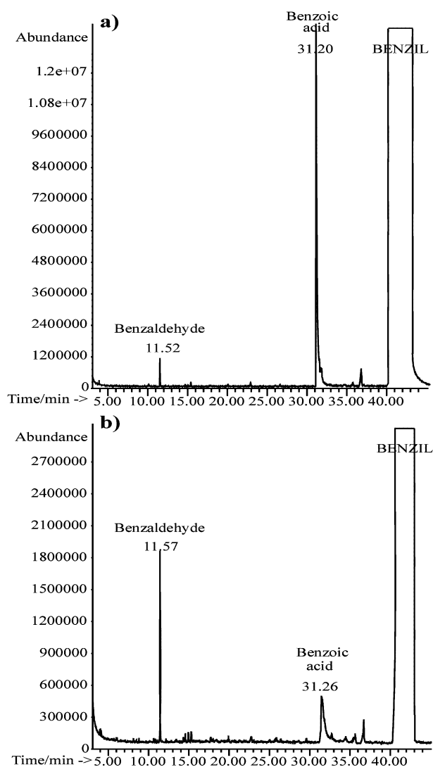
Fig. 6 GC-MS chromatograms of the acetonitrile extract from an 'unwashed' laser-irradiated sample of benzil/cellulose: (a) air-equilibrated; (b) argon-purged.
