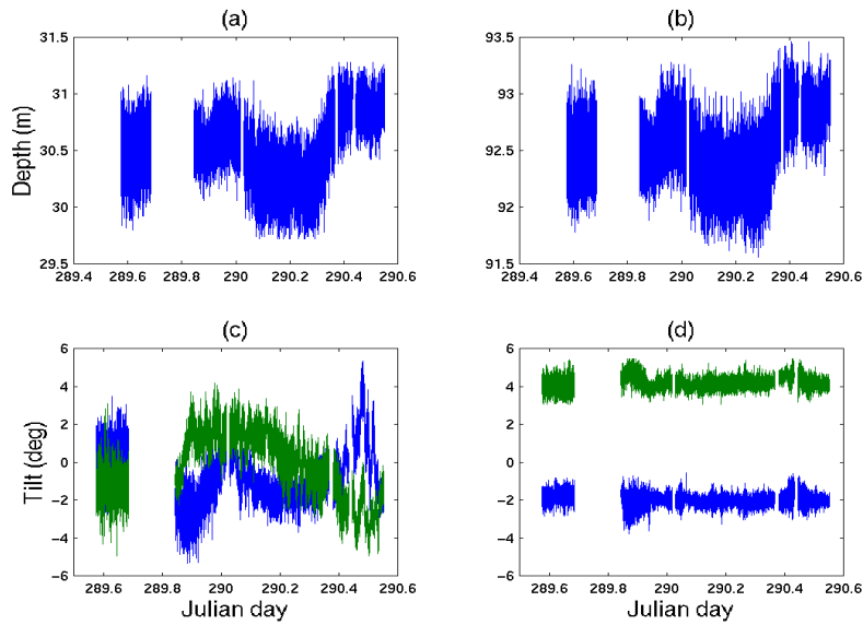
Figure 4.9: Event 2: receiving array depth (a)-(b) and tilt (c)-(d).
