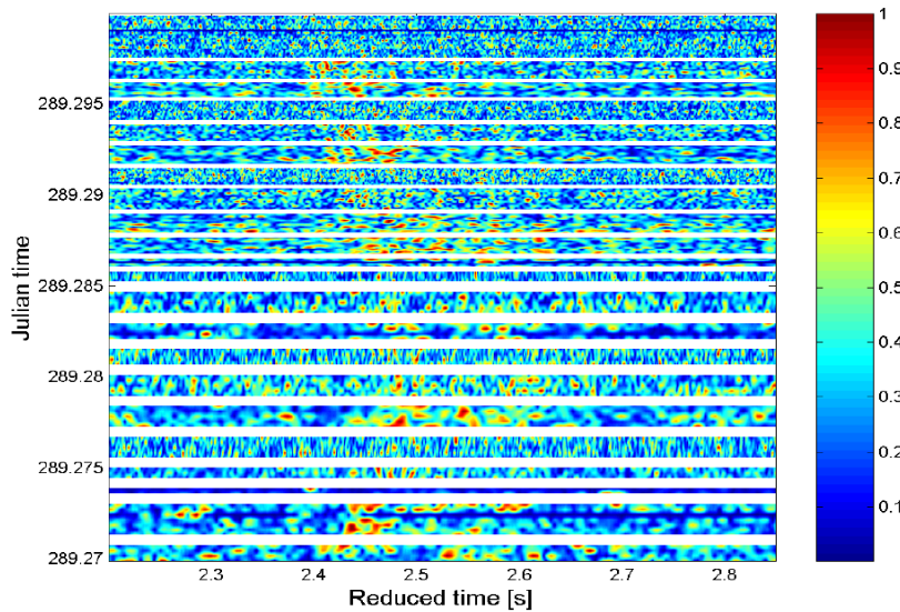
Figure 5.16: Pulse compressed received probe signal for hydrophone 1 and all codes during station 3.
