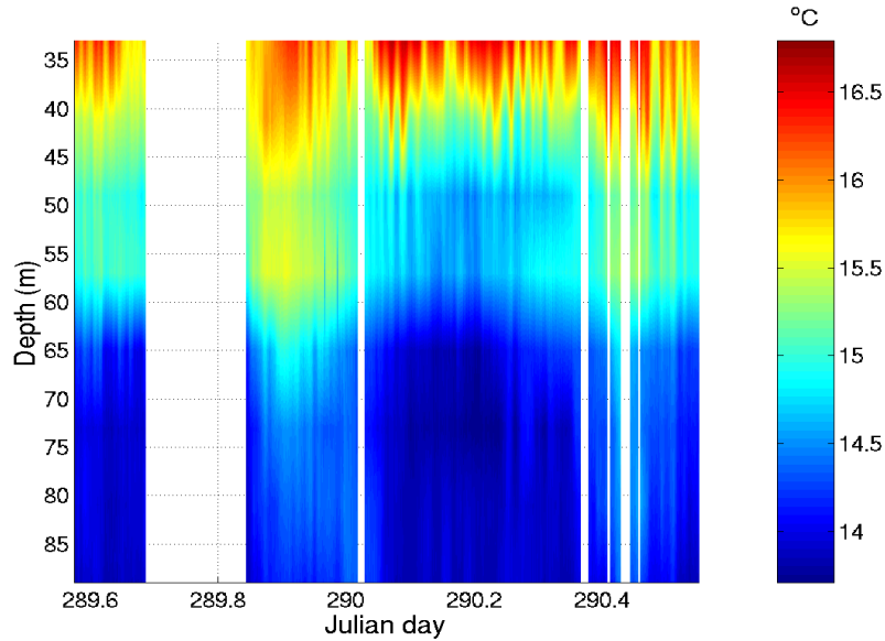
Figure 3.6: Temperature field recorded at the VLA during Event 2.
