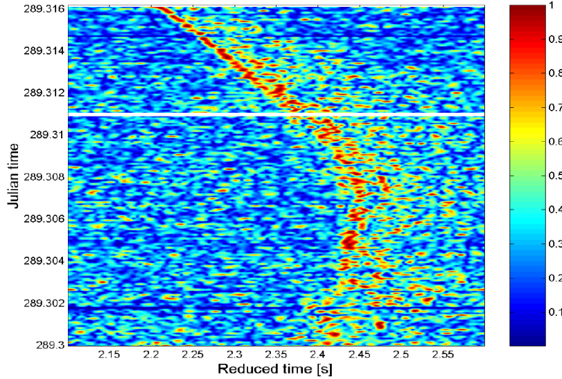
Figure 5.17: Pulse compressed received probe signal for hydrophone 1 and all codes during part of the course between station 3 and station 4.
