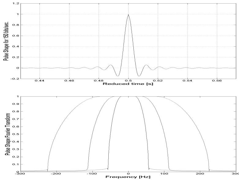
Figure 5.1: Root-root raised cosine pulse shape (a) and its spectrum for 75, 150 and 300 symbols/s(b).
