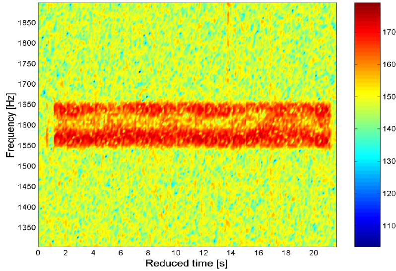
Figure 5.6: Time-frequency plot of received code N20PSK275, at hydrophone 1 during Event 1.
