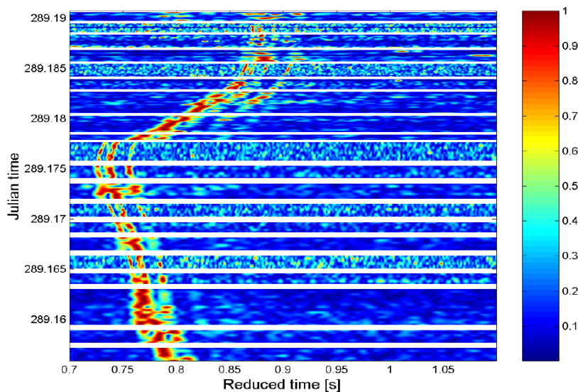
Figure 5.11: Pulse compressed received probe signal for hydrophone 1 and all codes during station 1.
