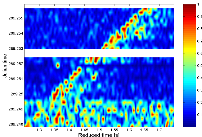
Figure 5.14: Pulse compressed received probe signal for hydrophone 1 and all codes during part of the course between station 2 and station 3.
