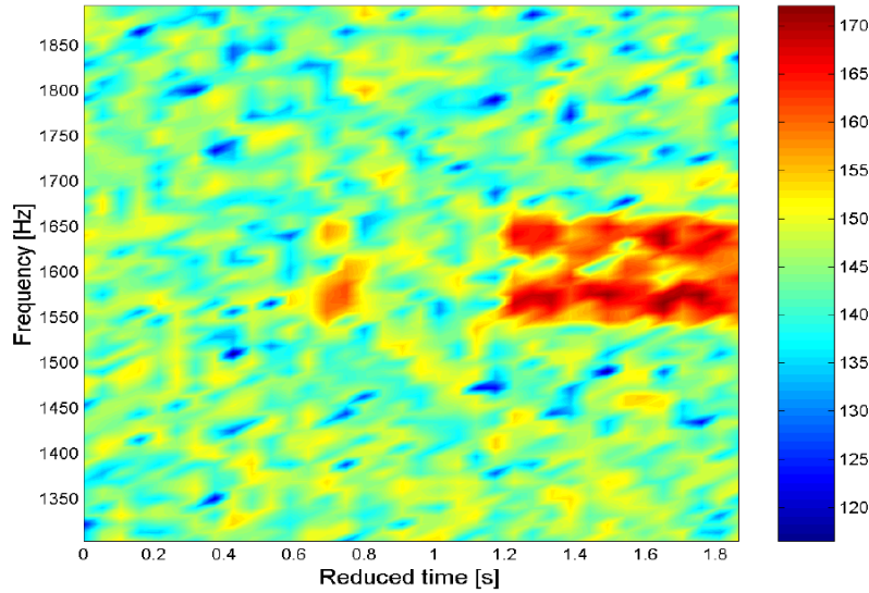
Figure 5.7: Blowup of time-frequency plot of received code N20PSK275, at hydrophone 1 during Event 1: first 2 seconds.
