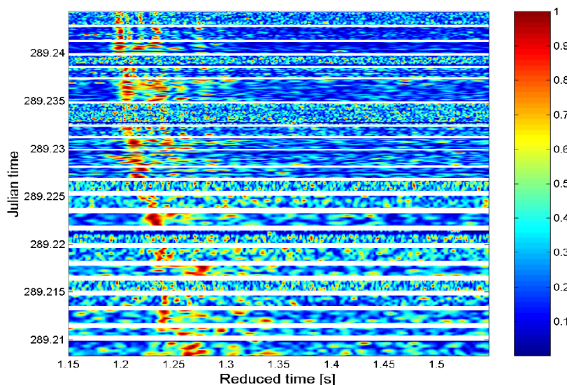
Figure 5.13: Pulse compressed received probe signal for hydrophone 1 and all codes during station 2.
