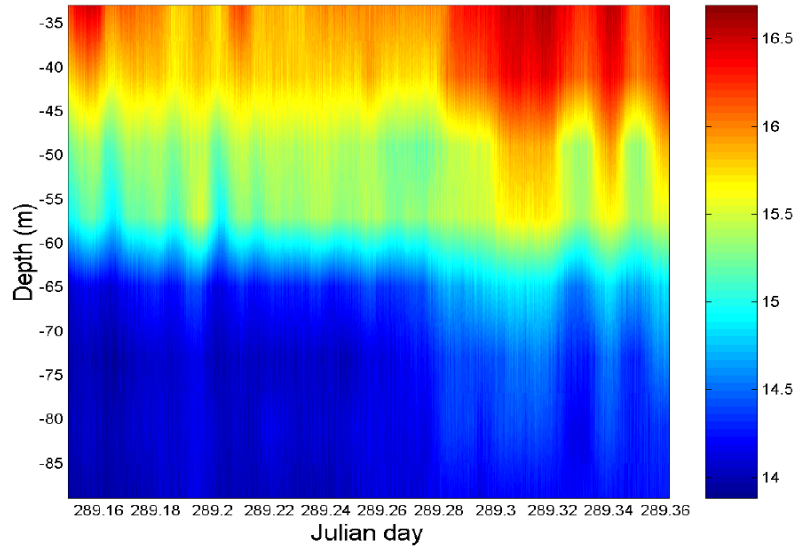
Figure 3.5: Temperature field recorded at the VLA during Event 1.
