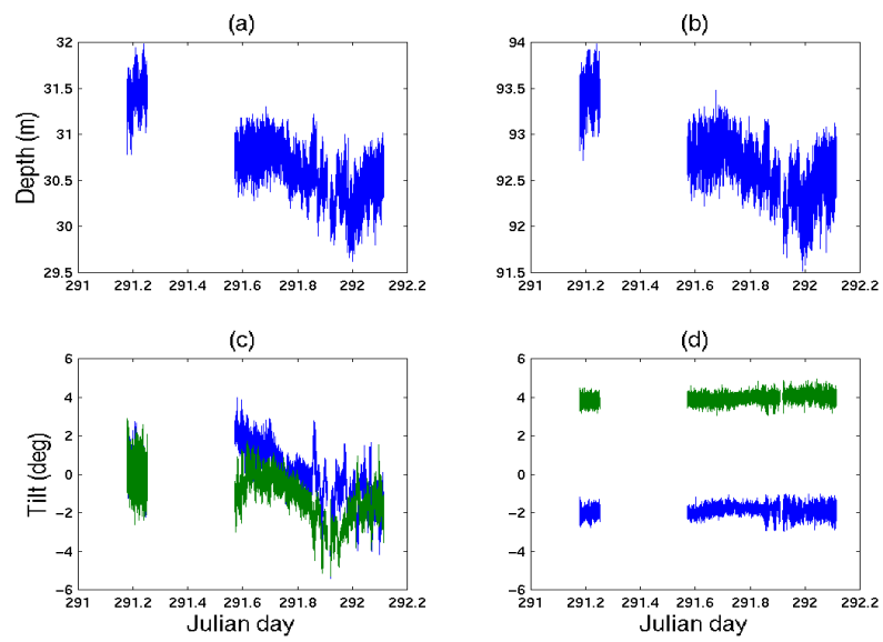
Figure 4.10: Event 3: receiving array depth (a)-(b) and tilt (c)-(d).
