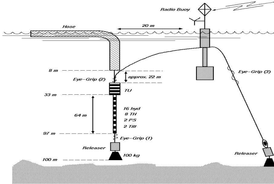
Figure 2.2: Vertical Line Array (VLA) structure.
