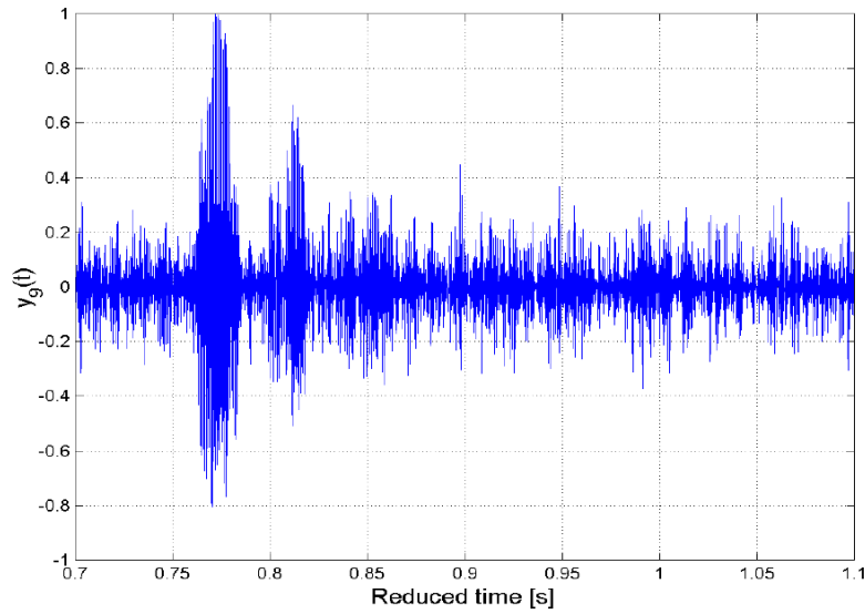
Figure 5.8: Received probe signal on hydrophone 9 for the 75 bits/s data rate.
