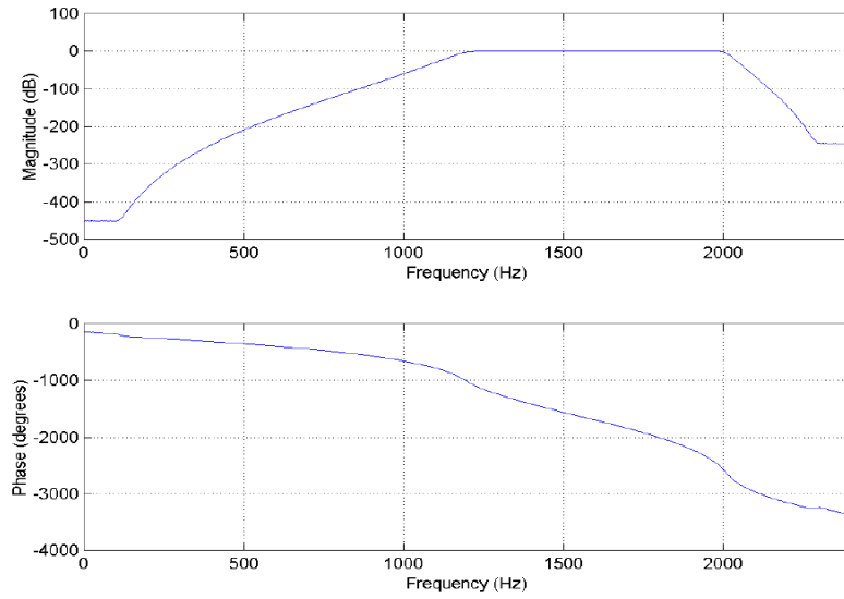
Figure 5.4: Transfer function of bandpass filter used for visualization of received signals during Event 1.
