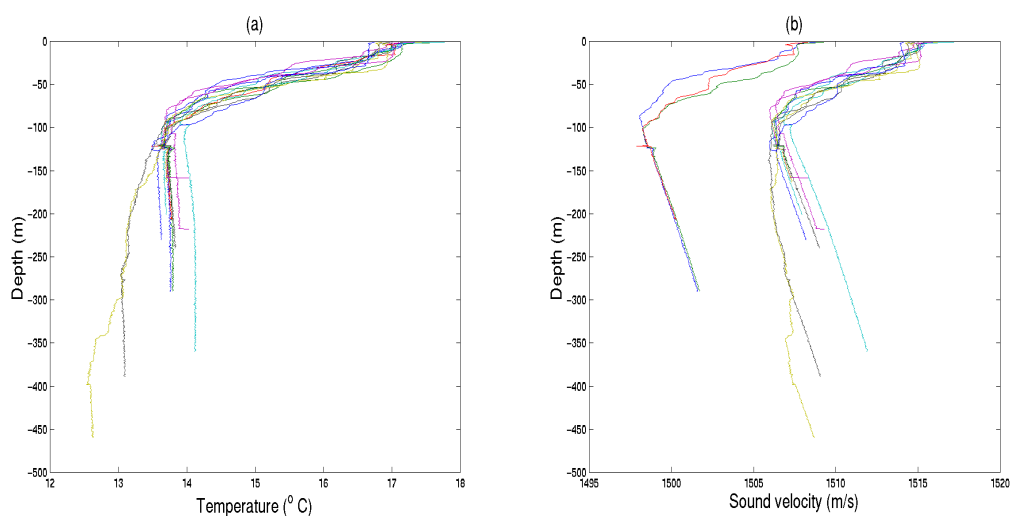
Figure 3.2: XBT data: temperature (a) and calculated sound velocity (b).
