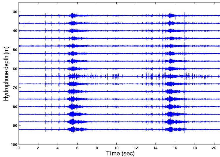
Figure 5.25: Received signals during Event 3.
