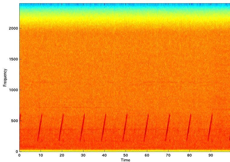
Figure 5.22: Event 2: spectrogram of the signal received on hydrophone 8.
