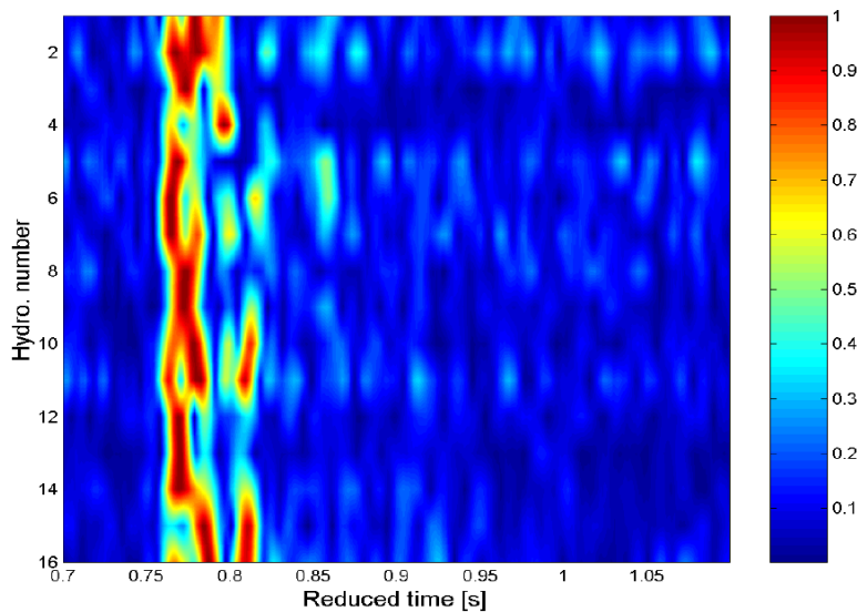
Figure 5.10: Pulse compressed received probe signal for all hydrophones and for the 75 bits/s data rate.
