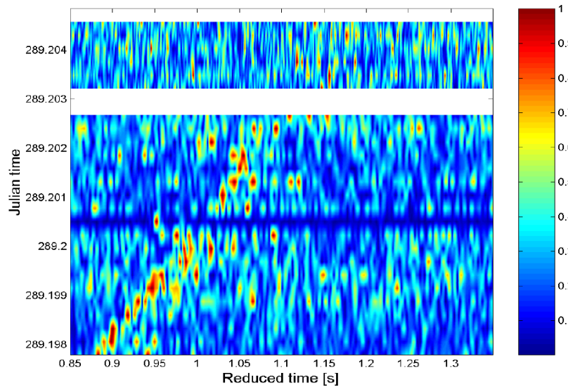
Figure 5.12: Pulse compressed received probe signal for hydrophone 1 and all codes during the course between station 1 and station 2.
