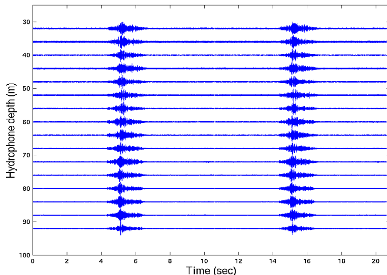
Figure 5.21: Received signals during Event 2 after pre-processing.
