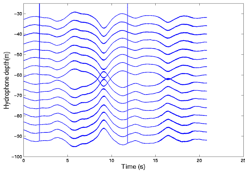
Figure 5.3: Example of phase inversion between top 8 and bottom 8 hydrophones.
