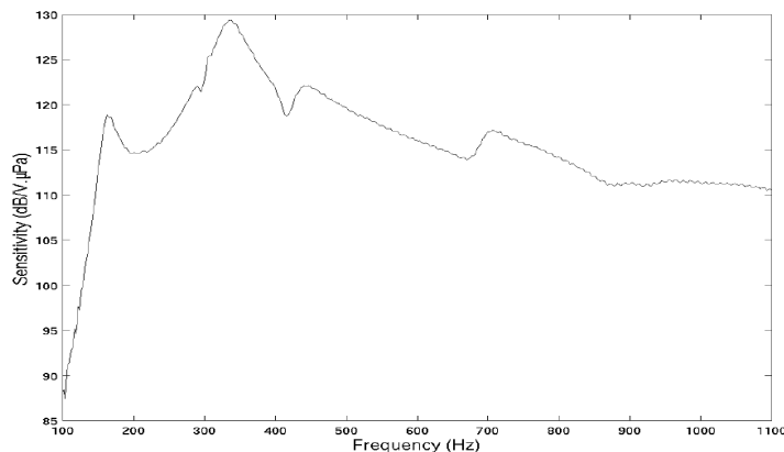
Figure 5.2: HX90 acoustic source sensitivity
