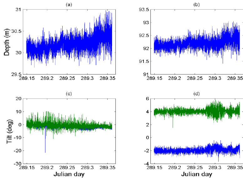
Figure 4.8: Event 1: receiving array depth (a)-(b) and tilt (c)-(d).
