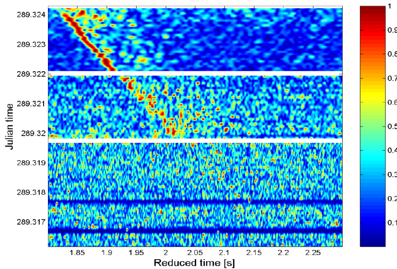
Figure 5.18: Pulse compressed received probe signal for hydrophone 1 and all codes during part of the course between station 3 and station 4.
