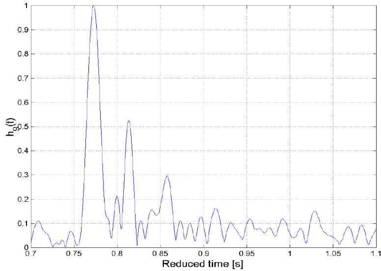
Figure 5.9: Pulse compressed received probe signal on hydrophone 9 for the 75 bits/s data rate.
