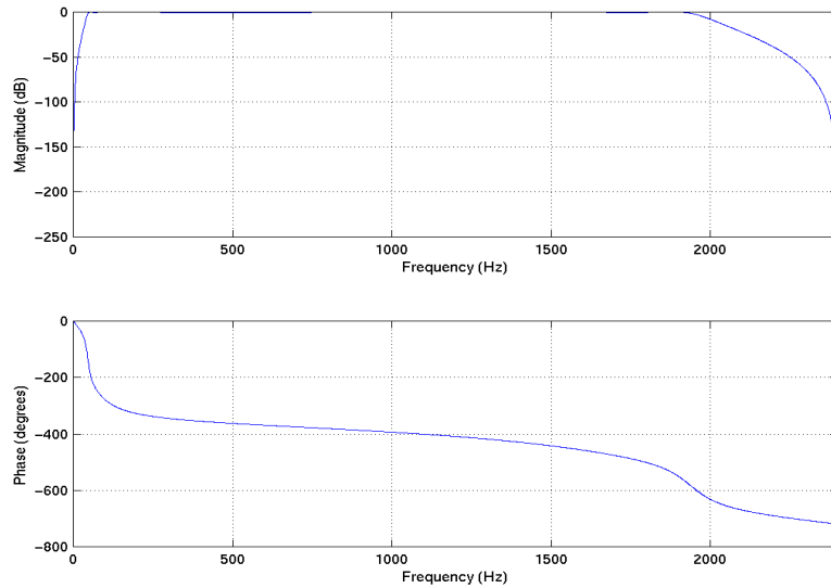
Figure 5.20: Chebychev 4th-order [48,1920] Hz, band-pass filter amplitude frequency response.
