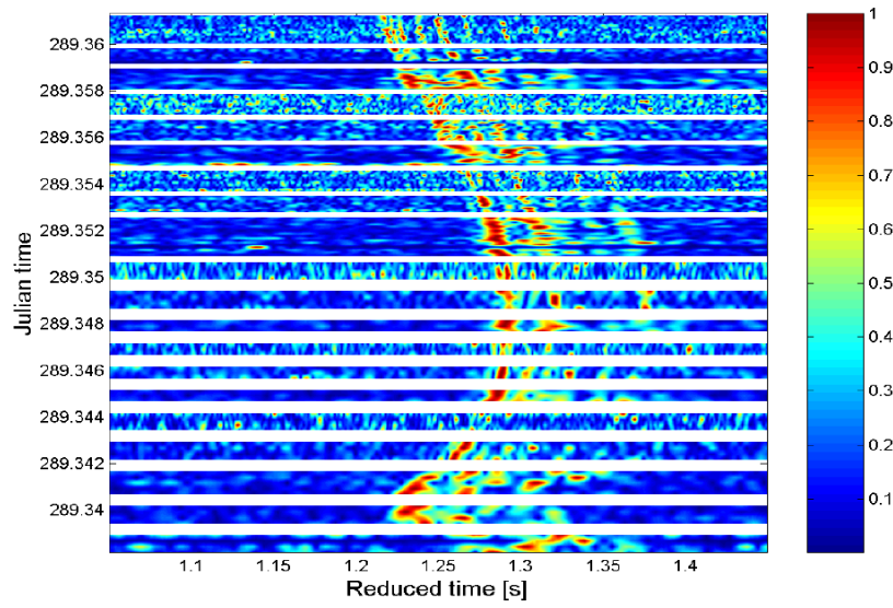
Figure 5.19: Pulse compressed received probe signal for hydrophone 1 and all codes during station 4.
