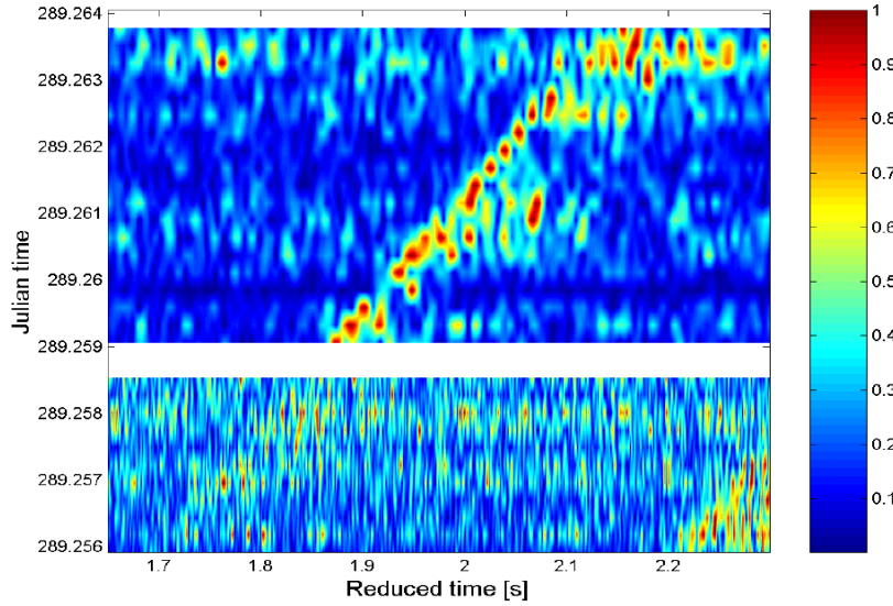
Figure 5.15: Pulse compressed received probe signal for hydrophone 1 and all codes during part of the course between station 2 and station 3.
