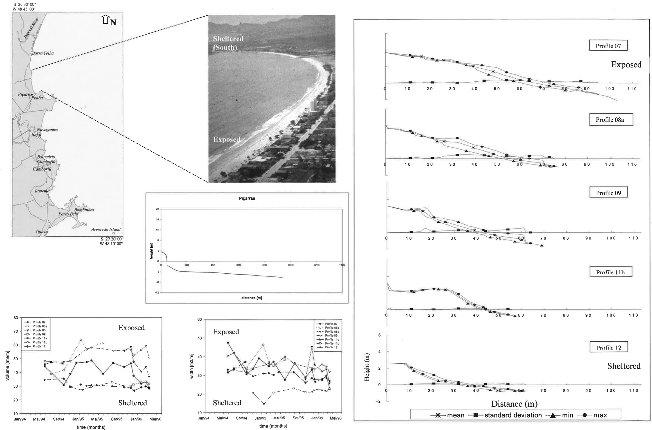
Figure 4.14. Principal beach characteristics observed in a semi-exposed/parabolic beach stage, reflective to dissipative, during the study period (Piçarras beach).
