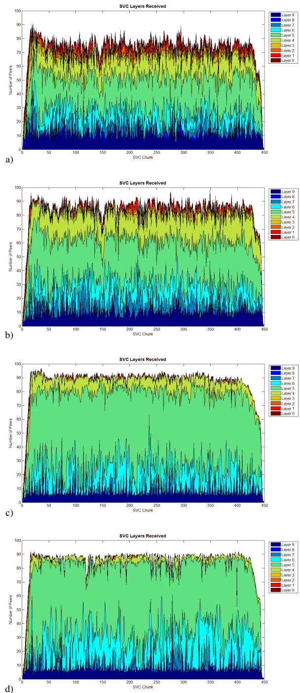
Figure 7. SVC layers received using different sliding window sizes: a) 2 chunks b) 3 chunks c) 4 chunks d) 5 chunks.
