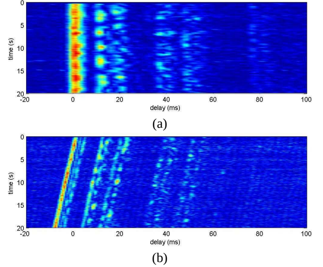
Figure 2: Evolution of estimated channel impulse responses before Doppler compensation (a) PKT 106 (200 baud, f_{dop} = -0.11 Hz) (b) PKT 149 (400 baud, f_{dop} = 1.65 Hz)
