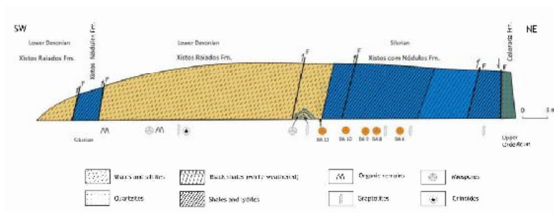
Figure 2. Scheme of the road cut EN 258, Sto Aleixo da Restauração to Barrancos, km 103,7, with location of productive palynostratigraphic samples (adapted from Oliveira, et al. , 2000).
