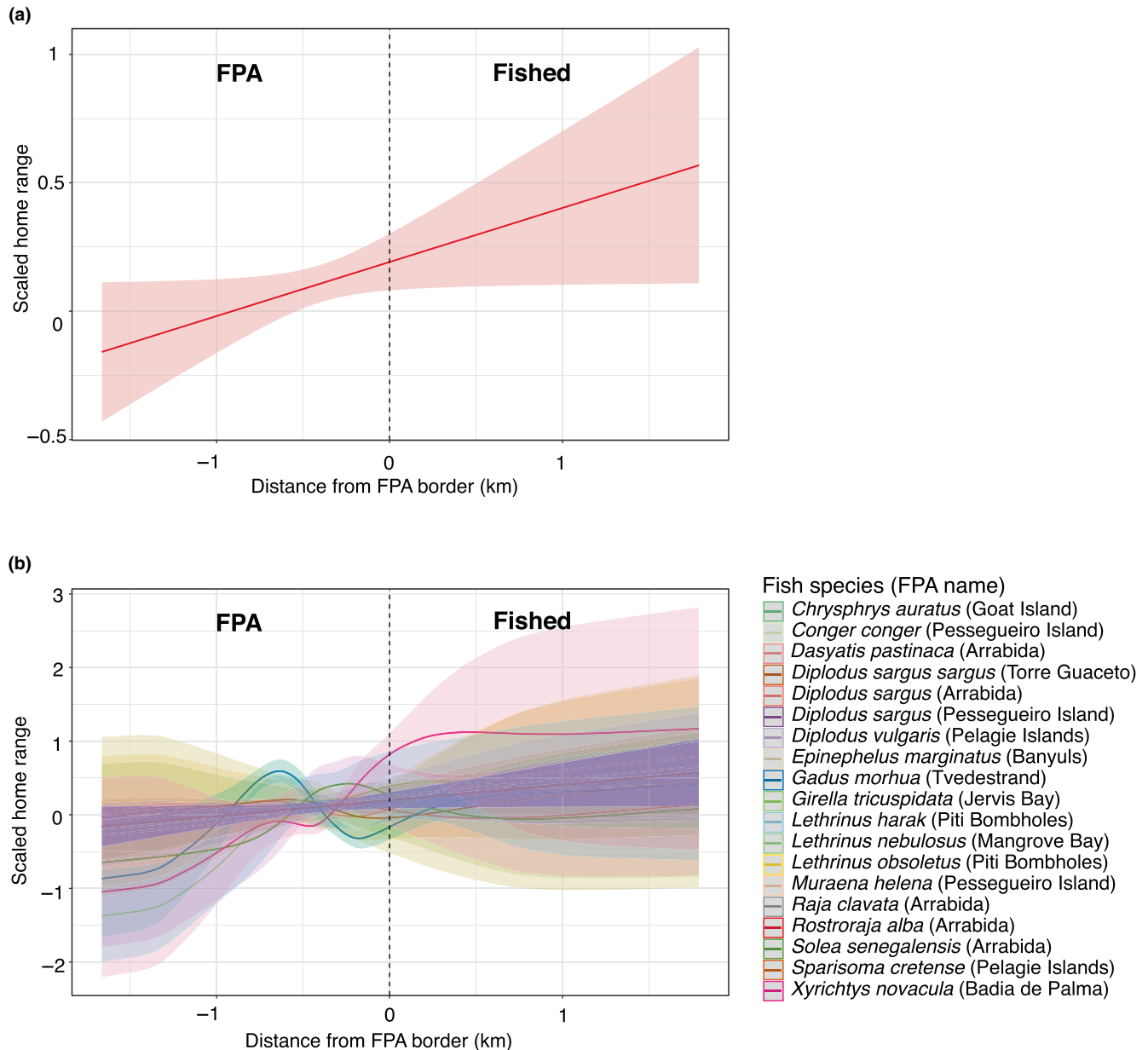
FIGURE 3 The spatial patterns of individual-level home range sizes as a function of distance from the FPAs border. (a) The global effect of distance from the FPA border (x-axis, in km) on home range size (y-axis, home range is standardized). (b) The species-level effect of distance from the FPA border on home range size (each colour represents a different dataset). Both (a) and (b) present the marginal effects of the best-supported GAM model (Table 1). We note that it is difficult to discern the exact shape of the curve for specific species, thus we show the species-level patterns in Figure S2. The dashed vertical lines represent the FPA border. The shaded areas around the model curves denote 95% confidence intervals.
