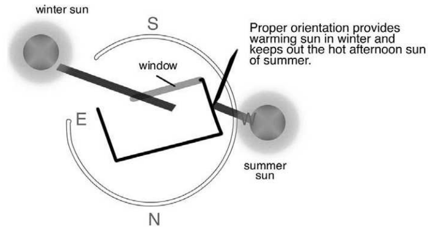
Figure 9.2 Structures designed for the local climate use less energy and provide more comfort to occupants.
