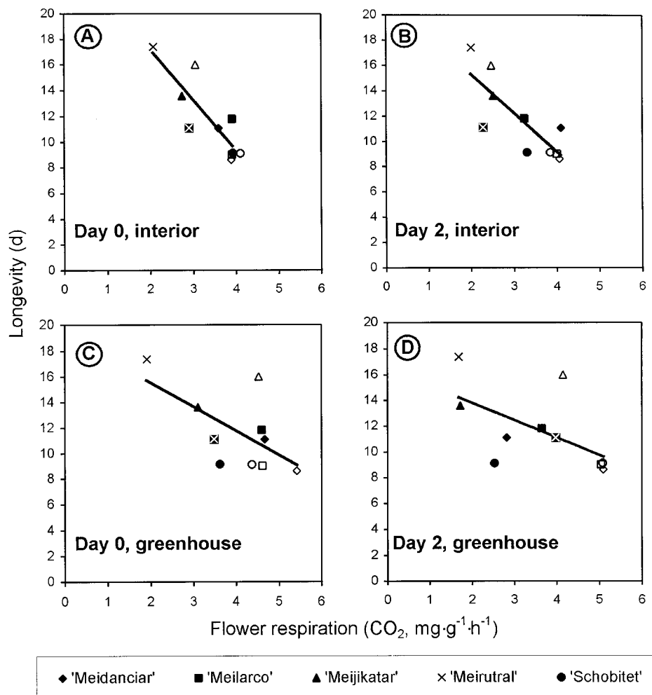
Fig. 2. Spring/summer experiments (Expts. 1 and 2). Correlation of flower longevity under interior conditions with flower respiration at different times and environments: (A) at anthesis under interior conditions: Y = 25.039 - 3.908x , significant at P = 0.0014 ; (B) 2 d after anthesis under interior conditions: Y = 21.39 - 3.039x , significant at P = 0.0051 ; (C) at anthesis in the greenhouse: Y = 19.32 - 1.89x , significant at P = 0.055 ; (D) 2 d after anthesis in the greenhouse: Y = 16.52 - 1.348x , significant at P = 0.0778 . Interior rooms provided 21 ± 1 °C and 50 ± 5% relative humidity with a 12-h photoperiod of 12 μmol·m -2 ·s -1 ( PAR ). Each symbol represents the mean ( n \geq 4 ) of a cultivar for a specific experiment. Solid symbols (as in the legend) are from the June experiment, and open symbols are from the April experiment.
