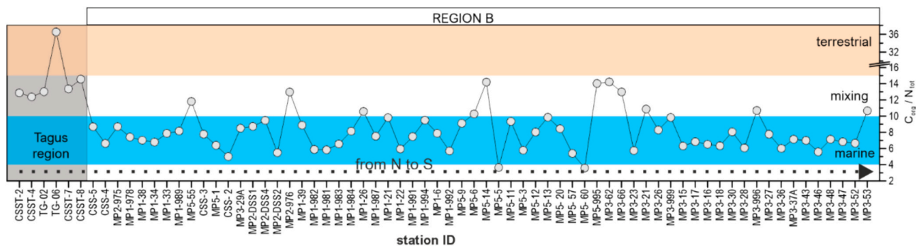
Fig. 9. Spatial variation of C_{org}/N_{tot} in the collected surface sediments. The samples are ordered from North (left) to South (right). The shaded area marks the surface sediment samples collected from the Tagus region. The light brownish and blue shaded bands represent the ranges of C_{org}/N_{tot} values of terrestrial and marine organic matter originated, as indicated in Meyers (1994, 1997). (For interpretation of the references to colour in this figure legend, the reader is referred to the web version of this article.)
