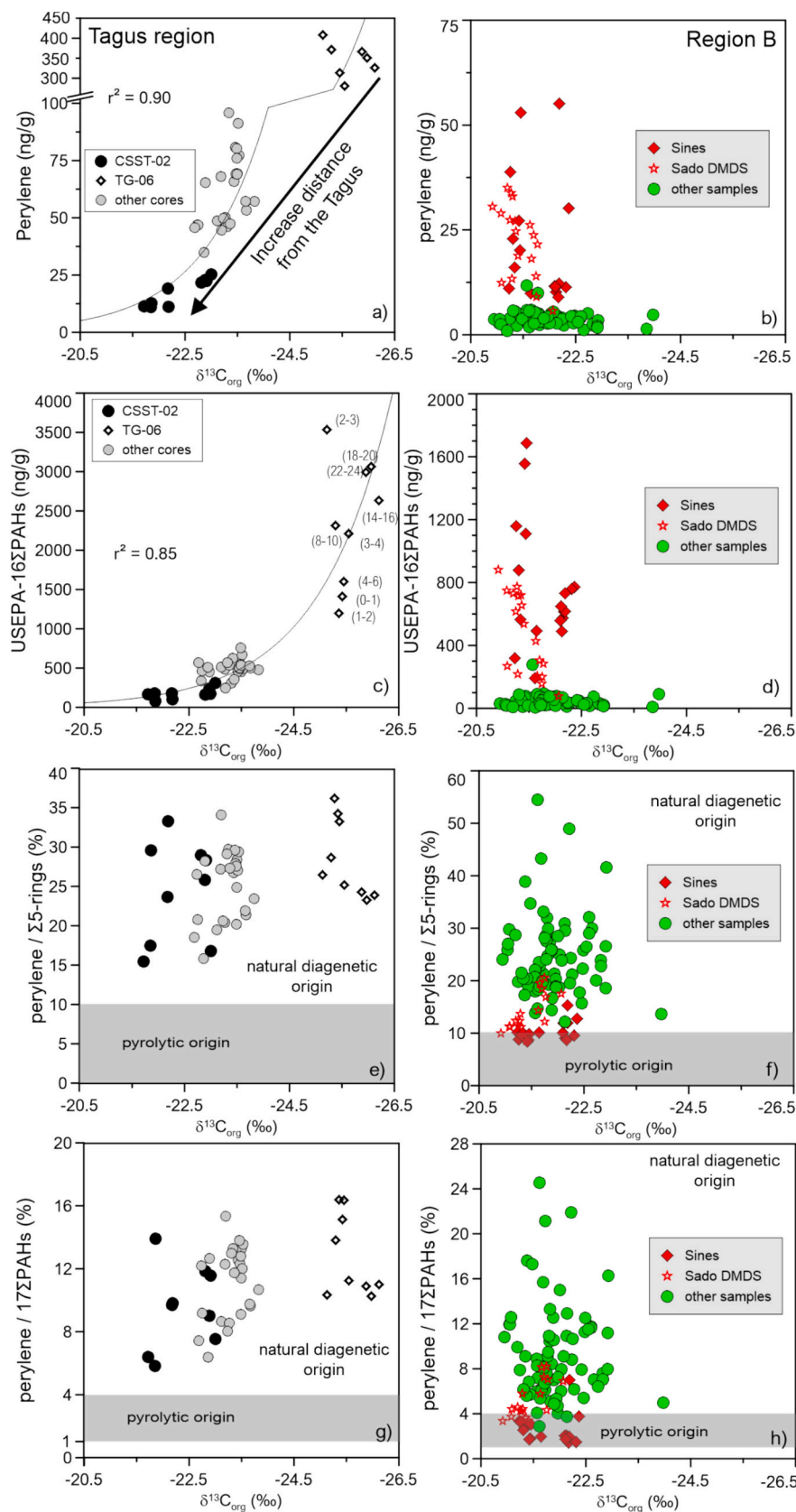
Fig. 15. \delta^{13}\text{C}_{\text{org}} versus perylene, \delta^{13}\text{C}_{\text{org}} versus 16ΣPAHs, \delta^{13}\text{C}_{\text{org}} versus perylene/Σ5-ring PAHs and \delta^{13}\text{C}_{\text{org}} versus perylene/17ΣPAHs in the sediment samples from the Tagus region (a, c, e and g) and Region B (b, d, f and h).
