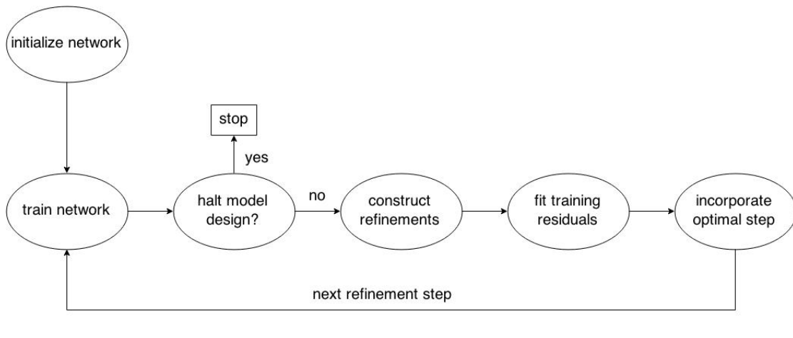
FIGURE 4.6: B-spline network design cycle.
