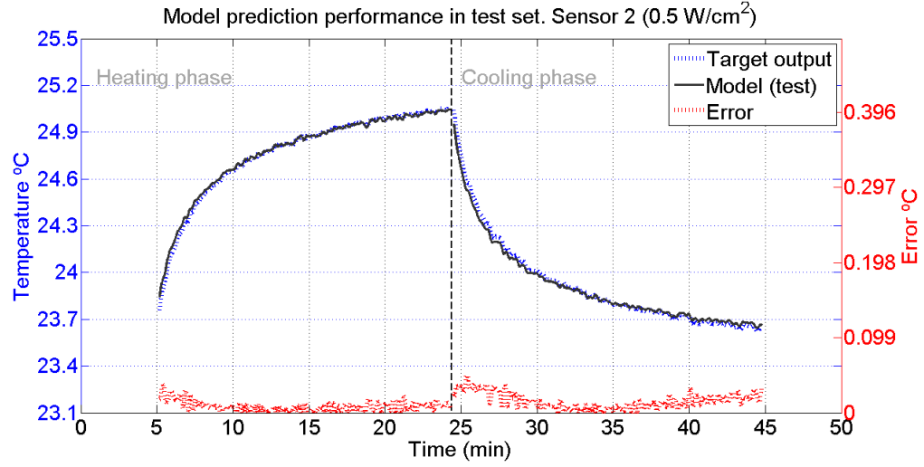
FIGURE D.2: Behaviour of model 4 in the test set (Sensor 2 0.5W/cm^2 ), selected using the KTB approach. The blue line represents the desired behaviour and the model's test output is given by the black line. The error line is red. SIMP, homogeneous phantom experimental setup. Data used: corrupted.
