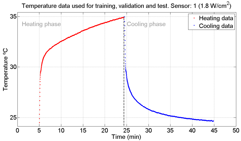
FIGURE C.1: Uncorrupted original data set used for SPSI model training, validation and test. Collected from the homogeneous phantom experimental setup. TUS intensity: 1.8W/cm^2 . Sensor 1.
