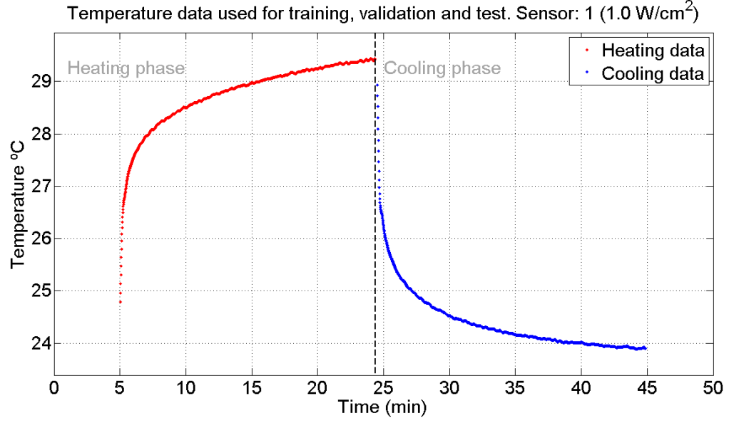
FIGURE 5.1: Unaltered data set used for SPSI model training, validation and test. Collected from the homogeneous phantom experimental setup. TUS intensity: 1.0 \text{ W/cm}^2 . Sensor 1.
