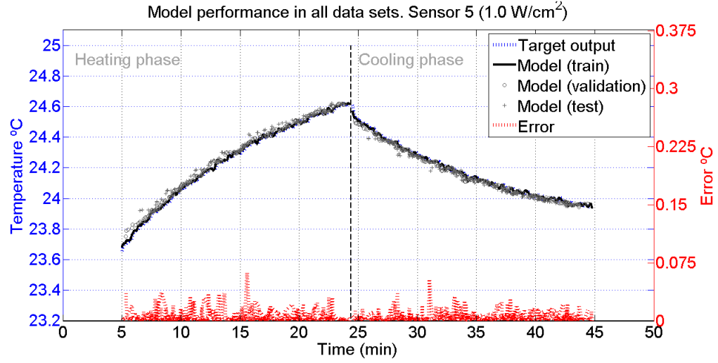
FIGURE C.18: Behaviour of the model through the whole data set, selected using the KTB approach. The blue line represents the desired behaviour and the model's training output is given by the black line. The error line is red, circle and cross markers represents the model's validation and test output respectively. SISP, homogeneous phantom experimental setup. TUS intensity: 1.0W/cm^2 . Sensor 5. Data used: uncorrupted.
