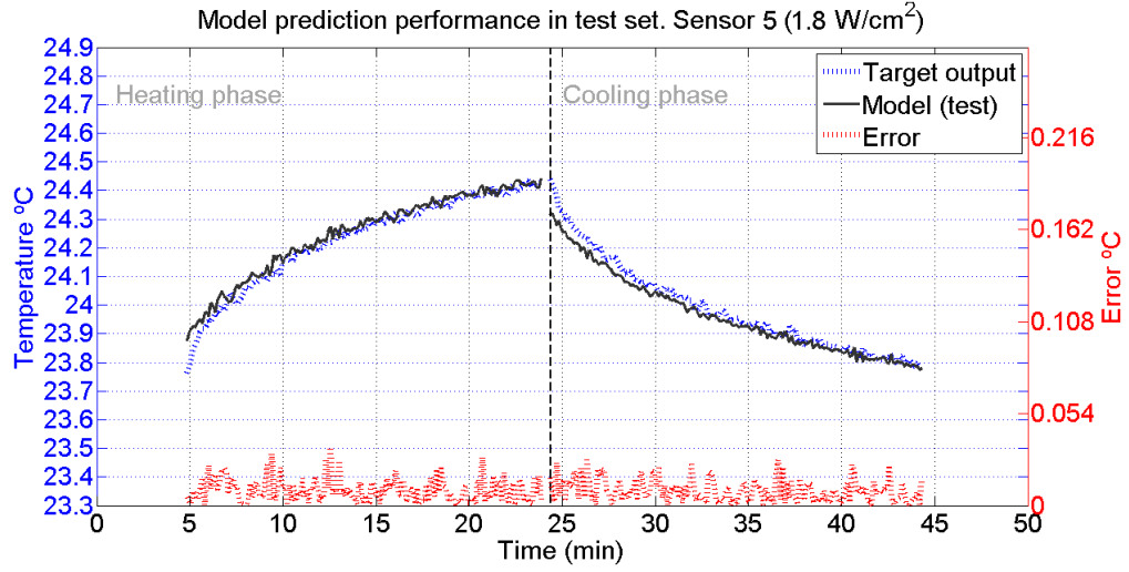
FIGURE E.3: Model's behaviour in the test set (Sensor 5 1.8W/cm^2 ), selected using the KTB approach. The blue line represents the desired behaviour and the model's test output is given by the black line. The error line is red. MIMP, homogeneous phantom experimental setup. Data used: uncorrupted.
