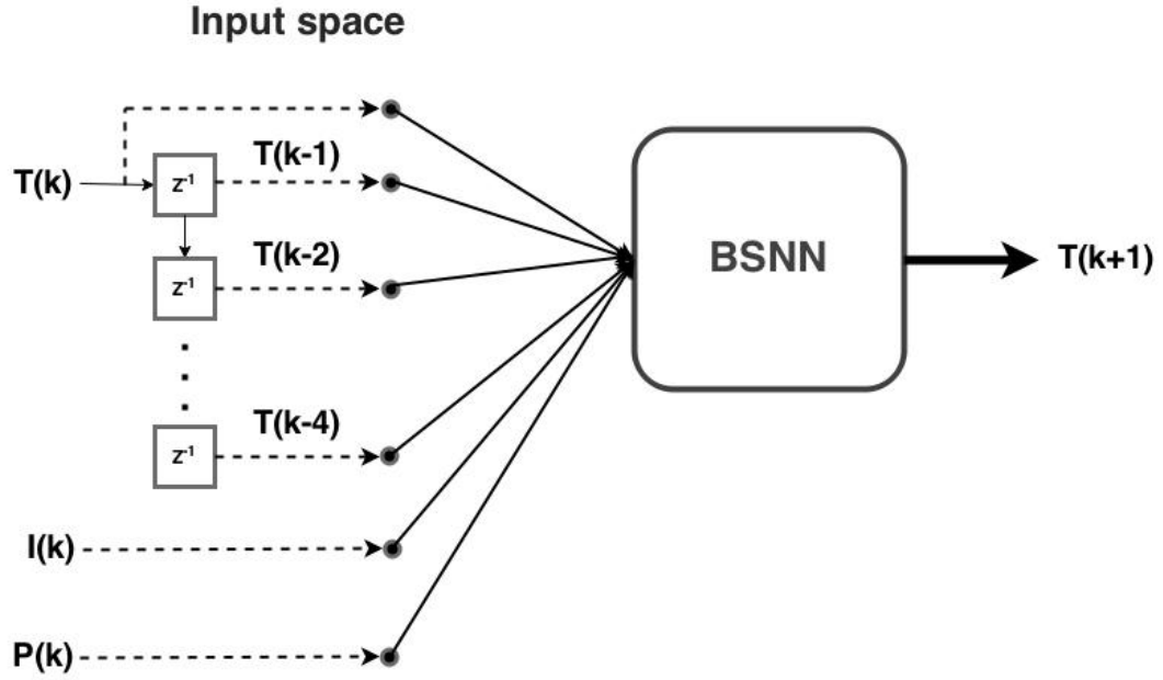
FIGURE 4.15: Predictive system architecture employing the traditional KTB method.
