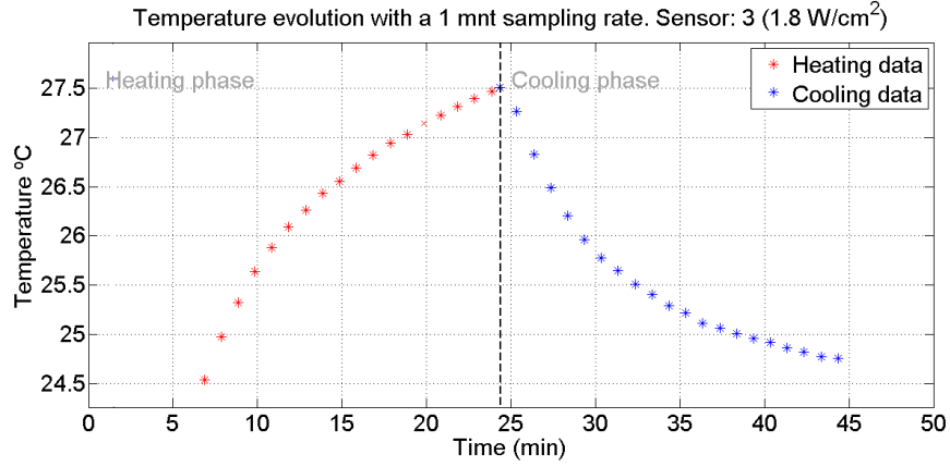
FIGURE 5.10: An example of a trial consisting of 40 temperature data points, divided between heating and cooling phase. Sampling period T = 60 seconds. Collected from the homogeneous phantom experimental setup.
