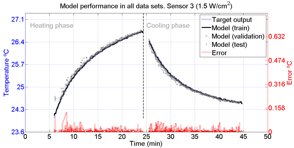
FIGURE C.10: Behaviour of the model through the whole data set, selected using the KTB approach. The blue line represents the desired behaviour and the model's training output is given by the black line. The error line is red, circle and cross markers represents the model's validation and test output respectively. SISP, homogeneous phantom experimental setup. TUS intensity: 1.5 \text{ W/cm}^2 . Sensor 3.
