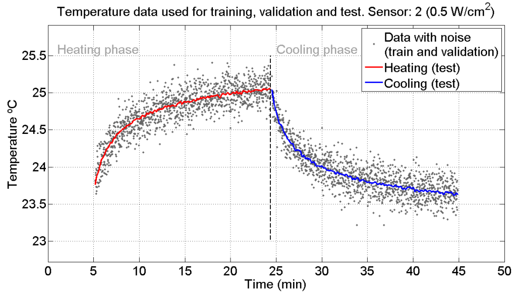
FIGURE C.7: Data after the addition of random Gaussian noise. The noisy data is used for training and validation. The Uncorrupted, noise free data is used to test the model. Collected from the homogeneous phantom experimental setup. TUS intensity: 0.5W/cm^2 . Sensor 2.
