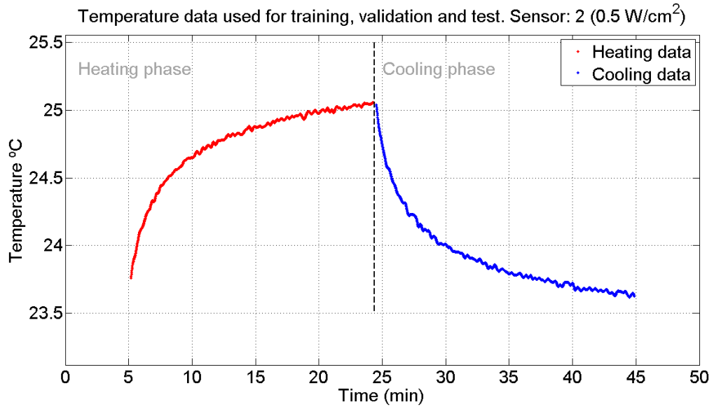
FIGURE C.5: Uncorrupted data set used for SPSI model training, validation and test. Collected from the homogeneous phantom experimental setup. TUS intensity: 0.5W/cm^2 . Sensor 2.
