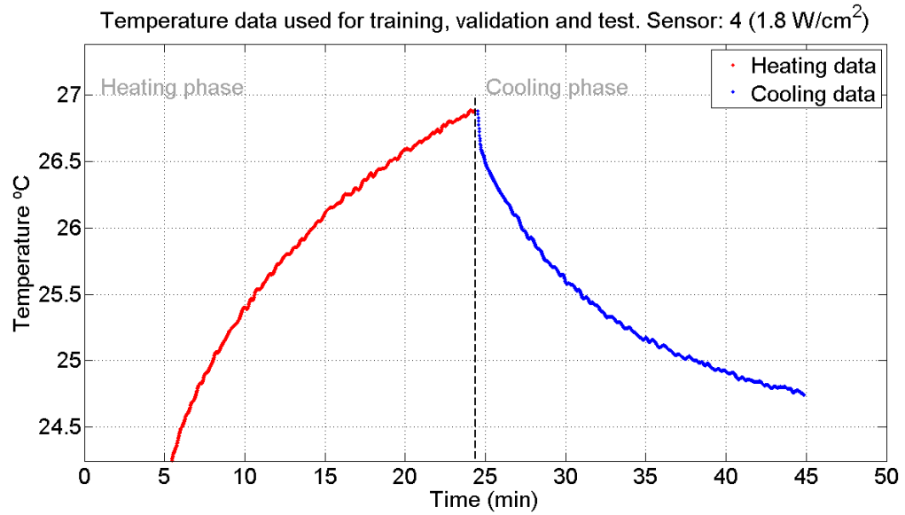
FIGURE C.13: Uncorrupted data set used for SPSI model training, validation and test. Collected from the homogeneous phantom experimental setup. TUS intensity: 1.8W/cm^2 . Sensor 4.
