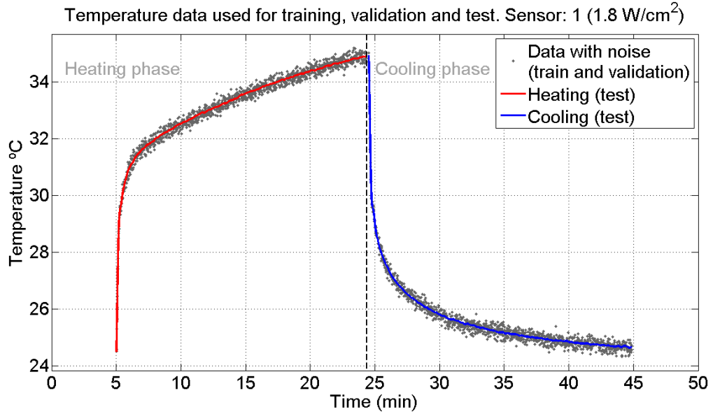
FIGURE C.3: Corrupted data after the addition of random Gaussian noise. The noisy data is used for training and validation. The Uncorrupted, noise free data is used to test the model. Collected from the homogeneous phantom experimental setup. TUS intensity: 1.8 \text{ W/cm}^2 . Sensor 1.
