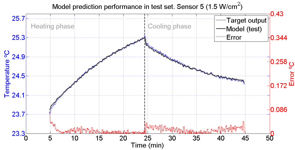
FIGURE D.9: Behaviour of model 4 in the test set (Sensor 5 1.5W/cm^2 ), selected using the KTB approach. The blue line represents the desired behaviour and the model's test output is given by the black line. The error line is red. SIMP, homogeneous phantom experimental setup. Data used: corrupted.
