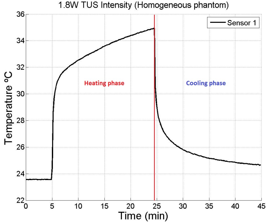
FIGURE 4.1: Two distinct phases can be observed in the temperature propagation. Firstly the temperature rises due to the ultrasound being applied to the phantom . After some time, the device is turned off and the phantom cools down naturally.
