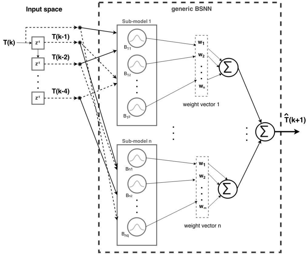
FIGURE 4.8: Network structure used in SPSI typology models.
