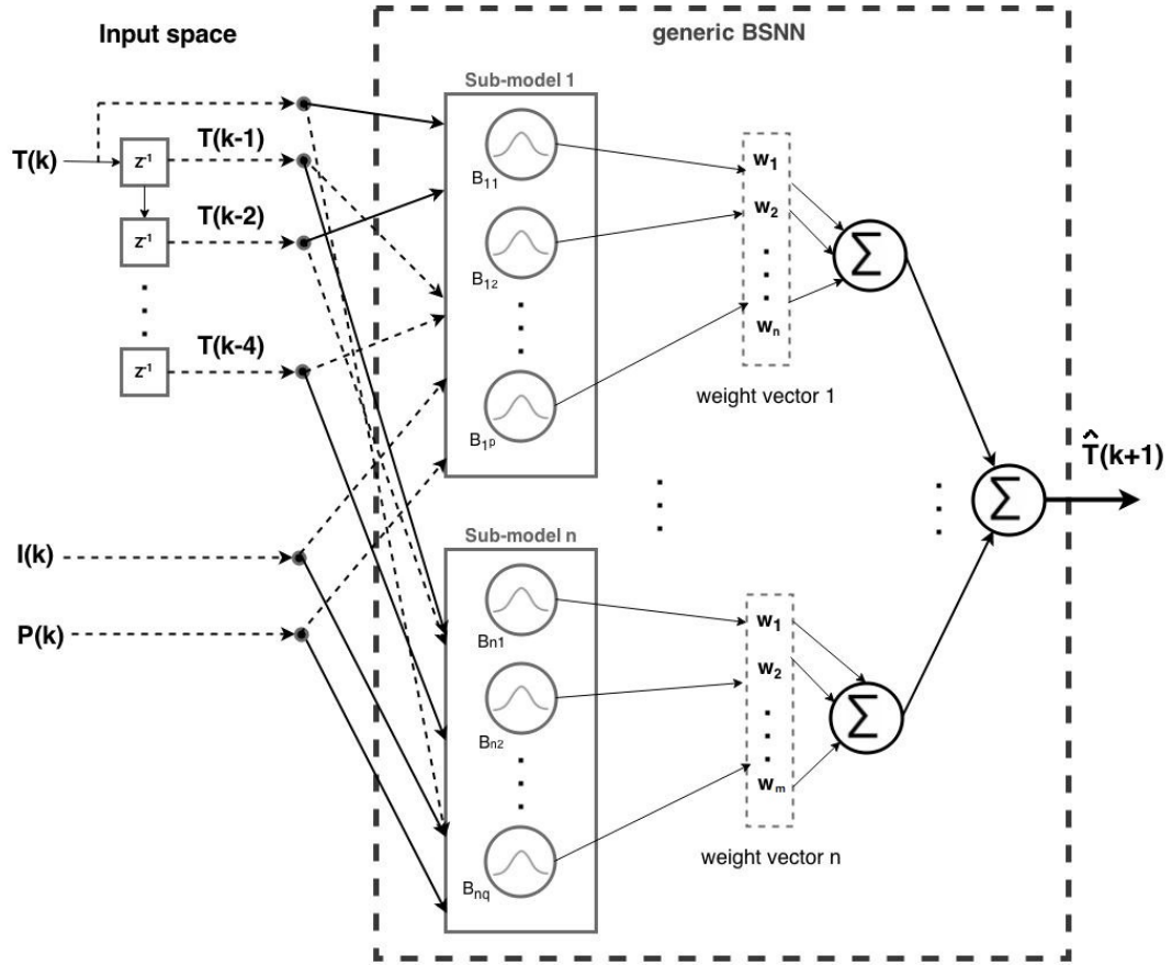
FIGURE 4.10: Network structure used in MPMI 1 – D typology models.
