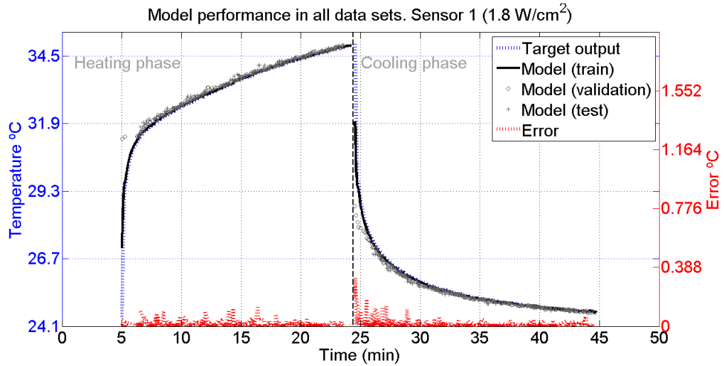
FIGURE C.2: Output curve of model 3 through the whole data set, selected using the KTB approach. The blue line represents the desired behaviour and the model's training output is given by the black line. The error line is red, circle and cross markers represents the model's validation and test output respectively. SISP, homogeneous phantom experimental setup. TUS intensity: 1.8 \text{ W/cm}^2 . Sensor 1. Data used: uncorrupted.
