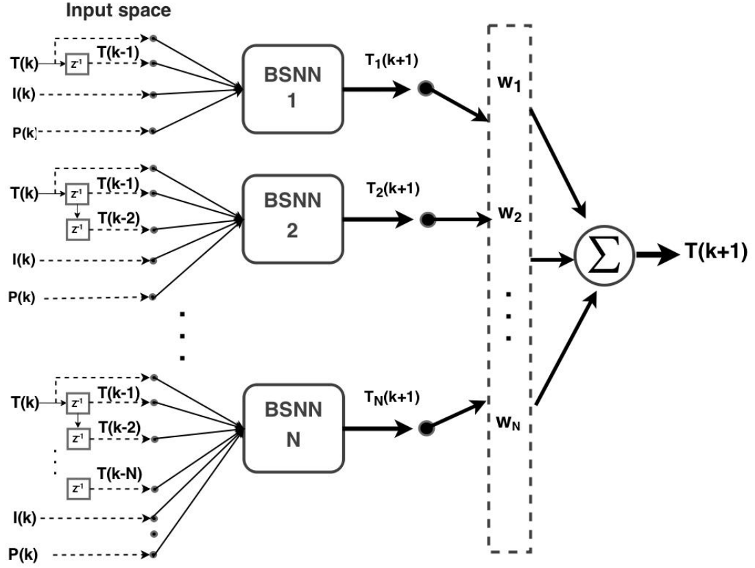
FIGURE 4.16: Predictive system architecture employing a neural network ensemble.
