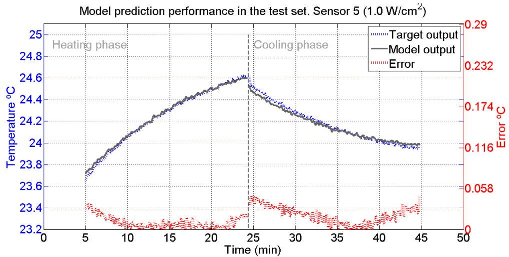
FIGURE C.20: Behaviour of model 3 in the test set, selected using the KTB approach. The blue line represents the desired behaviour and the model's test output is given by the black line. The error line is red. SISP, homogeneous phantom experimental setup. TUS intensity: 1.0 \text{ W/cm}^2 . Sensor 5. Data used: corrupted.
