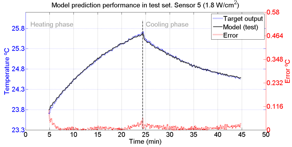
FIGURE D.10: Behaviour of model 4 in the test set (Sensor 5 1.8W/cm^2 ), selected using the KTB approach. The blue line represents the desired behaviour and the model's test output is given by the black line. The error line is red. SIMP, homogeneous phantom experimental setup. Data used: corrupted.
