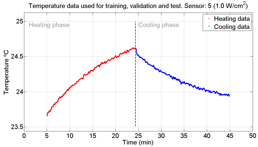
FIGURE C.17: Uncorrupted data set used for SPSI model training, validation and test. Collected from the homogeneous phantom experimental setup. TUS intensity: 1.0W/cm^2 . Sensor 5.
