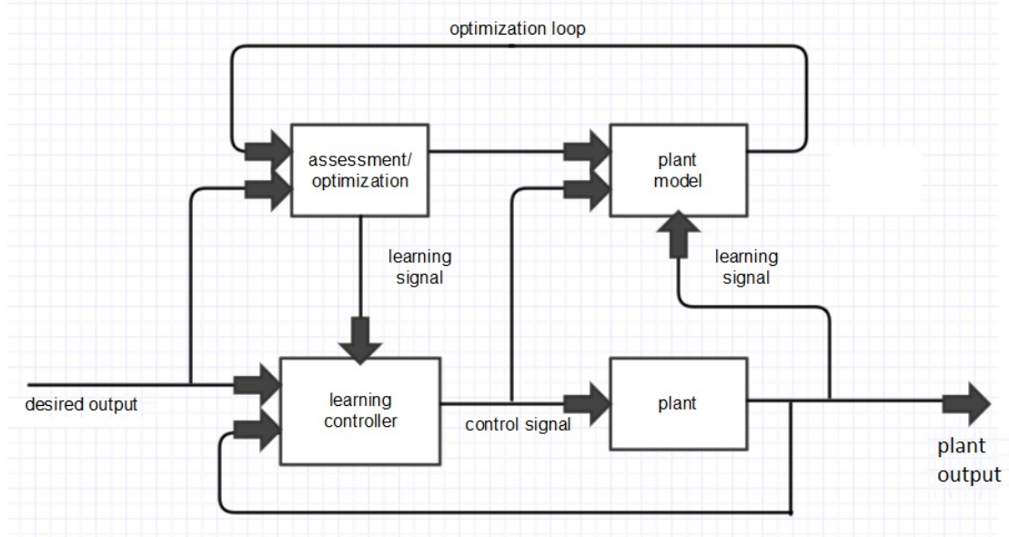
FIGURE 2.11: Predictive control architecture. Adapted from [5]
