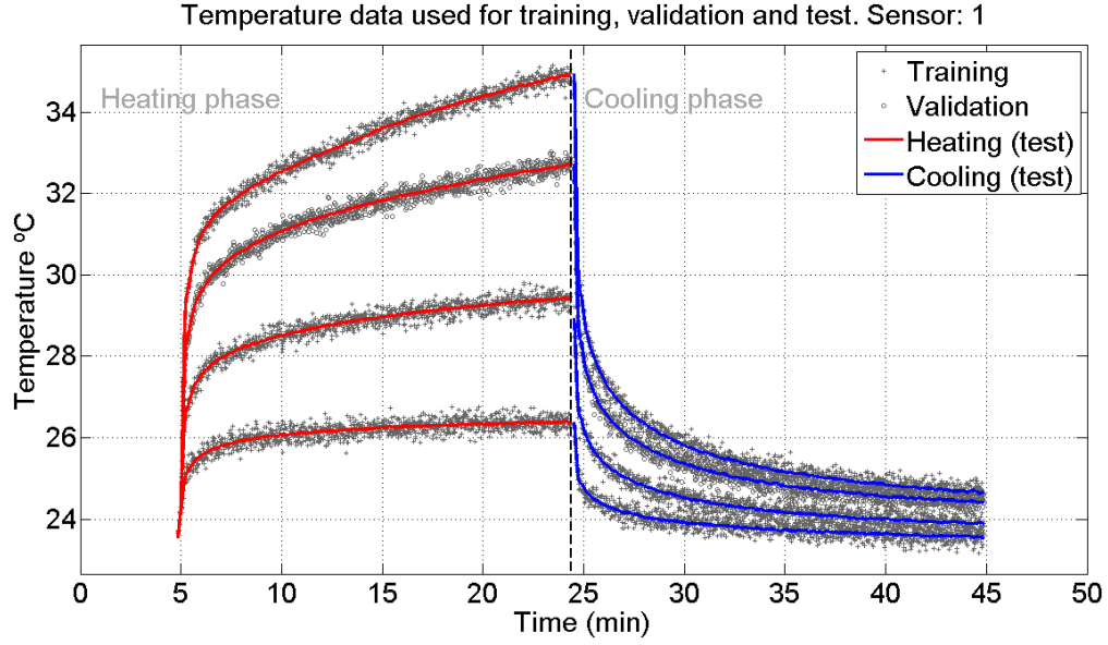
FIGURE 5.5: Data after the addition of random Gaussian noise. The noisy data is used for training and validation. The unaltered, noise free data is used to test the model. Collected from the homogeneous phantom experimental setup. The top curve corresponds to the strongest intensity. TUS intensity (from the shortest curve to the tallest curve): 0.5W/cm^2 , 1.0W/cm^2 , 1.5W/cm^2 and 1.8W/cm^2 . Sensor 1.
