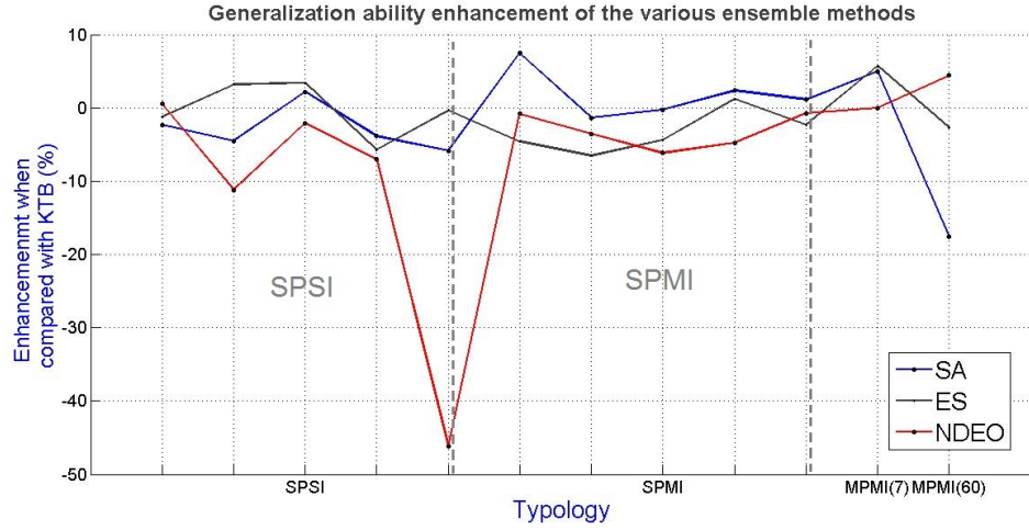
FIGURE 6.3: Ensemble methods performance enhancements of the various methods when compared with the KTB paradigm, regarding experiences where the models were build using uncorrupted data. SPSI and SPMI model typology both set 5 discrete points in the plot, whereas MPMI typologies just have one point. This is due to the fact that for the last typology all of the data universe had to be used, resulting in just one possible operating point: all sensors at all TUS beam intensities.
