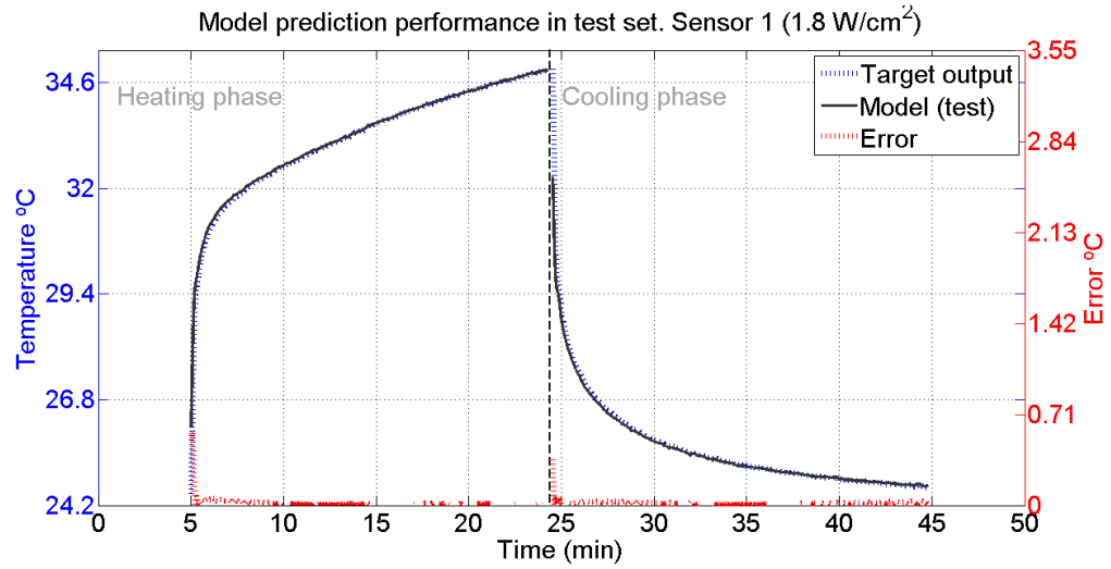
FIGURE 5.9: Behaviour of model 3 in the test set (Sensor 1 1.8W/cm^2 ), selected using the KTB approach. The blue line represents the desired behaviour and the model's test output is given by the black line. The error line is red. SIMP, homogeneous phantom experimental setup. Used data: corrupted.
