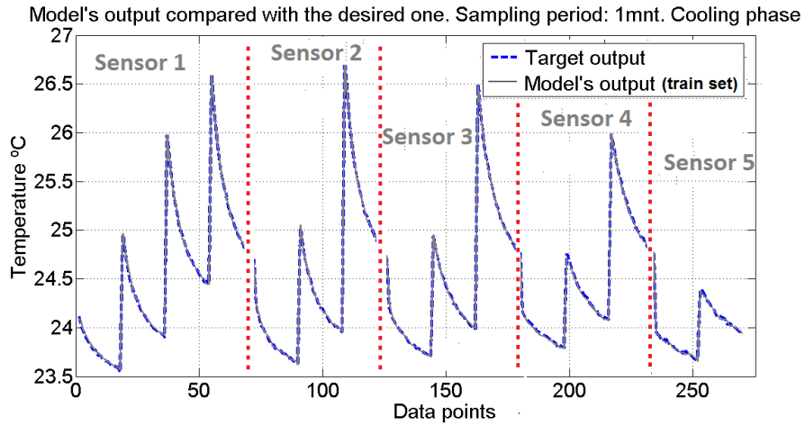
FIGURE 5.13: Top view from the output of model 3 concerning training set (cooling phase), selected using the KTB approach. The blue line represents the desired behaviour and the model's test output is given by the black line. homogeneous phantom experimental setup. The sensors labels just serve as a guidance. The model was constructed using the data illustrated in Figure (5.11). Data division during the model constructed followed the scheme exposed in Appendix(B), Model 2.
