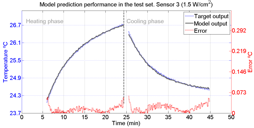
FIGURE C.12: Model's behaviour in the test set, selected using the KTB approach. The blue line represents the desired behaviour and the model's test output is given by the black line. The error line is red. SISP, homogeneous phantom experimental setup. TUS intensity: 1.5W/cm^2 . Sensor 3. Data used: corrupted.
