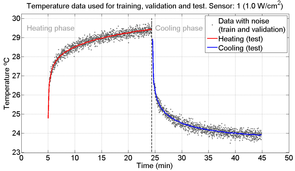
FIGURE 5.3: Data after the addition of random Gaussian noise. The noisy data is used for training and validation. The unaltered, noise free data is used to test the model. Collected from the homogeneous phantom experimental setup. TUS intensity: 1.0W/cm^2 . Sensor 1.
