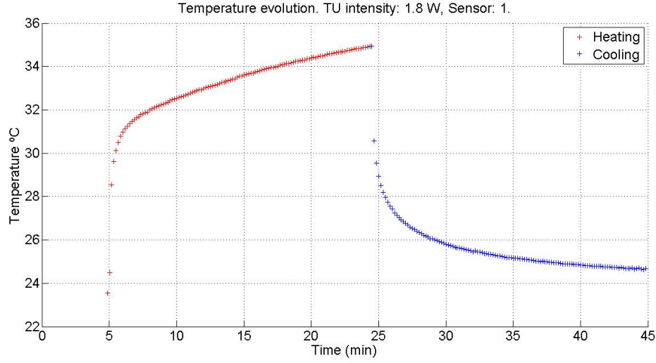
FIGURE 4.3: Data set collected from the homogeneous phantom experimental setup. TUS Intensity: 1.8W/cm^2 . Sensor: 1. The initial moments clearly exhibit a deficit of data, which can compromise the model learning potential over this region.
