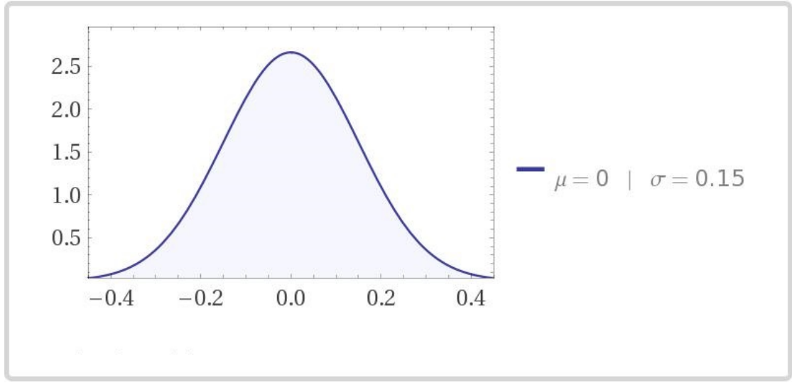
FIGURE 4.12: Gaussian distribution with \mu = 0 and \sigma = 0.15 .
