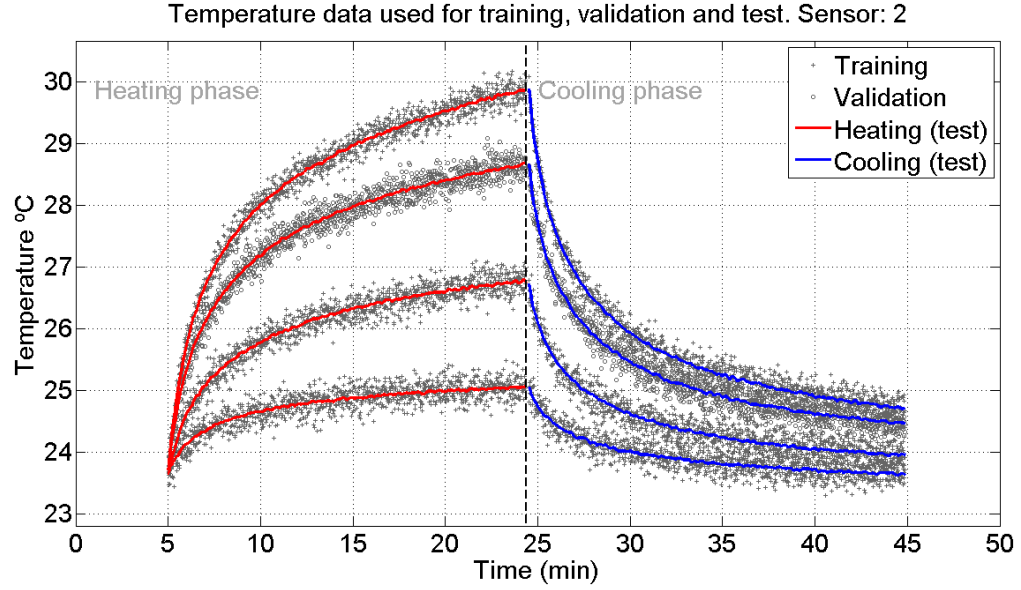
FIGURE D.1: Corrupted data after the completion of the Gaussian contamination process.. The noisy data is used for training and validation. The unaltered, noise free data is used to test the model. Collected from the homogeneous phantom experimental setup. The top curve corresponds to the strongest intensity. TUS intensity (from the shortest curve to the tallest curve): 0.5W/cm^2 , 1.0W/cm^2 , 1.5W/cm^2 and 1.8W/cm^2 . Sensor 1.
