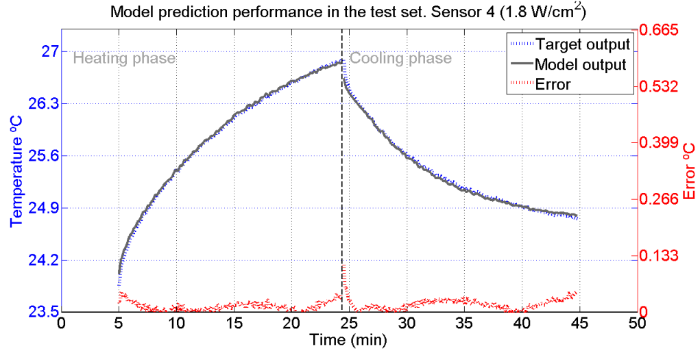
FIGURE C.16: Model's behaviour in the test set, selected using the KTB approach. The blue line represents the desired behaviour and the model's test output is given by the black line. The error line is red. SISP, homogeneous phantom experimental setup. TUS intensity: 1.8W/cm^2 . Sensor 4. Data used: corrupted.
