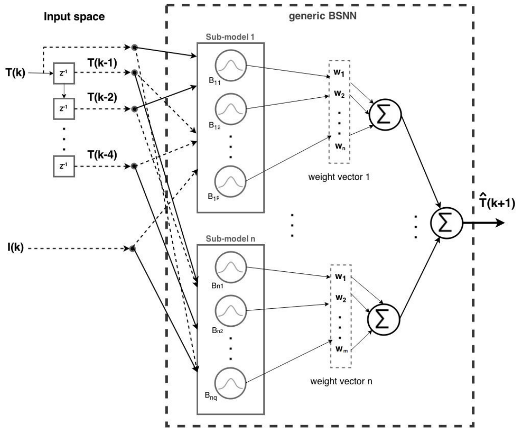
FIGURE 4.9: Network structure used in SPMI typology models.
