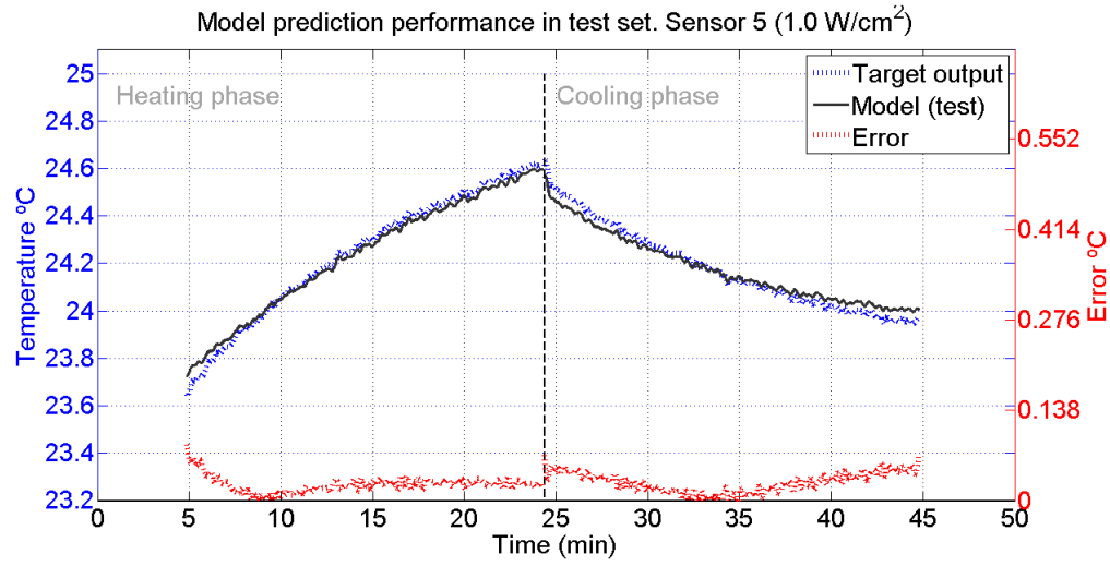
FIGURE D.8: Behaviour of model 4 in the test set (Sensor 5 1.0W/cm^2 ), selected using the KTB approach. The blue line represents the desired behaviour and the model's test output is given by the black line. The error line is red. SIMP, homogeneous phantom experimental setup. Data used: corrupted.
