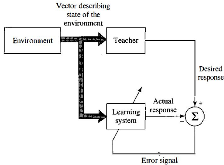
FIGURE 2.12: Block diagram of a learning process with a teacher. Adapted from [6]
