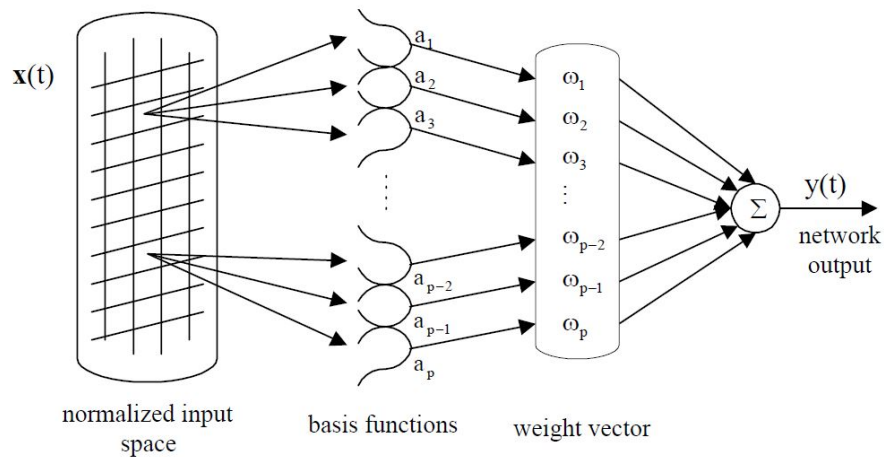
FIGURE 2.13: Associative memory network structure. Adapted from [4].
