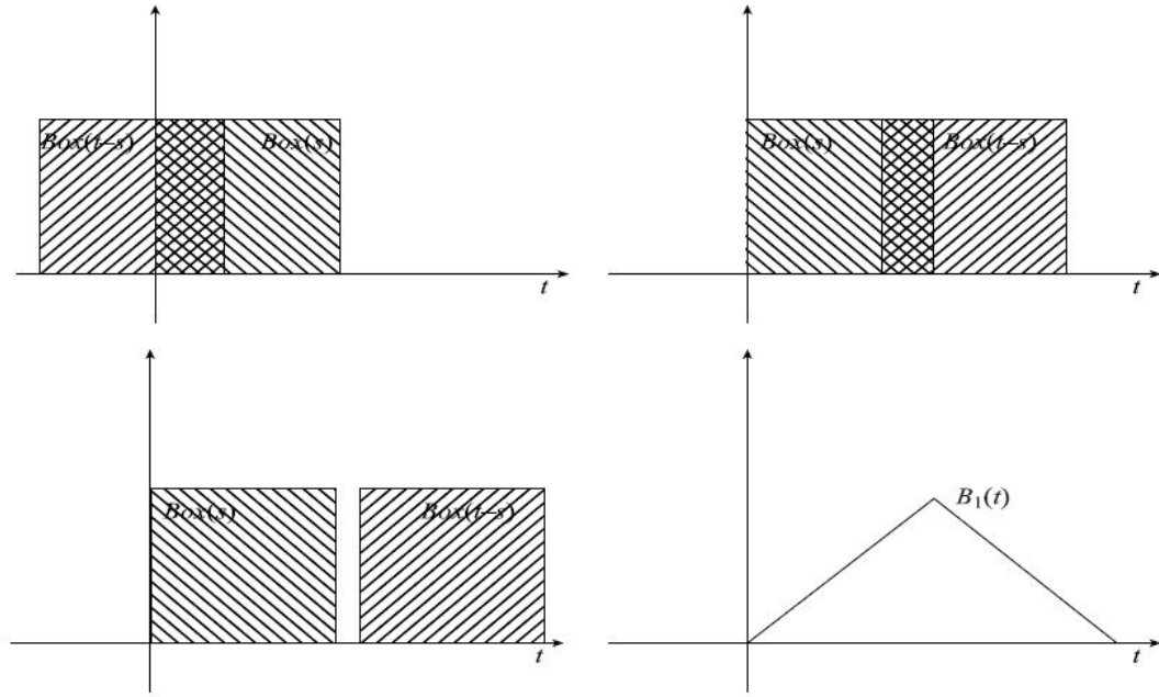
FIGURE A.1: Defining a BS of order 2 through the use of convolution operation. Adapted from [9]
