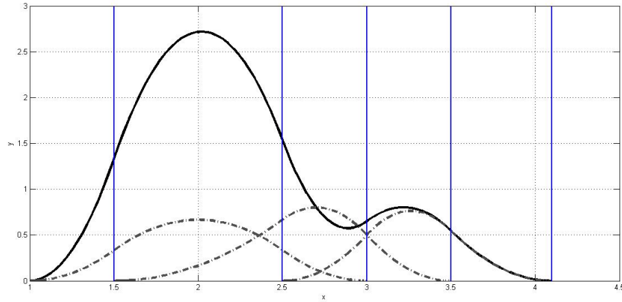
FIGURE 2.8: Spline function of order 3 resulting from changing the control vector. The blue lines indicate the position of knot, the gray dashed lines represent the B-splines, and the solid black line shows the resulting spline function. Figure generated with MATLAB, using the Curve Fitting Toolbox [3]
