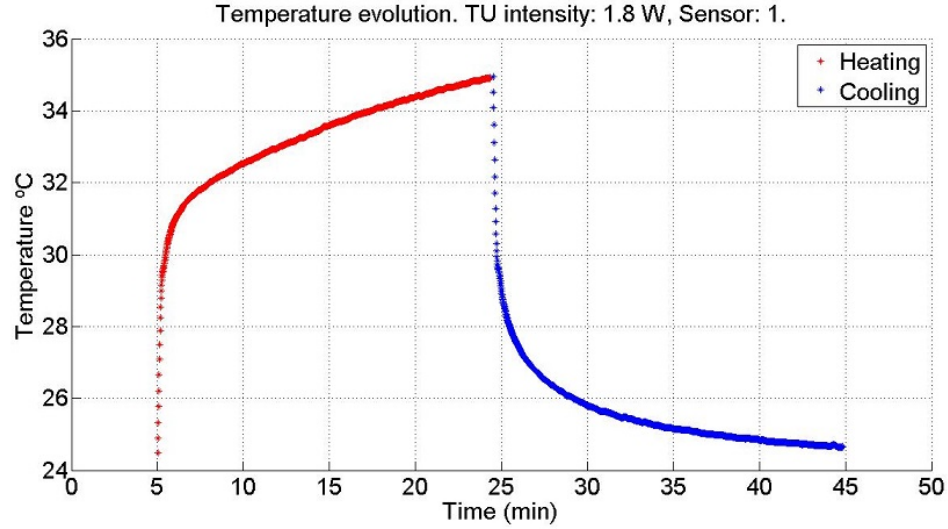
FIGURE 4.5: Interpolation result, applied to the data illustrated in Figure (4.4). The results exhibit a more robust and compact data set, assigning more knowledge about the process to the deficient areas.
