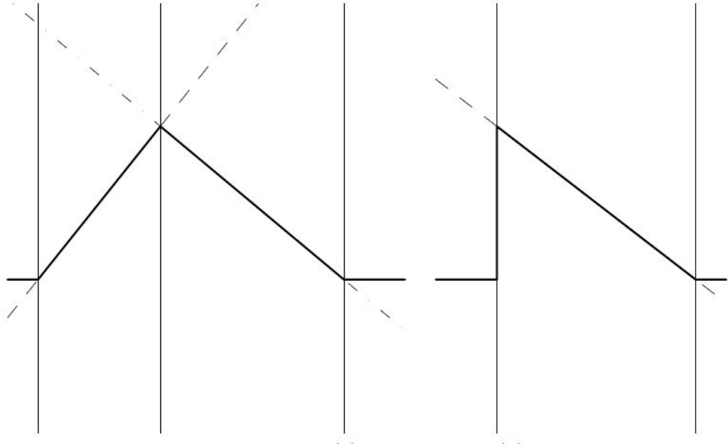
FIGURE 2.4: BS of order 2 with (a) simple knots, (b) a double knot. Adapted from [2]
