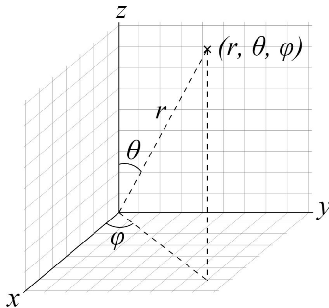
FIGURE 6.5: Spherical coordinates (r, \theta, \phi) as commonly used in physics: radial distance r , polar angle \theta (theta), and azimuthal angle \phi (phi). Taken from [3]
