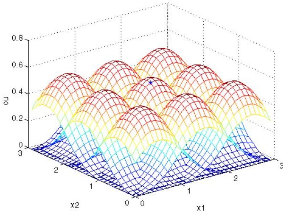
FIGURE 2.10: Two-dimensional multivariable basis functions formed with order 3 univariate basis functions. Adapted from [4].
