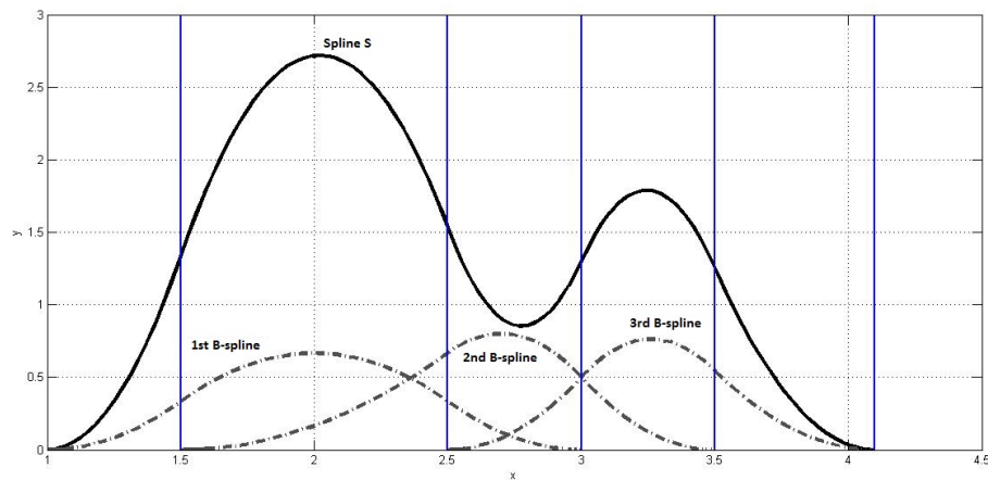
FIGURE 2.7: Spline function of order 3, constructed by linearly combining three B-splines of order 3. The blue lines indicate the position of knot, the gray dashed lines represent the B-splines, and the solid black line shows the resulting spline function. Control points employed a = [4 \ 0.3 \ 2.3] . Figure generated with MATLAB, using the Curve Fitting Toolbox [3]
