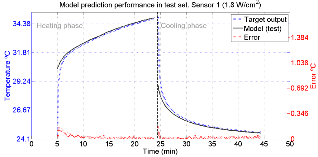
FIGURE E.5: Model's behaviour in the test set (Sensor 1 1.8W/cm^2 ), selected using the KTB approach. The blue line represents the desired behaviour and the model's test output is given by the black line. The error line is red. MIMP, homogeneous phantom experimental setup.
