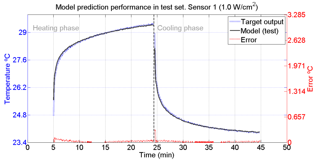
FIGURE 5.7: Behaviour of model 3 in the test set (Sensor 1 1.0 \text{ W/cm}^2 ), selected using the KTB approach. The blue line represents the desired behaviour and the model's test output is given by the black line. The error line is red. SIMP, homogeneous phantom experimental setup. Used data: corrupted.
