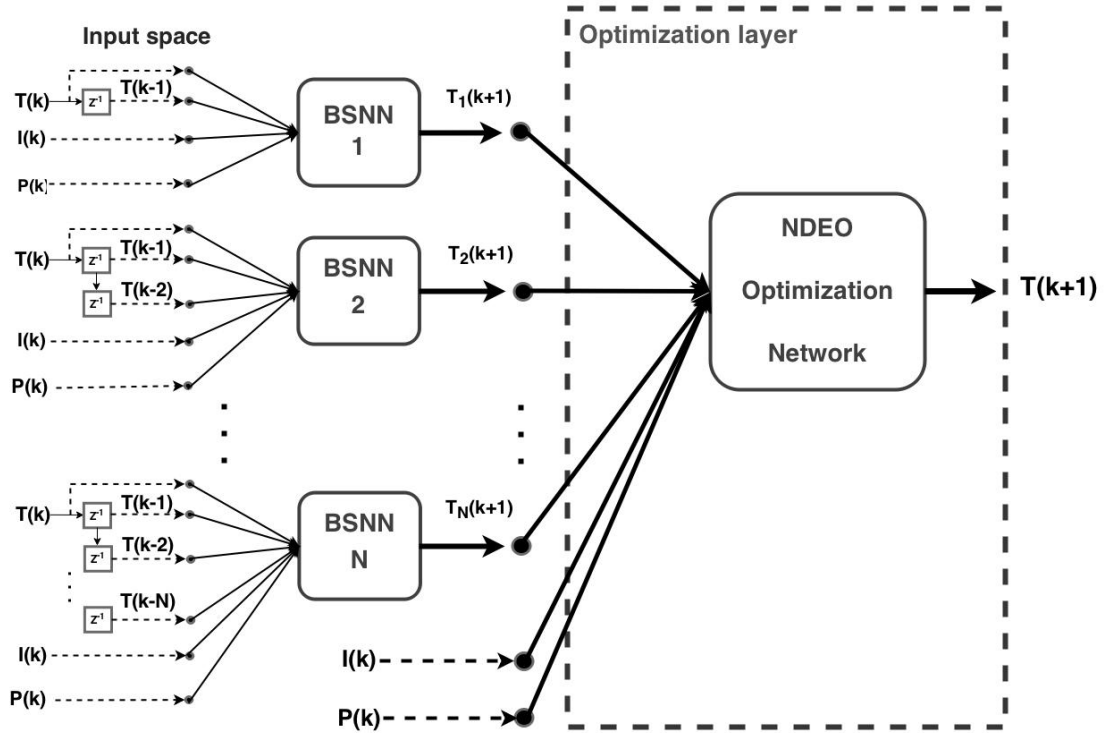
FIGURE 4.17: Predictive system architecture employing NDEO.
