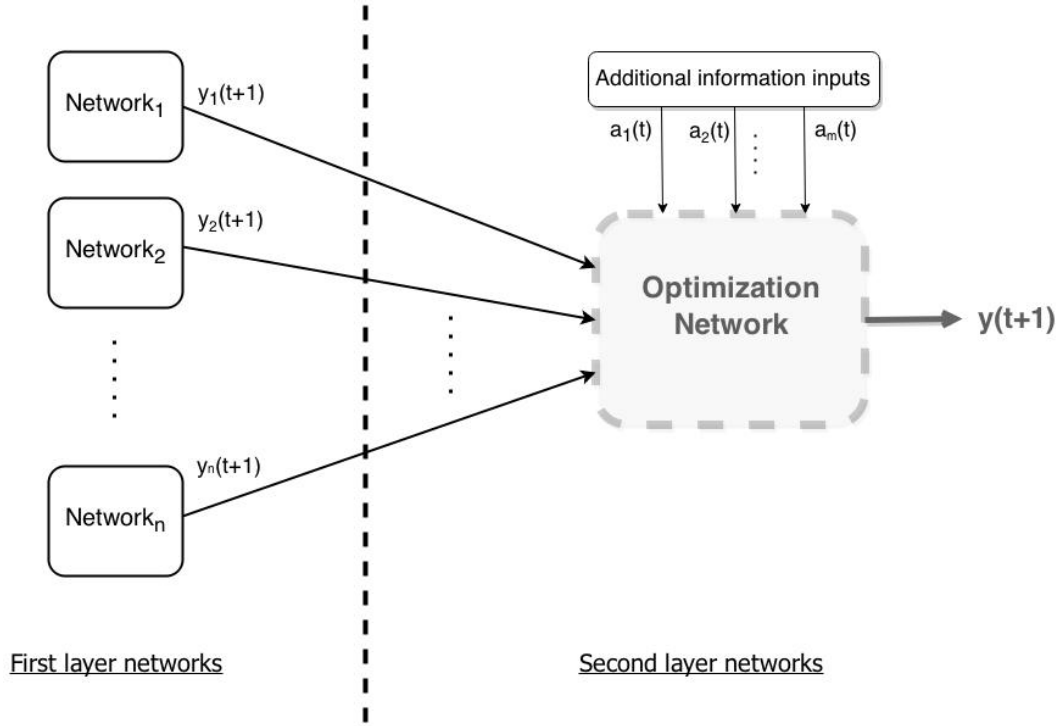
FIGURE 2.18: Purposed architecture for a neural ensemble system, employing NDEO.
