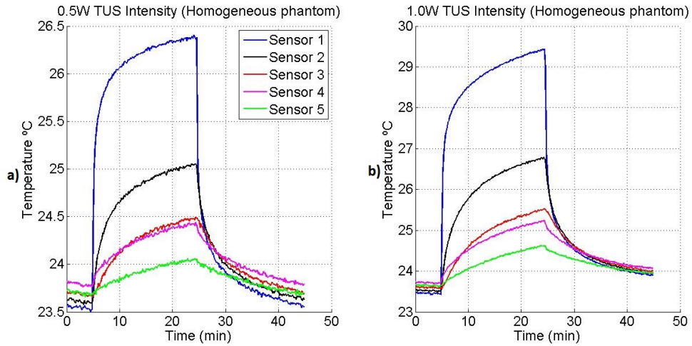
FIGURE 3.5: Temperature recorded by the temperature sensors in the experiment described in Section (3.3), considering a beam intensity of: a) 0.5W/cm^2 and b) 1.0W/cm^2 .
