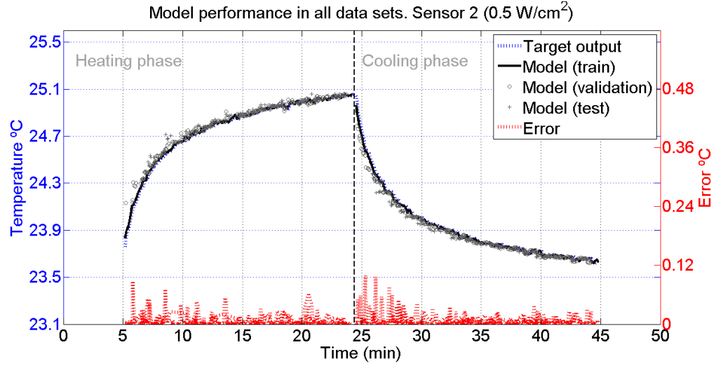
FIGURE C.6: Behaviour of the model 1 through the whole data set, selected using the KTB approach. The blue line represents the desired behaviour and the model's training output is given by the black line. The error line is red, circle and cross markers represents the model's validation and test output respectively. SISP, homogeneous phantom experimental setup. TUS intensity: 0.5W/cm^2 . Sensor 2. Data used: uncorrupted.
