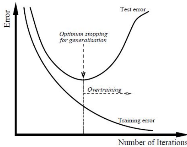
FIGURE 2.16: Illustration of the early-stopping rule based on cross-validation. [6].
