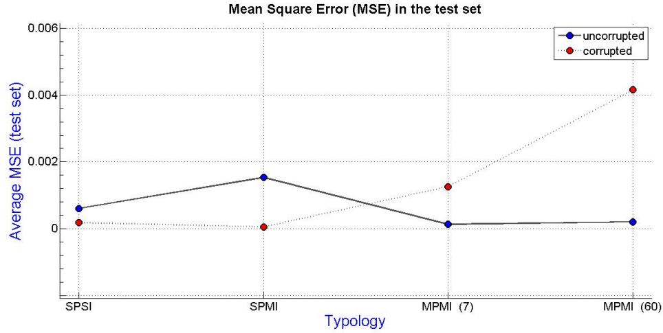
FIGURE 6.1: Graphical illustration of the average MSE (test set) calculated for all models typologies, using uncorrupted and Gaussian contaminated data. Solid line: values obtained with uncorrupted data; Dashed line: vales obtained with corrupted data.
