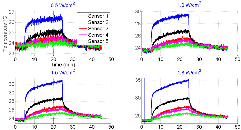
FIGURE 5.17: Data after the addition of random Gaussian noise. The noisy data is used for training and validation. The unaltered, noise free data is used to test the model. Collected from the homogeneous phantom experimental setup.
