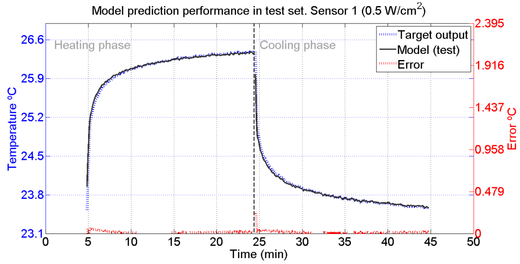
FIGURE 5.6: Behaviour of model 3 in the test set (Sensor 1 0.5 \text{ W/cm}^2 ), selected using the KTB approach. The blue line represents the desired behaviour and the model's test output is given by the black line. The error line is red. SIMP, homogeneous phantom experimental setup. Used data: corrupted.
