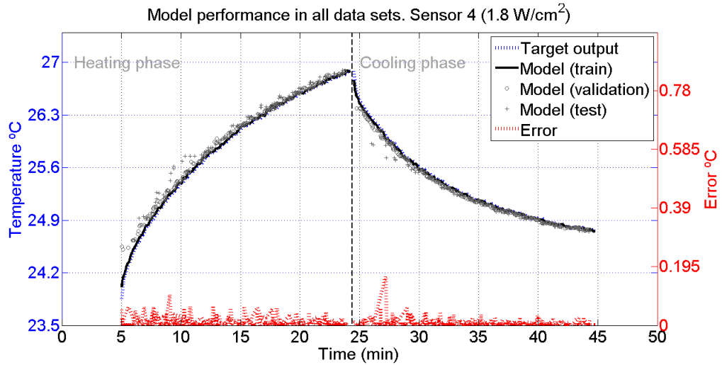
FIGURE C.14: Behaviour of the model through the whole data set, selected using the KTB approach. The blue line represents the desired behaviour and the model's training output is given by the black line. The error line is red, circle and cross markers represents the model's validation and test output respectively. SISP, homogeneous phantom experimental setup. TUS intensity: 1.8 \text{ W/cm}^2 . Sensor 4. Data used: uncorrupted.
