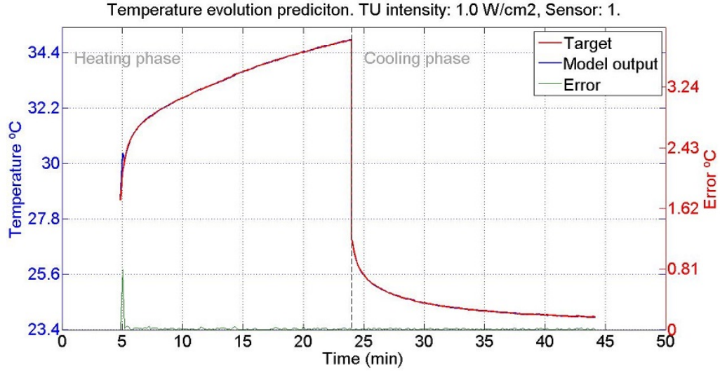
FIGURE 4.4: Results comparison between a model prediction and desired observed values. TUS Intensity: 1.0W/cm^2 . Sensor: 1. The green line represents the absolute error evaluated through all the data set. The effects of the lack of data points are visible, in the initial moments when the temperature is rising rapidly.
