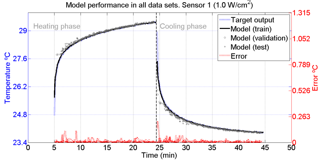
FIGURE 5.2: Behaviour of model 2 through the whole data set, selected using the KTB approach. The blue line represents the desired behaviour and the model's training output is given by the black line. The error line is red, circle and cross markers represents the model's validation and test output respectively. SISP, homogeneous phantom experimental setup. TUS intensity: 1.0\text{ W/cm}^2 . Sensor 1. Used data: uncorrupted
