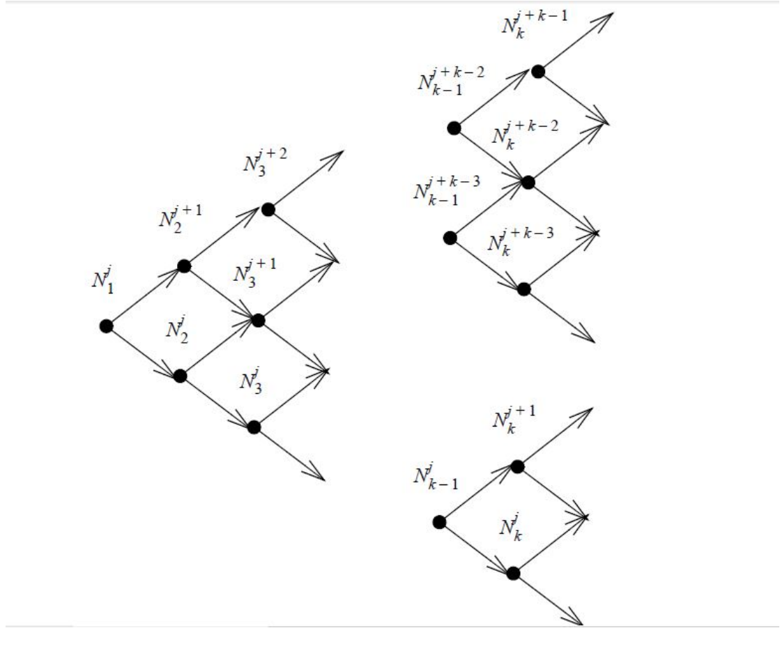
FIGURE 2.9: Triangular array used for evaluating k BSs of order k . [4]
