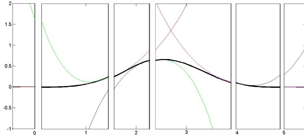
FIGURE 2.5: B-spline of order 4 with knot sequence t = [0 \ 1.5 \ 2.3 \ 4 \ 5] . Each interval, with the respective color, represents one piece of the basis function. Figure generated with MATLAB, using the Curve Fitting Toolbox [3]
