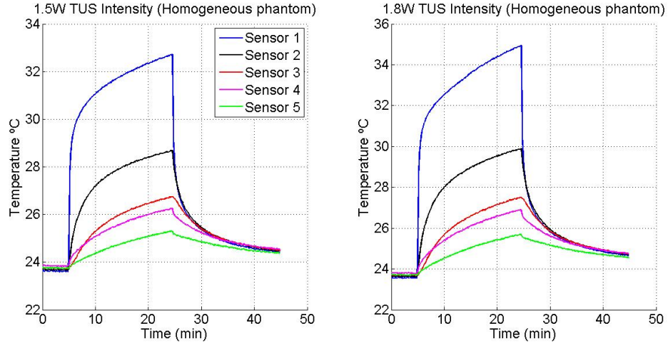
FIGURE 3.6: Temperature recorded by the temperature sensors in the experiment described in Section (3.3), considering a beam intensity of: a) 1.5W/cm^2 and b) 1.8W/cm^2 .
