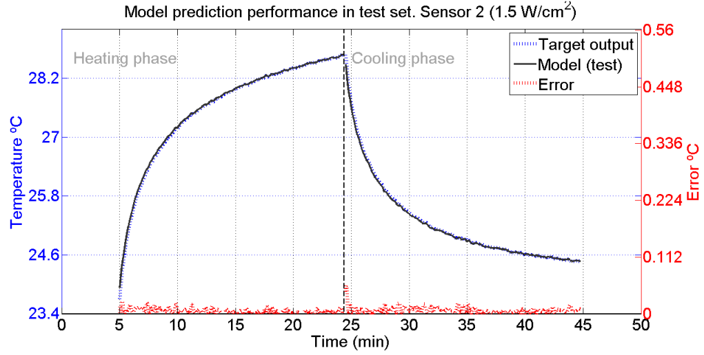
FIGURE D.4: Behaviour of model 4 in the test set (Sensor 2 1.5W/cm^2 ), selected using the KTB approach. The blue line represents the desired behaviour and the model's test output is given by the black line. The error line is red. SIMP, homogeneous phantom experimental setup. Data used: corrupted.
