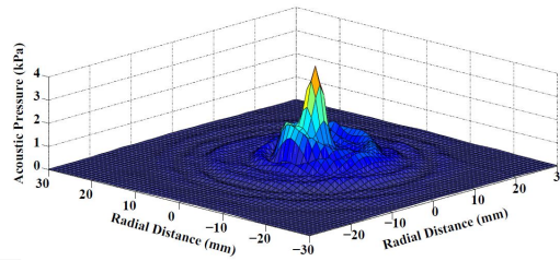
FIGURE 3.2: Pressure field of the therapeutic transducer measured in a plan parallel to the face and at 48mm distance. Figure taken from [8].
