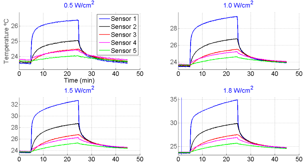
FIGURE E.1: Uncorrupted data set used for MPMI model training, validation and test. Collected from the homogeneous phantom experimental setup.
