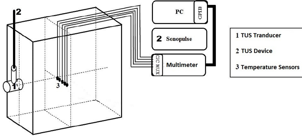
FIGURE 3.3: Schematic diagram of the experiment setup used in the first environment, homogeneous phantom . Figure adapted [7].
