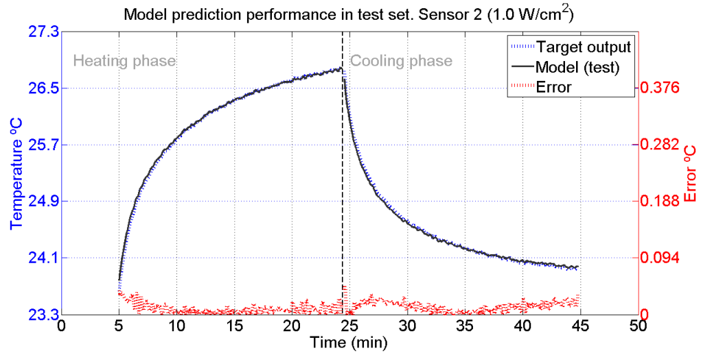
FIGURE D.3: Behaviour of model 4 in the test set (Sensor 2 1.0W/cm^2 ), selected using the KTB approach. The blue line represents the desired behaviour and the model's test output is given by the black line. The error line is red. SIMP, homogeneous phantom experimental setup. Data used: corrupted.
