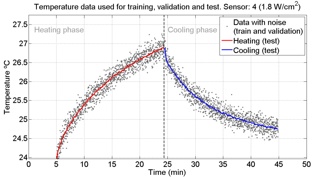
FIGURE C.15: Data after the addition of random Gaussian noise. The noisy data is used for training and validation. The Uncorrupted, noise free data is used to test the model. Collected from the homogeneous phantom experimental setup. TUS intensity: 1.8 \text{ W/cm}^2 . Sensor 4.
