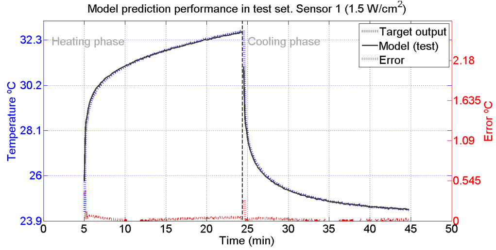
FIGURE 5.8: Behaviour of model 3 in the test set (Sensor 1 1.5W/cm^2 ), selected using the KTB approach. The blue line represents the desired behaviour and the model's test output is given by the black line. The error line is red. SIMP, homogeneous phantom experimental setup. Used data: corrupted.
