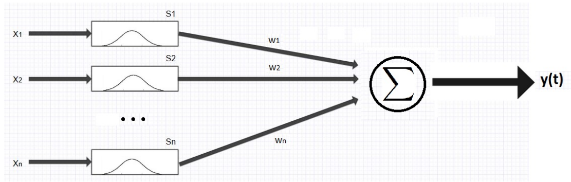
FIGURE 2.15: Additive decomposition of the network.
