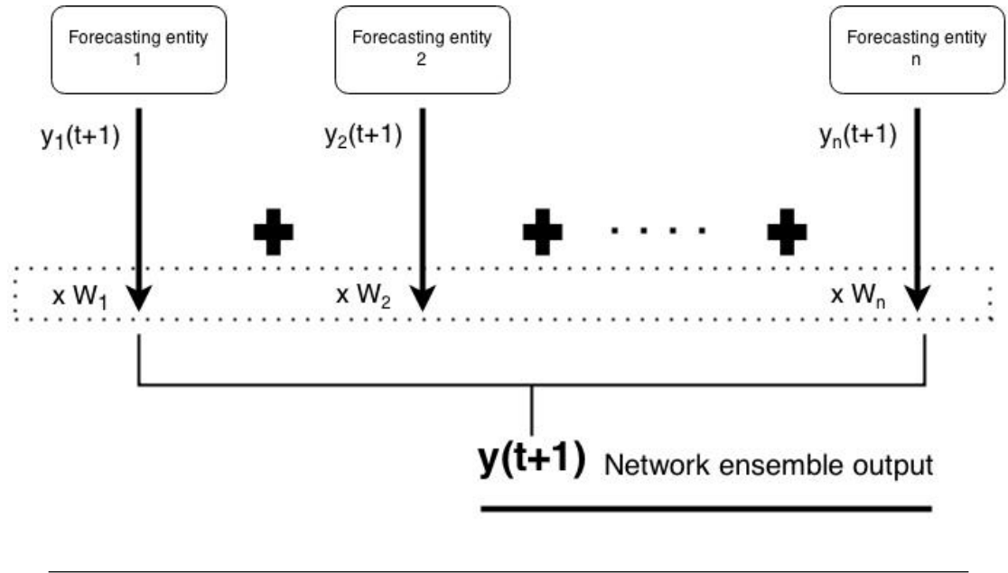
FIGURE 2.17: Weighted combination of forecasts.
