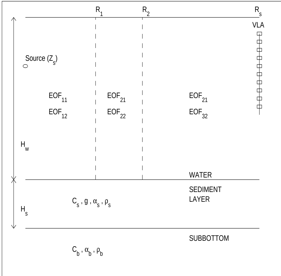
Figure 2.1: Waveguide model.
