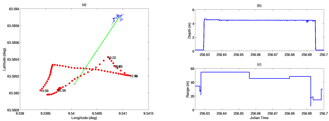
Figure 2.13: Day 256, September 13, 2008: target GPS estimated position (a), source depth (b) and source - target range (c).
