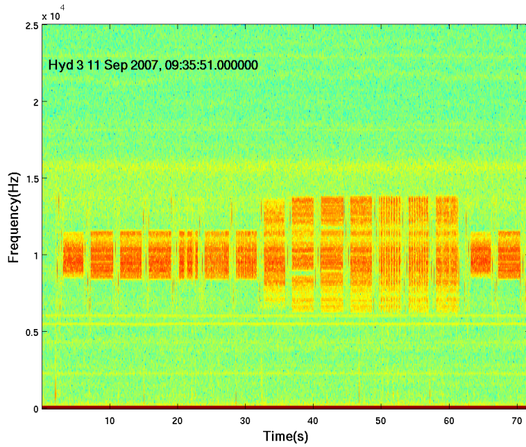
Figure 3.7: Day 254: OFDM communication signals for source testing as received on hydrophone 1 (6.6 m depth).
