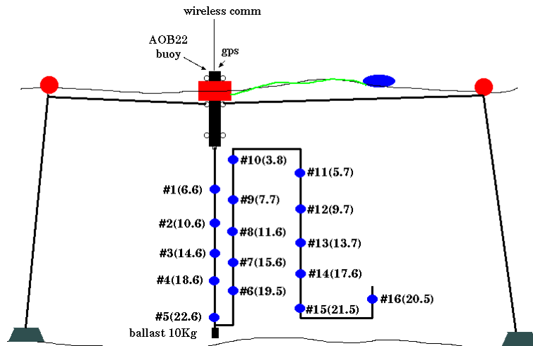
Figure 2.10: sketch of the AOB folded receiver array during the mooring at Sletvik.
