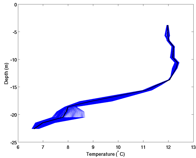
Figure 2.5: low-pass filtered AOB22 temperature profiles from thermistor string data for the first 10 minutes of day 254; thick line is the mean temperature profile.
