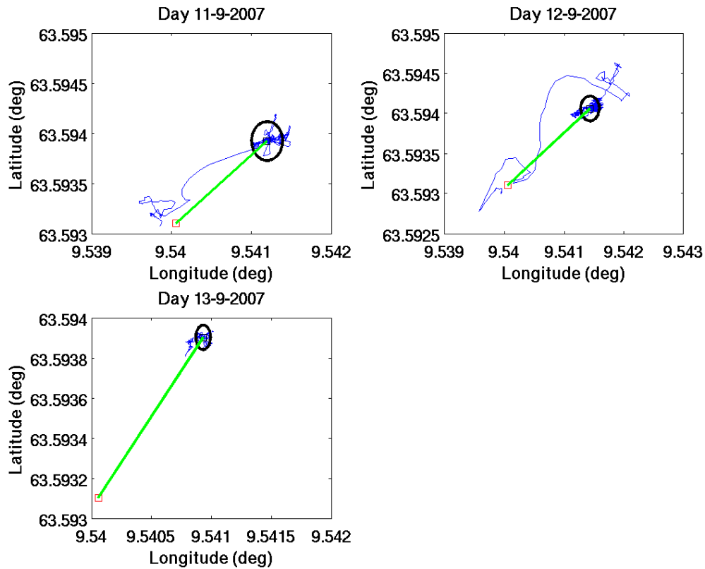
Figure 2.11: AOB22 GPS position during the Hopavågen bay deployments of days 11, 12 and 13 of September, 2007: source position (red square), mean array position (black square), one standard deviation on GPS position of receiving array (thick circle), mean acoustic barrier position (green line).
