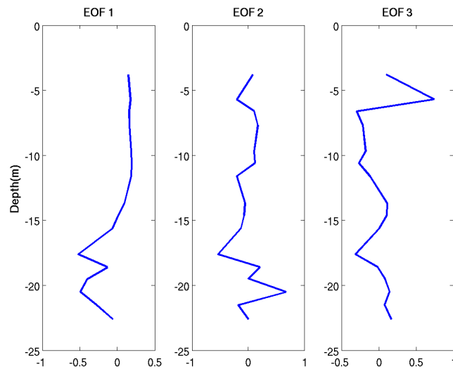
Figure 2.6: first three EOF's computed from thermistor chain data during the Hopavågen bay part of the UAB07 experiment.
