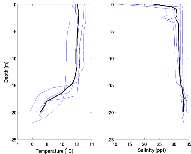
Figure 2.2: Mean temperature and salinity profiles from archival data for the month of September of the last 10 years (1996 - 2006) for the Hopvåagen bay.
