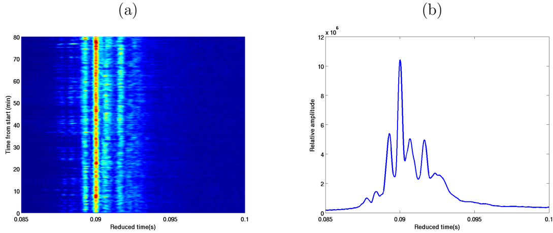
Figure 3.10: Day 255 hydrophone 5 at 22.6 m depth, 0.5 s LFM sweeps in the 7.5 - 10.5 kHz band, start time 10:31 UTC: time variability (a) and mean arrival pattern (b).
