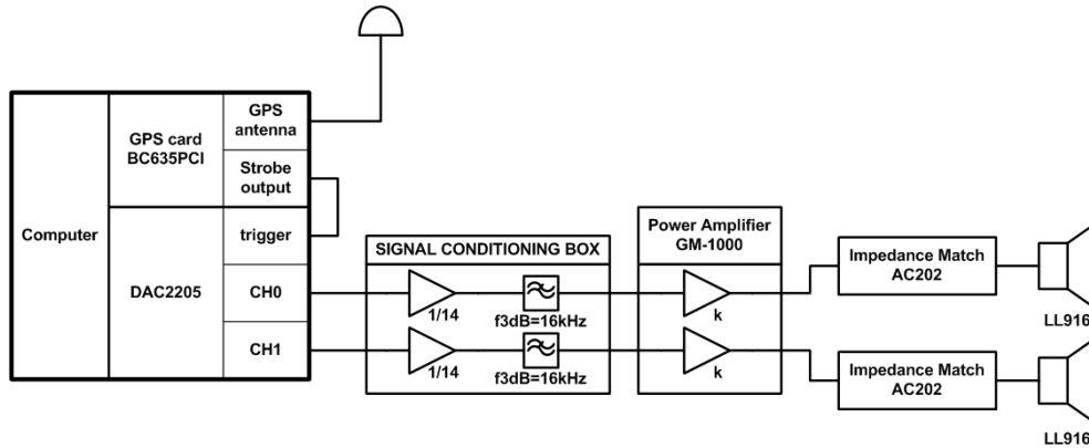
Figure 3.3: Signal generation system used during the Hopavågen bay phase of UAB07.
