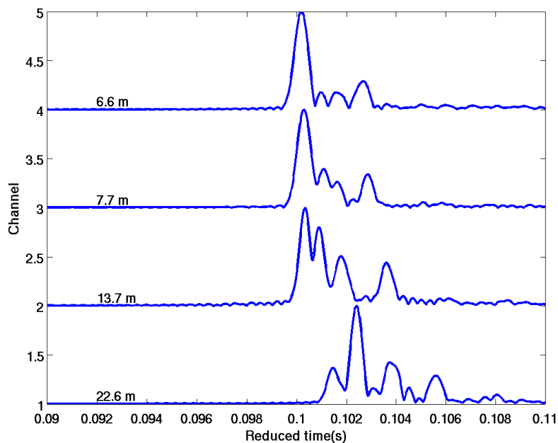
Figure 3.6: Day 254 14:12 UTC: pulse compression of channels 1, 5, 9 and 13 at respective depths of 6.6, 22.6, 7.7 and 13.7 meter [LF upsweep 0.2 s duration in the LF band: 3500-6500 Hz].
