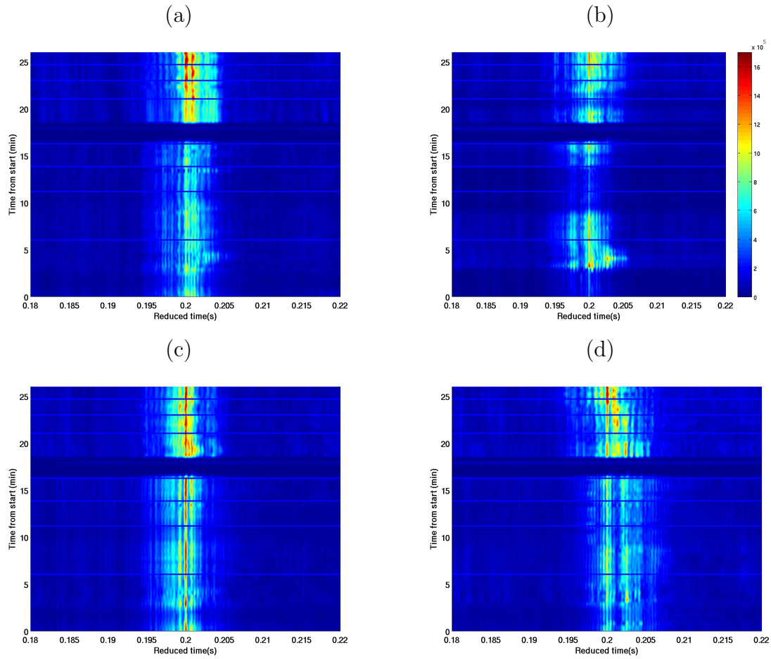
Figure 3.13: Day 256 correlations with HF downswEEP pulse starting at 16:01 UTC for channels: 1 at 6.6 m depth (a), 9 at 7.7 m depth (b), 13 at 13.7 m depth (c) and 5 at 22.6 m depth (d). Signal transmission was interrupted and re-initialized at 16:18 UTC. Horizontal lines mark the target crossings of the virtual barrier according to measured time of table 2.3.
