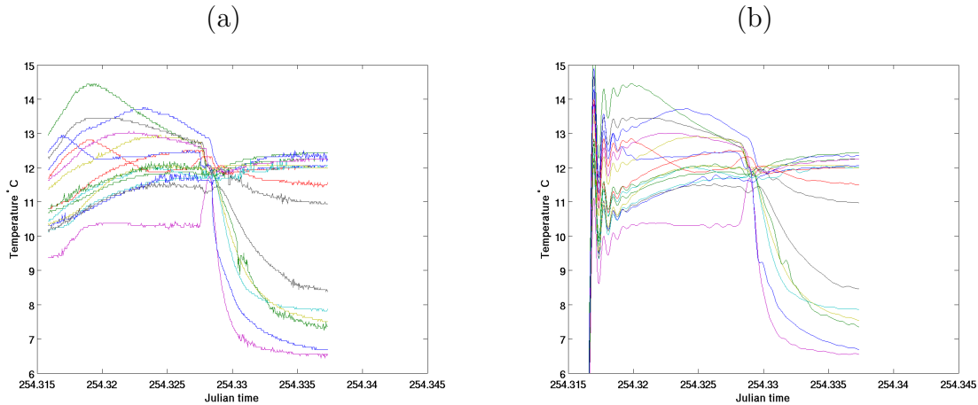
Figure 2.4: AOB22 thermistor string data for day 254 unfiltered (a) and lowpass filtered (b).
