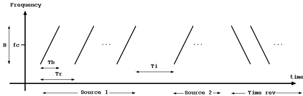
Figure 3.2: Time - frequency sketch of the typical transmit sequence.
