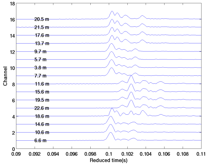
Figure 3.5: Day 254 14:12 UTC: pulse compression of all channels with LFM upsweep 0.2 s duration in the band LF band: 3500 - 6500 Hz.
