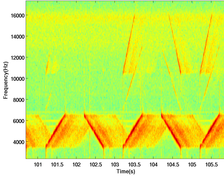
Figure 3.8: Day 254 hydrophone 1 (6.6 m depth): up - down sweeps in the lower 5 kHz band and corresponding harmonics.
