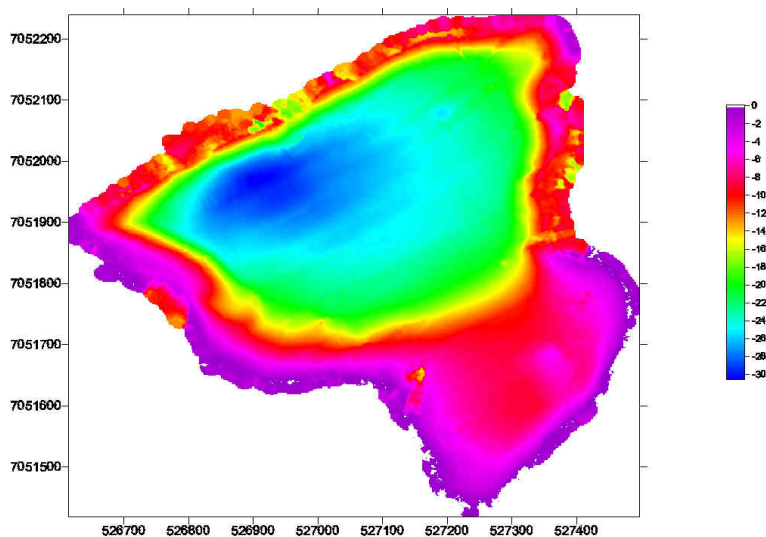
Figure 2.3: Bathymetry recording of the Hopavågen bay (courtesy of NTNU / Bates [1]).
