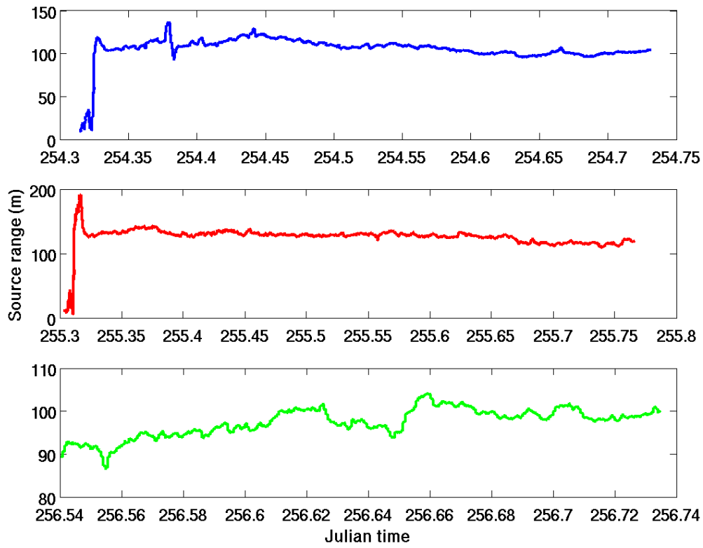
Figure 2.12: AOB22 GPS estimated source range variations along time for days 11, 12 and 23 September, 2007.
