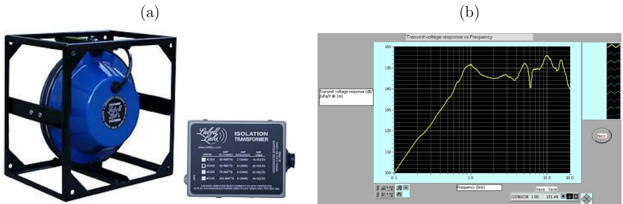
Figure 3.4: Lubell 916C sound source (a) and transmitt voltage response - TVR (b).
