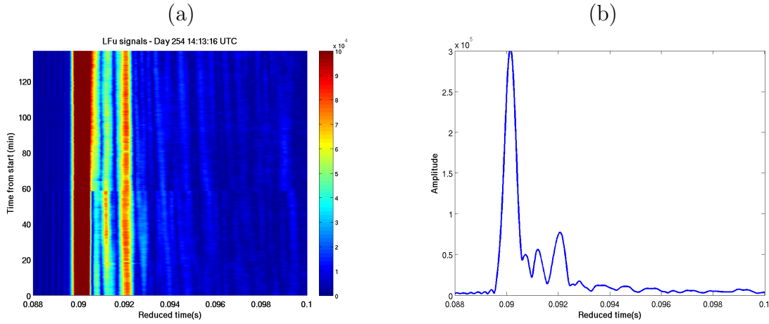
Figure 3.9: Day 254, hydrophone 1 (6.6 m depth): arrival pattern for the 3 kHz band up sweep along time (a) and mean arrival pattern (b).
