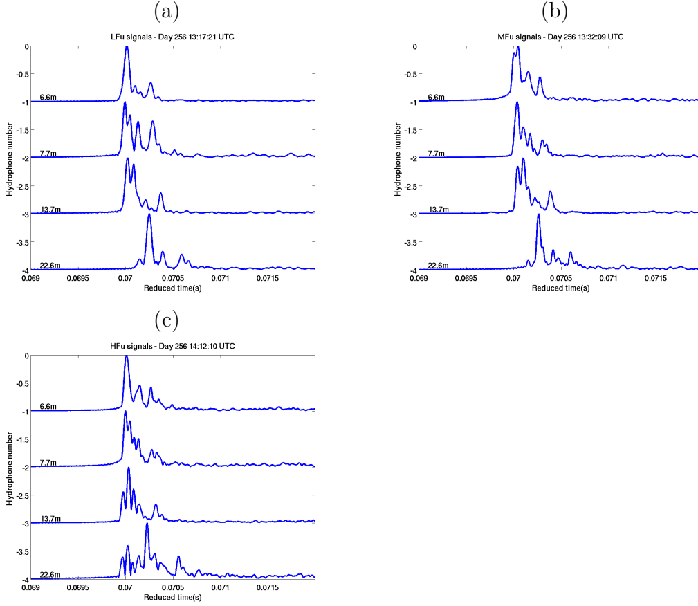
Figure 3.11: Day 256 impulse responses between sound source at 3 m depth ( S_1 ) and each hydrophone for frequency bands : 3500 - 6500 Hz (a), 7500 - 10500 Hz (b) and 12000 - 15500 Hz (c).
