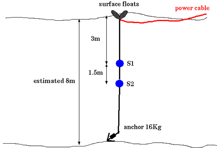
Figure 2.9: sketch of the source array mooring and configuration.
