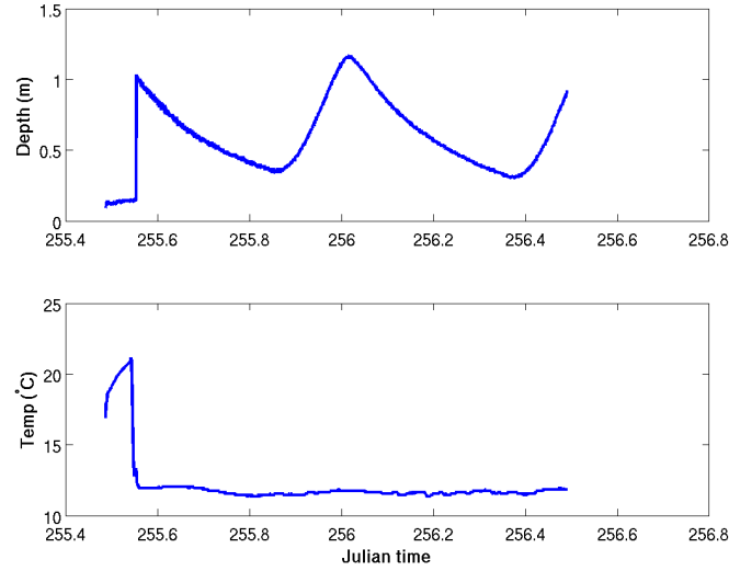
Figure 2.7: Hobo autonomous recording water depth (top) and temperature (bottom), near the pier to infer tidal variation in the bay.
