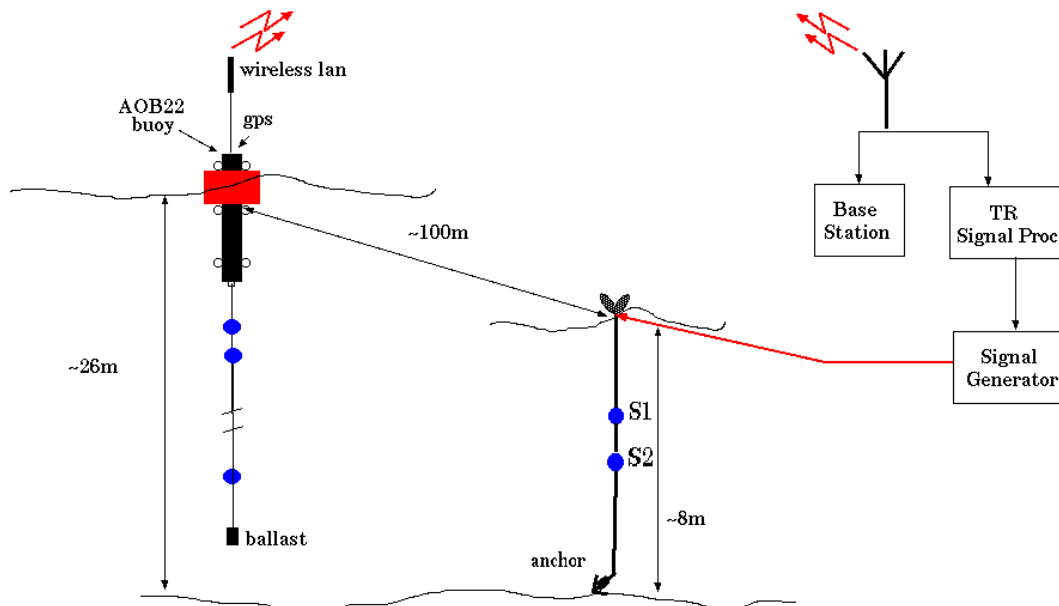
Figure 3.1: experimental setup for signal control and processing during the Hopavågen bay experiment.
