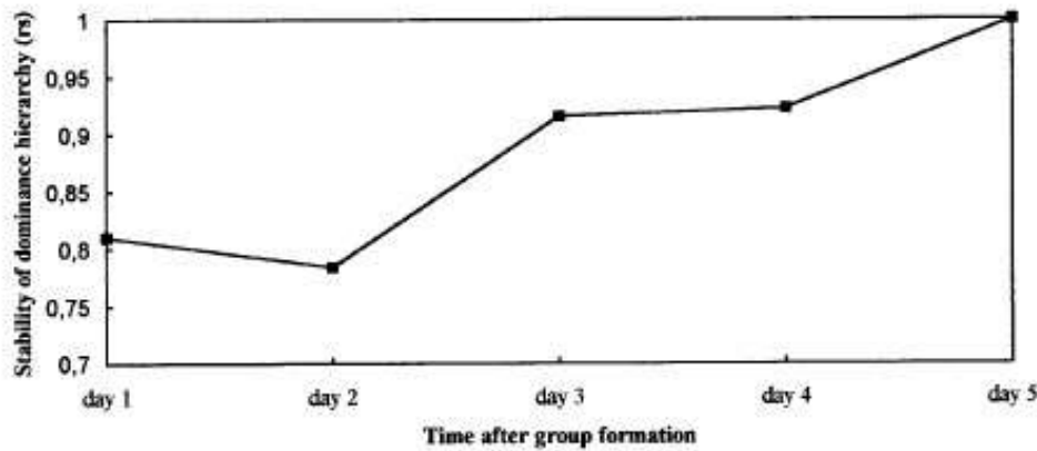
FIG. 1. Correlation coefficients between the dominance index computed daily, from day 1 to day 4, and the same index computed at day 5.
