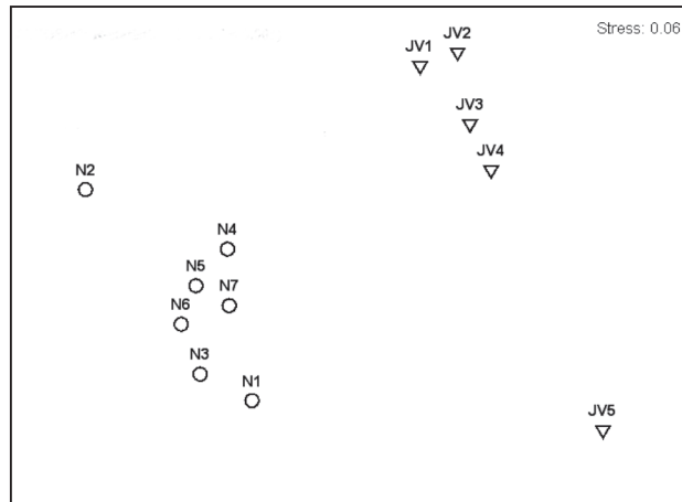
FIG. 2. – Non-metric multi-dimensional scaling ordination plot of the presence/absence data for fish assemblages sampled at Northwest Bank (Nn, ○) and João Valente Bank (JVn, ▽). Stress value for the plot is given in the top right hand corner.
