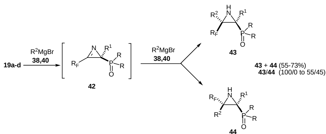
Scheme 12. Generation of 2 H -azirines 42 by Grignard reagents and nucleophilic addition.
