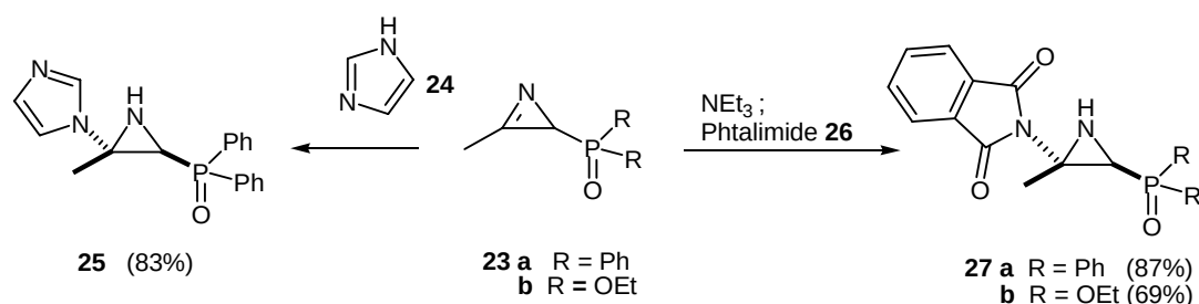
Scheme 8. Imidazole mediated generation of 2 H -azirine 20a and nucleophilic addition.
