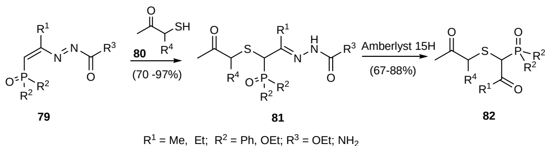
Scheme 22. Addition of 3-mercapto-2-ketones 80 to azoalkenes 79 .
