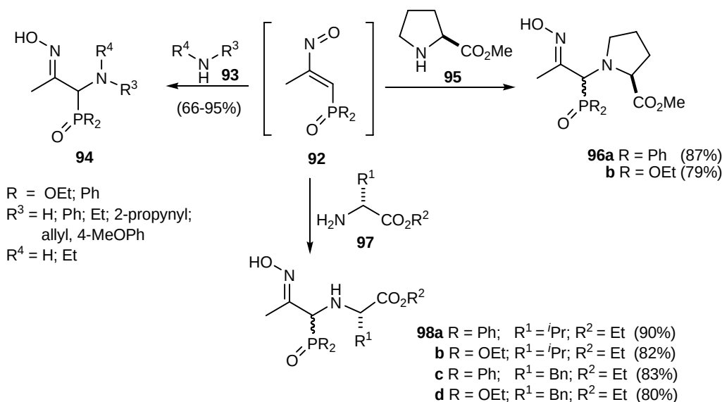
Scheme 25. Nitrosoalkenes 92 as Michael acceptors.
