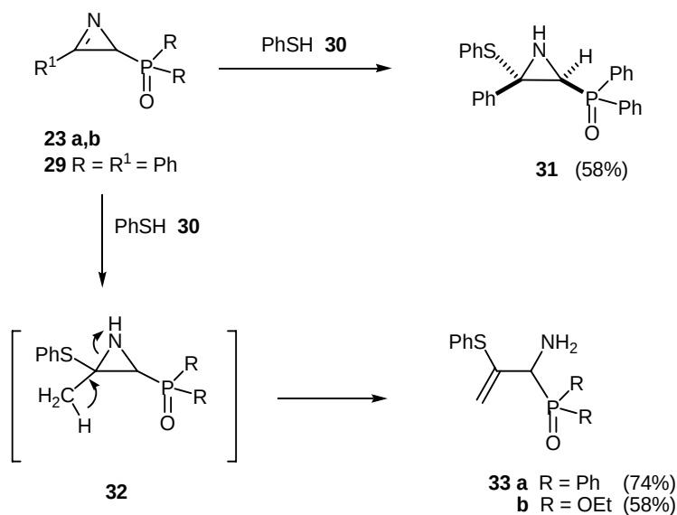
Scheme 10. Benzenethiol addition to 2 H -azirines 23 and 29 .
