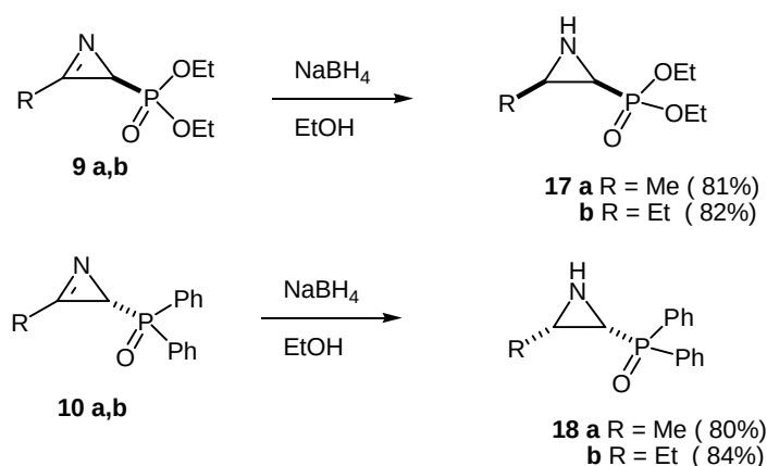
Scheme 5. Hydride addition to 2 H -azirines 9 and 10 .
