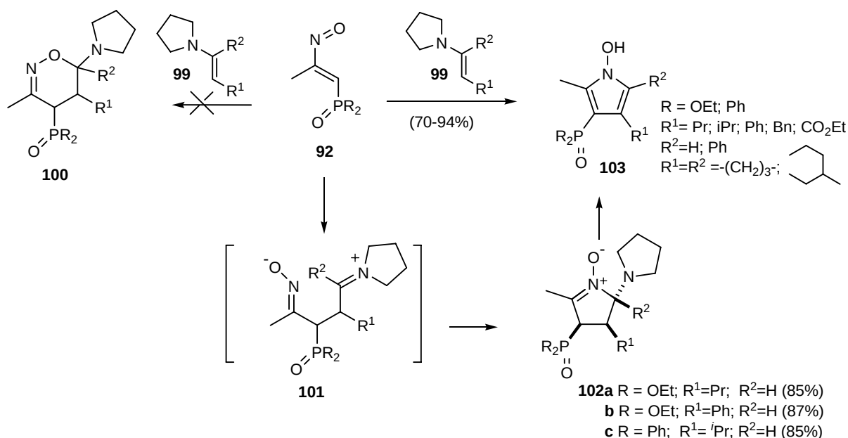
Scheme 26. Reaction of nitrosoalkenes 92 with enamines 99 .
