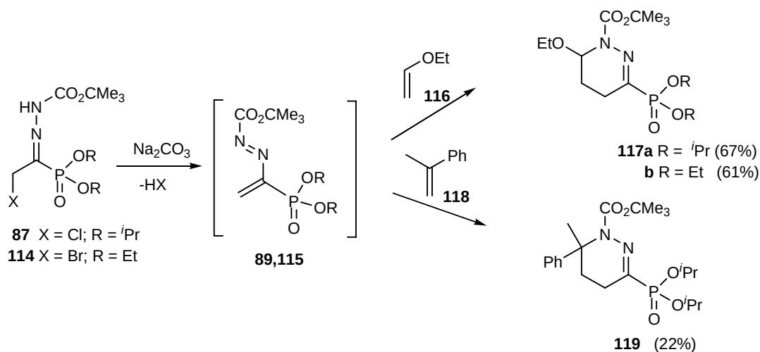
Scheme 28. Cycloaddition reactions of azoalkenes 89 and 115 with electron rich olefins.
