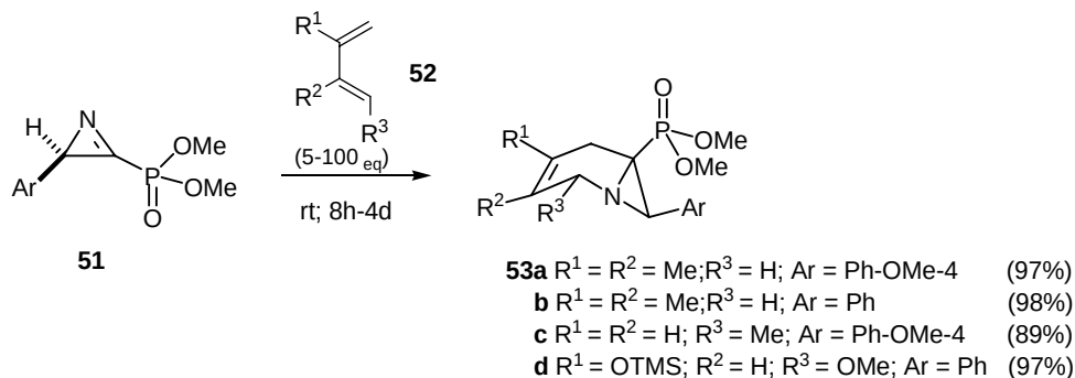
Scheme 15. Cycloaddition reactions of 2 H -azirine 51 .
