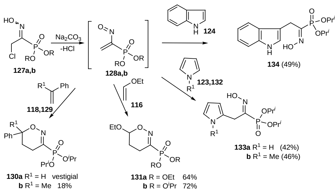
Scheme 29. Cycloaddition reactions of nitrosovinylphosphonates 128 .
