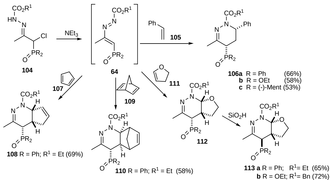
Scheme 27. Cycloaddition reactions of azoalkenes 64 .
