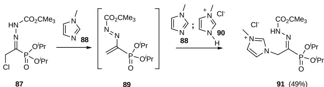
Scheme 24. N -methylimidazole generation of azoalkene 89 and nucleophilic addition.
