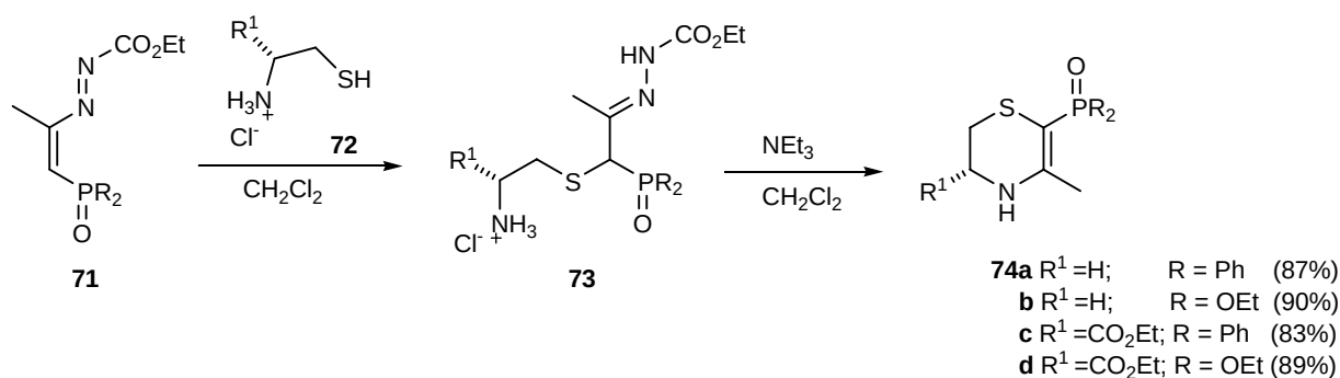
Scheme 20. 1,4-Addition of 1,2-aminothiols 72 to nitrosoalkenes 71 .
