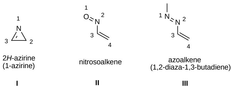
Figure 1. Name, structure and numbering of compounds.
