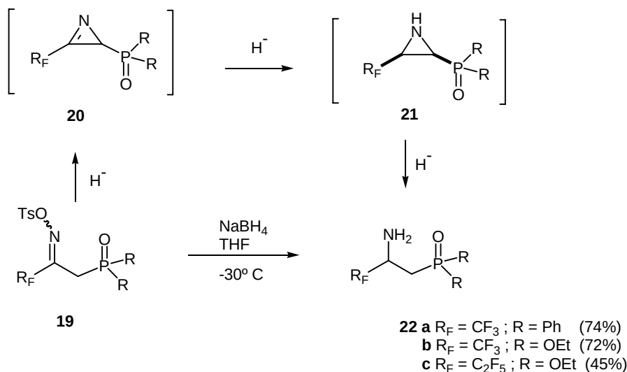
Scheme 6. \beta -Amino-phosphine oxides and -phosphonates 22 from tosyloximes 19 .
