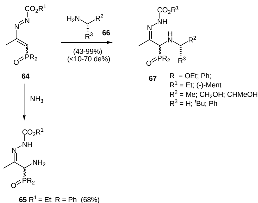
Scheme 18. Nucleophilic addition of ammonia, aminoesters and aminoalcohols to azoalkene 64 .
