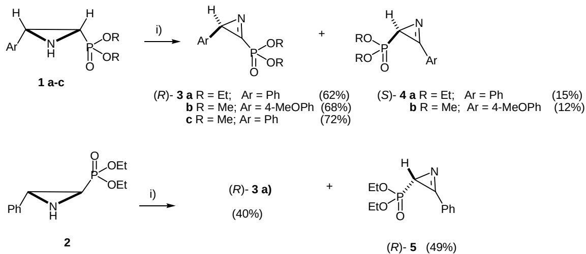
Scheme 1. Synthesis of 2 H -azirines by Swern oxidation.
