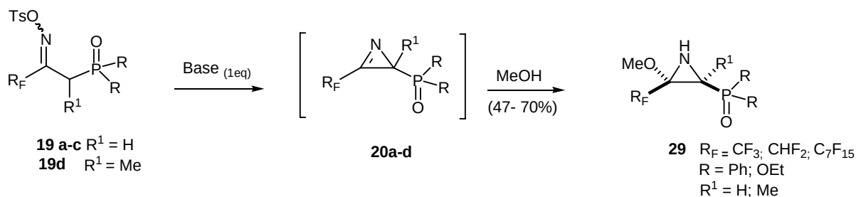
Scheme 10. Benzenethiol addition to 2 H -azirines 23 and 29 .
