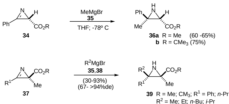
Scheme 11. Addition of Grignard reagents to 2 H -azirine-2-carboxylates.
