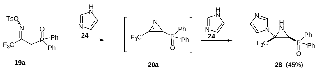
Scheme 8. Imidazole mediated generation of 2 H -azirine 20a and nucleophilic addition.
