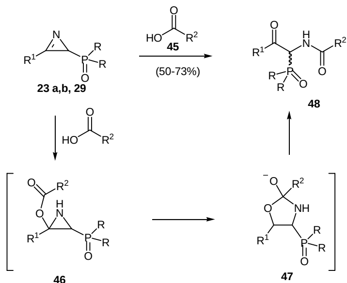
Scheme 13. Ketamides 48 from 2 H -azirines 23 and 29 .
