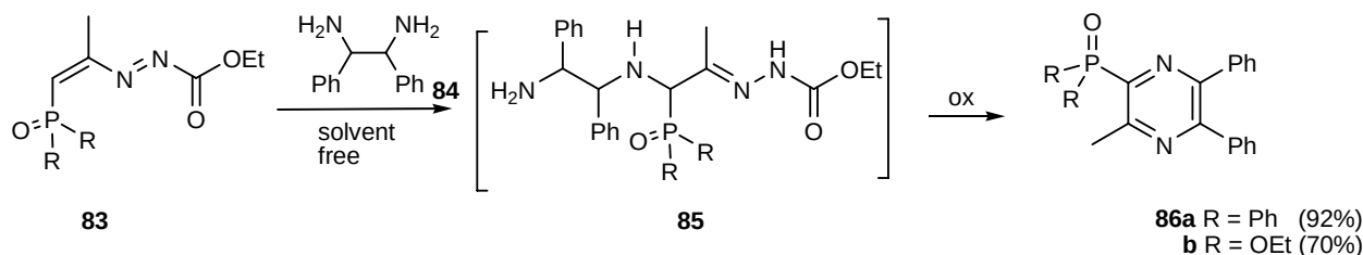
Scheme 23. Addition of 1,2-diamines to phosphinyl- and phosphonyl-azoalkenes 83 .
