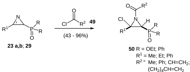
Scheme 14. Reactions of acyl chlorides with phosphinyl- and phosphonyl-2 H -azirines.
