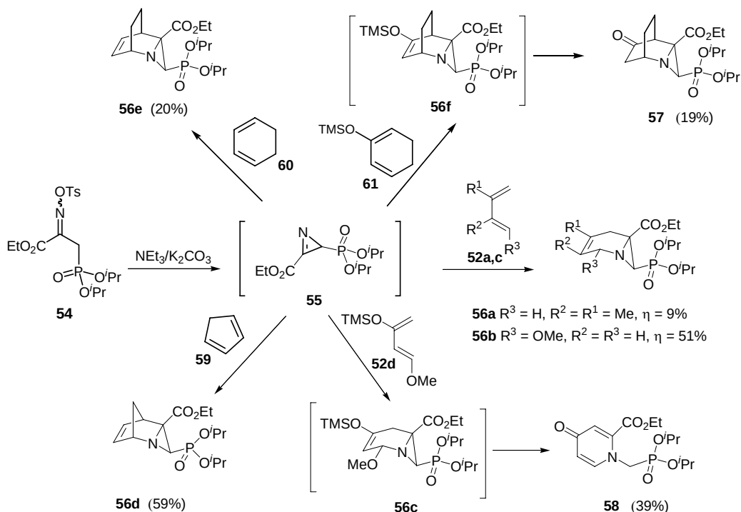
Scheme 16. Cycloaddition reactions of 2 H -azirine 55 with nucleophilic dienes.
