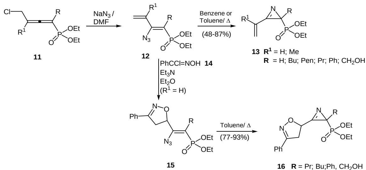
Scheme 4. Synthesis of 3-vinyl- and 3-dihydroisoxazolyl-2 H -azirines.
