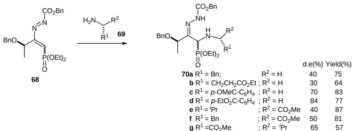
Scheme 19. Addition of amino esters to optically active azoalkene 68 .
