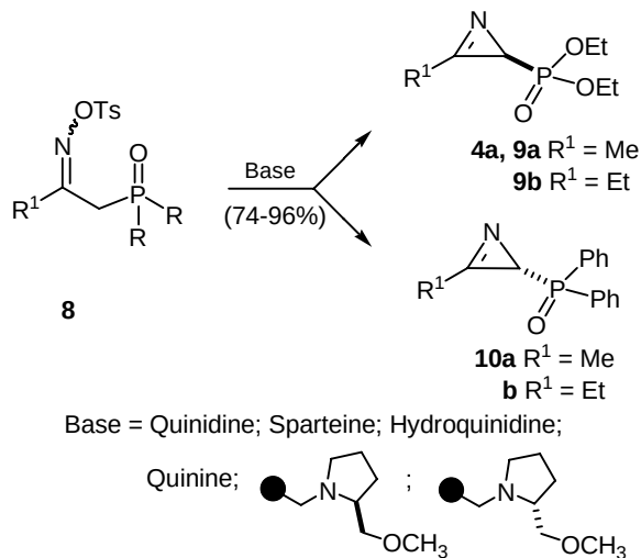
Scheme 3. 2 H -Azirines by Neber reactions of β-keto tosyloximes.
