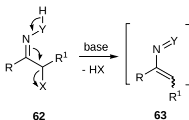
Scheme 17. General method for the obtention of nitroso- and azo-alkenes.
