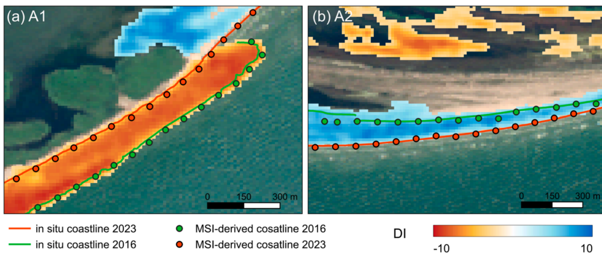
Fig. 6. Comparison of change area detected from SAR images with in situ -measured coastlines at Sahalin Spit in the Danube Delta. (a) Erosion case in A1, and (b) accretion case in A2. A1 and A2 are the same locations as in Fig. 4. Background is from the Sentinel-2 MSI true colour image on 5 August 2023. Colour of the pixel represents the difference intensity (DI) from SAR images, where blue indicates accretion and red is erosion. (For interpretation of the references to colour in this figure legend, the reader is referred to the web version of this article.)
