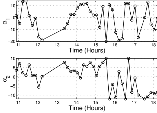
Figure 6. EOF coefficient estimates obtained by inversion of the acoustic data collected with AOB1.
