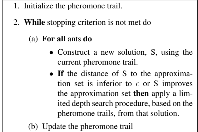
Figure 1. \epsilon -DANTE Algorithm
