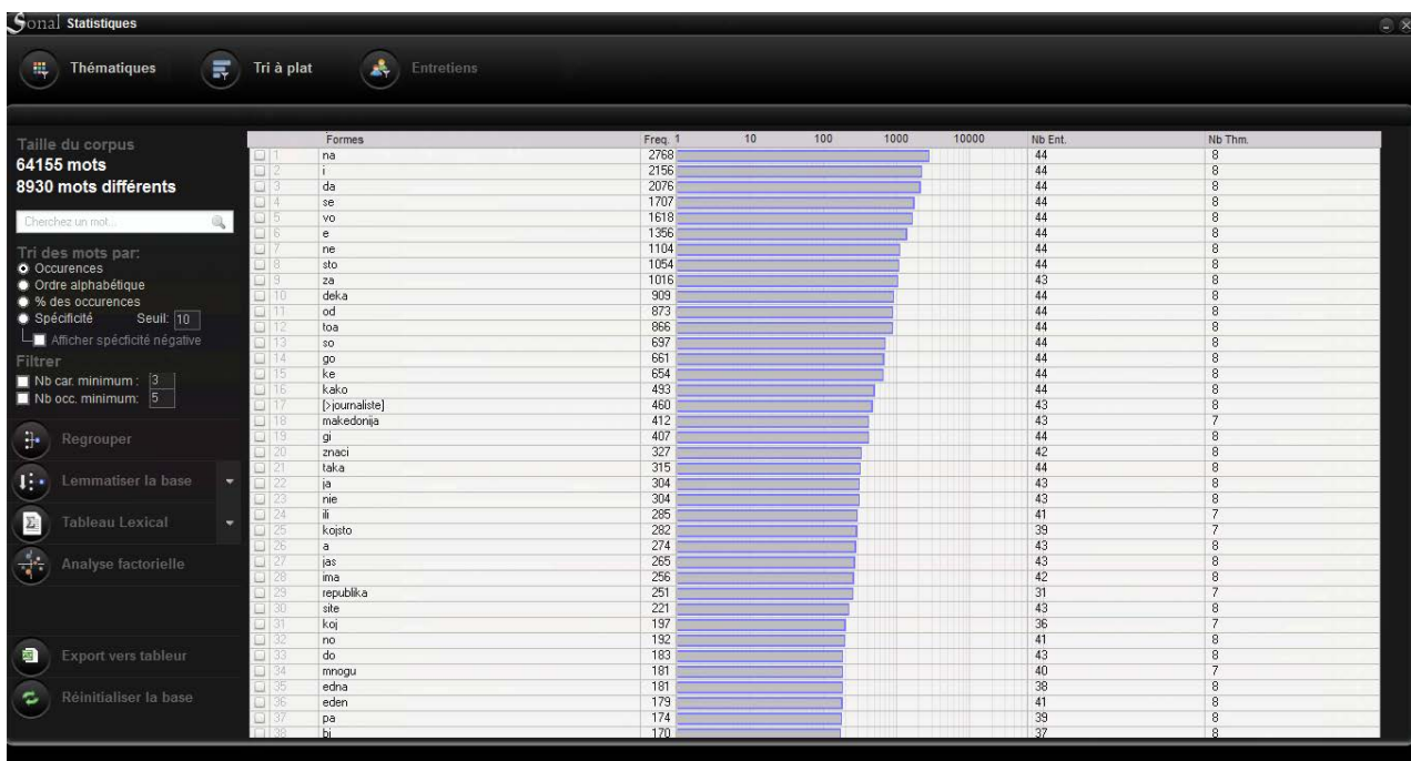
FIGURE 7: WORD COUNT
