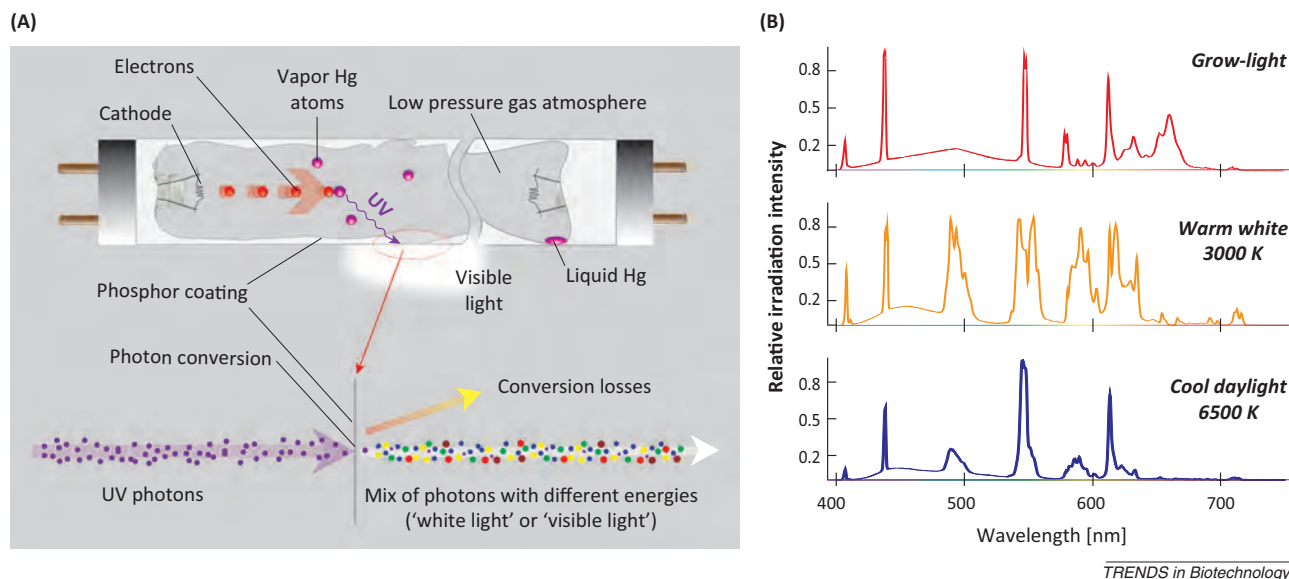
Figure 1. (A) Simplified diagram showing how fluorescent lamps (FLs) work. (B) Emission spectra for different FL types, including grow-lights, warm white FL, and cold daylight FLs.
