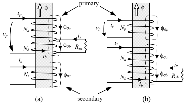
Fig. 3: Equivalent circuits for a fault occurring in the: (a) primary winding; (b) secondary winding.
