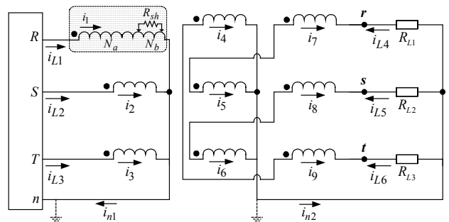
Fig. 5: Equivalent electric circuit for the case of a primary-side faulty winding (phase R).
