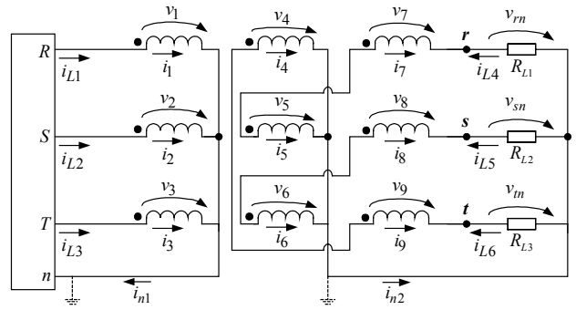
Fig. 2: Simplified equivalent electric circuit for the case of an Yzn5 connection and a balanced resistive load.
