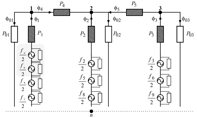
Fig. 4: Equivalent magnetic circuit for the case of a primary-side faulty winding (phase R).
