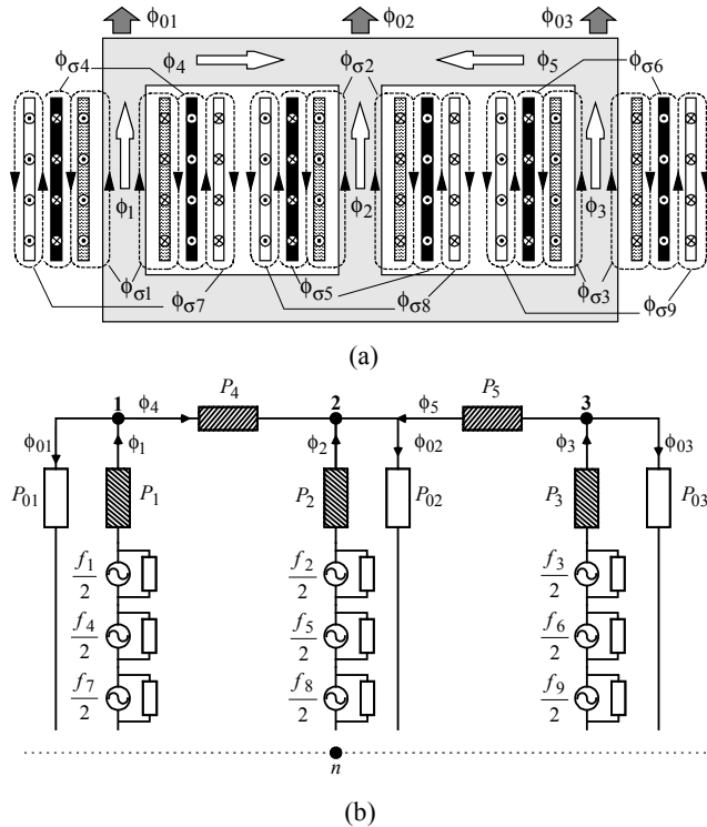
Fig. 1: (a) Flux distribution in a three-phase, three-limb, three-winding, core-type transformer, assuming a slightly greater magnetomotive force in the inner windings; (b) equivalent magnetic circuit.
