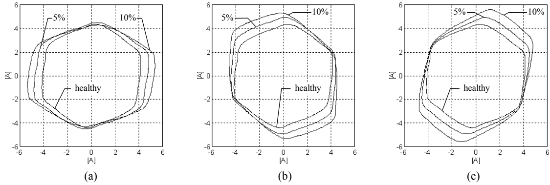
Fig. 9: Experimental primary-side phase current Park's Vector patterns for the case of a Yzn5 connection and a balanced resistive load, with several percentages of permanent shorted turns in the primary windings and for different faulty phases: (a) phase R ; (b) phase S ; (c) phase T .
