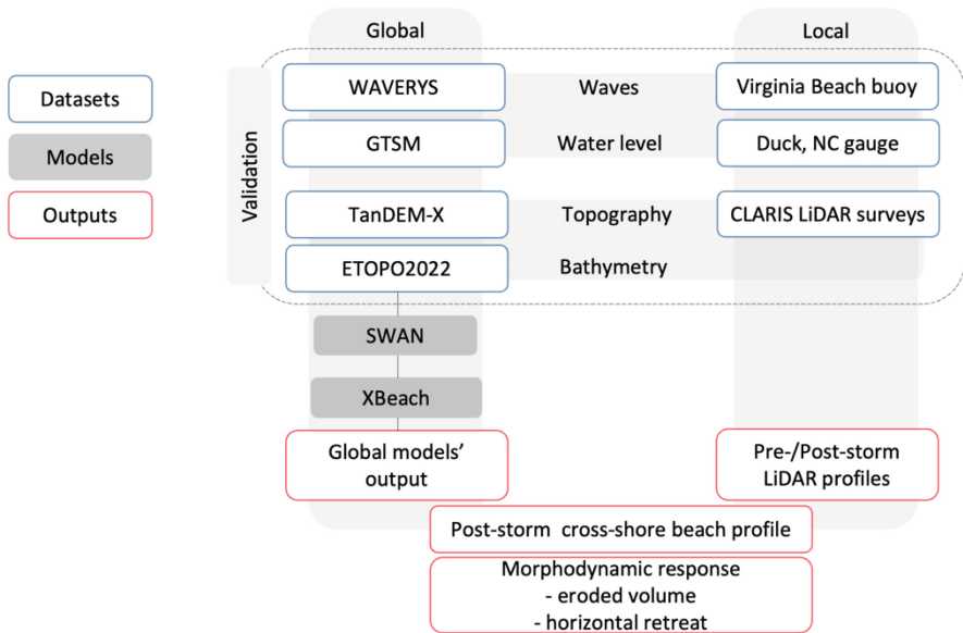
Fig. 1. Schematic representation of the methodology applied to the barrier island of Duck in North Carolina for validation of a storm impact assessment performed with global models.
