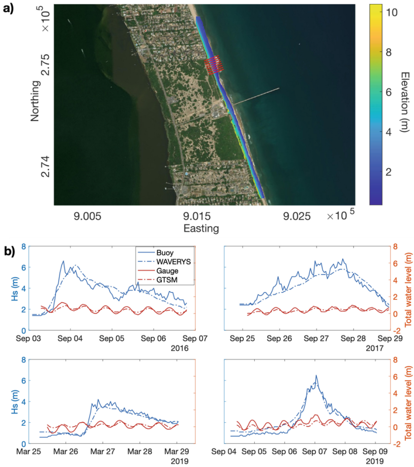
Fig. 2. a) ESRI Satellite aerial image of the barrier at Duck, North Carolina with CLARIS survey (22 September 2017) and cross-shore sampled profiles. b) Examples of storm significant wave height (blue) from Virginia buoy and WAVERYS as input for SWAN and total water level (red) from Duck tide gauge and GTSM as input for XBeach.
