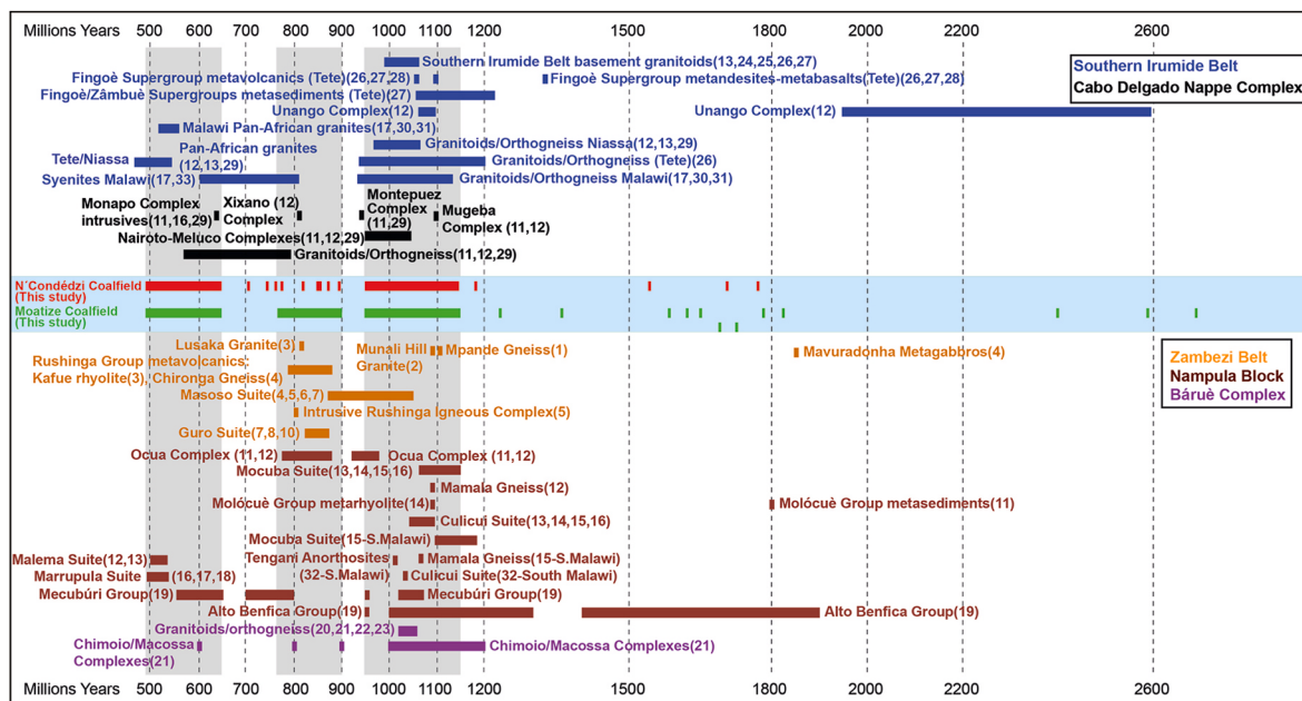
Fig. 8. Major tectonomagmatic events and zircon ages of the several geologic units in the Southern Irumide Belt, Cabo Delgado Nappe Complex, Zambezi Belt, Nampula Block and Bárué Complex. The vertical pale-grey bars indicate 650–490 Ma, 900–780 Ma and 1150–950 Ma time windows. Data sources are: (1) Hanson et al. (1988) , (2) Katongo et al. (2004) , (3) Johnson et al. (2007) , (4) Hargrove et al. (2003) , (5) Sakuwaha et al. (2022) , (6) Mariga et al. (1998) , (7) Vinyu et al. (1999) , (8) GTK-Consortium, 2006 , (9) Mántari (2008) , (10) Manjate and Tassinari (2018) , (11) Jamal (2005) , (12) Norconsult-Consortium (2007) , (13) Bingen et al. (2009) , (14) Macey et al. (2010) , (15) Kröner et al. (1997) , (16) Macey et al. (2007) , (17) Thomas et al. (2022) , (18) Grantham et al. (2007) , (19) Grantham et al. (2008) , (20) Jacobs et al. (2008) , (21) Thomas et al. (2010) , (22) Cháuque (2012) , (23) Cháuque et al. (2019) , (24) Manjate (2012) , (25) Manjate (2015) , (26) Westerhof et al. (2008) , (27) Petry et al. (2022) , (28) Kröner et al. (2001) , (29) Manda et al. (2019) , (30) Tsunogae et al. (2021) , (31) Ashwal et al. (2007) , (32) Thomas et al. (2022) .
