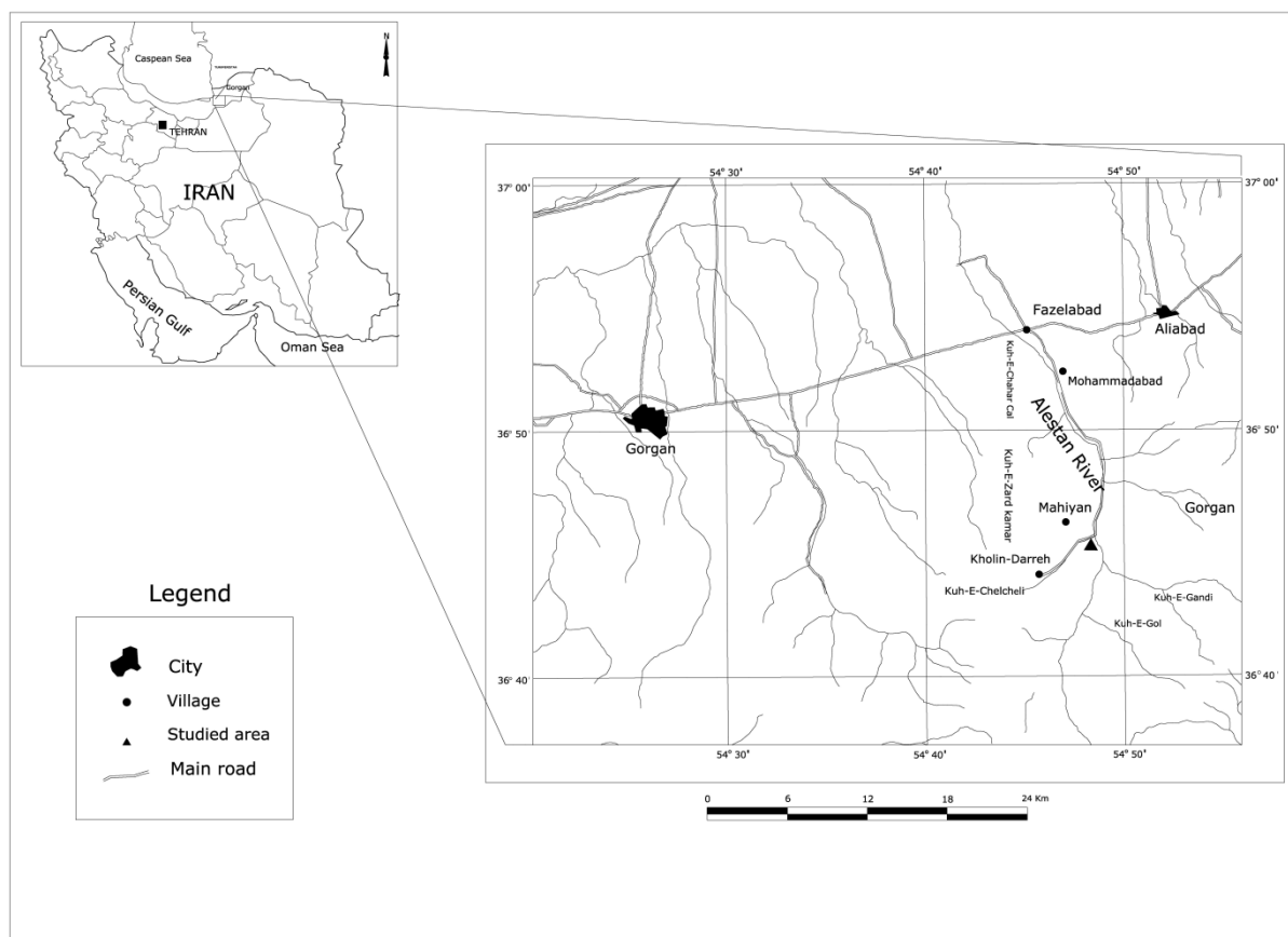
Figure 1. Location of the studied area.
