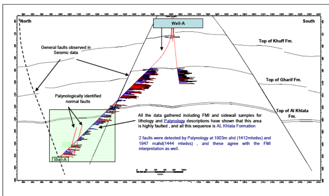
Figure 3. A simple cartoon illustrates where is the unknown lithologies encountered along the well path. This resulted in gathering sidwall samples in this section (with shaded square) for palynology study.
