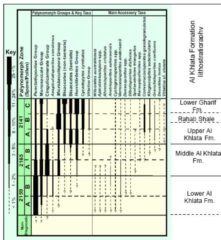
Figure 2. Modified from Penney et al. (2008) Al Khlata Formation Biozonation scheme. (Fm. = Formation; Mmb. = Member).
