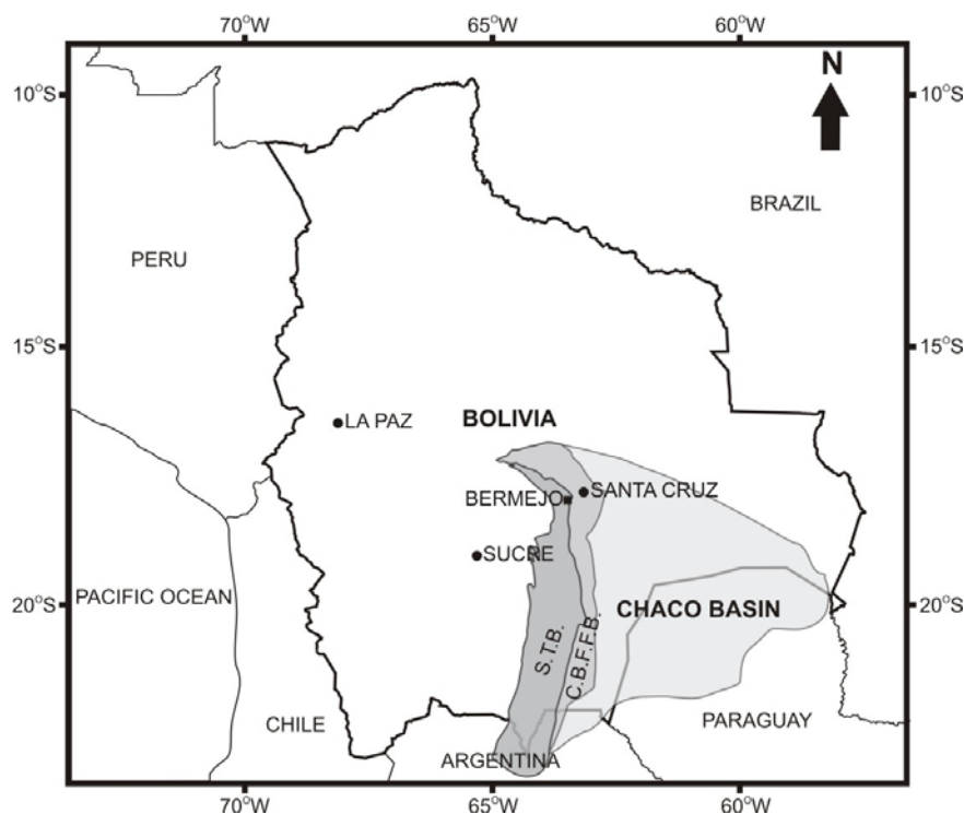
Figure 1. Outline map of Bolivia showing the sampled Devonian locality at Bermejo. Major cities are shown as black circles. Superimposed is the Chaco Basin, which is subdivided into the Subandean Thrust Belt and the Chaco Basin Foreland Fold Belt.
