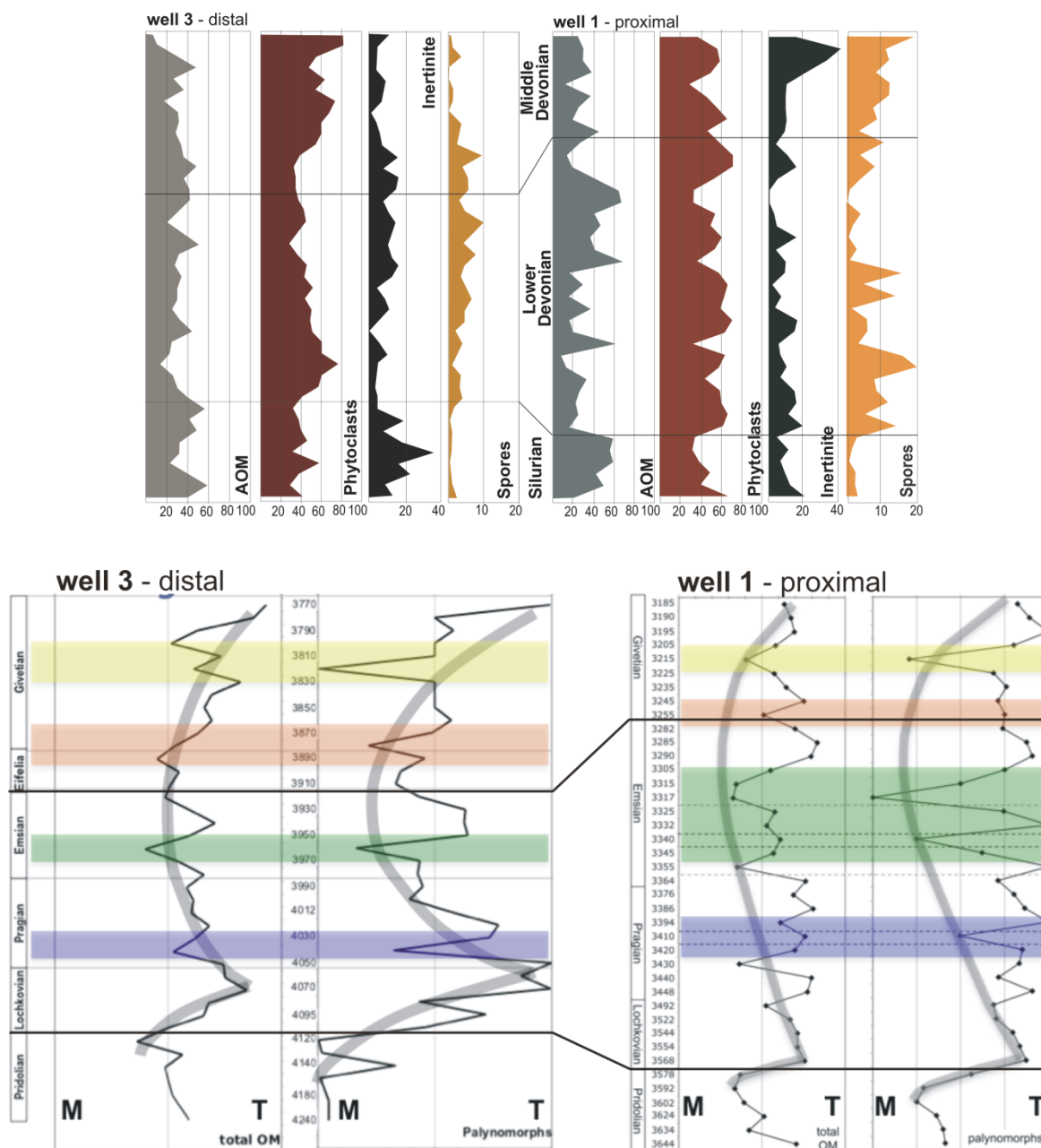
Figure 2. Palynofacies trends of main groups in high resolution studied wells 1 and 3.
