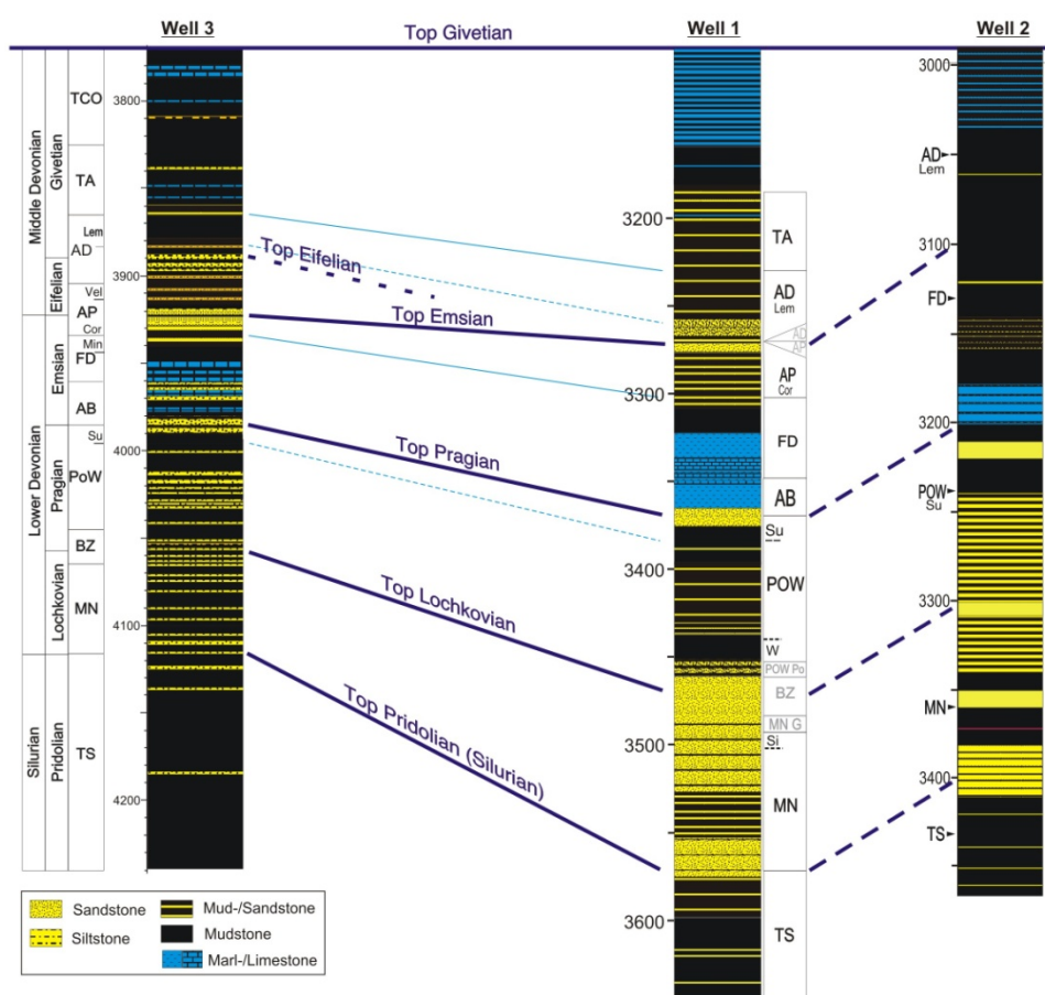
Figure 1. Palynostratigraphic correlation of three wells studied in the Reggane basin.
