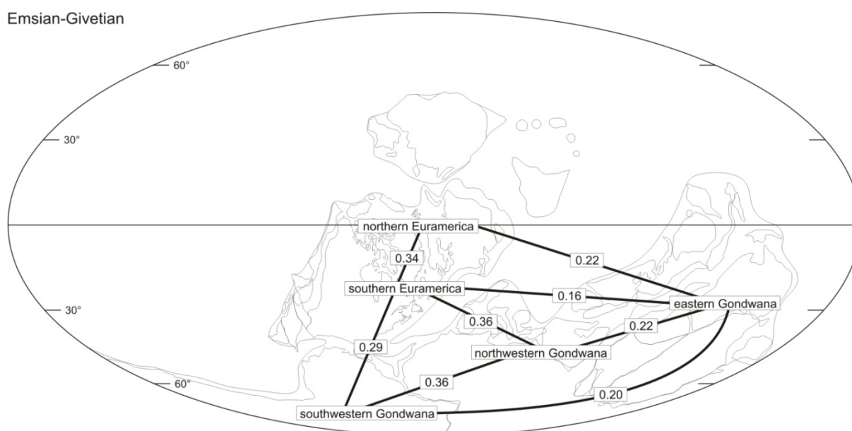
Figure 1. Coefficients of similarity between the different regions calculated on the basis of Emsian-Givetian miospore assemblages. Palaeogeographic reconstruction modified after Scotese (2000).
