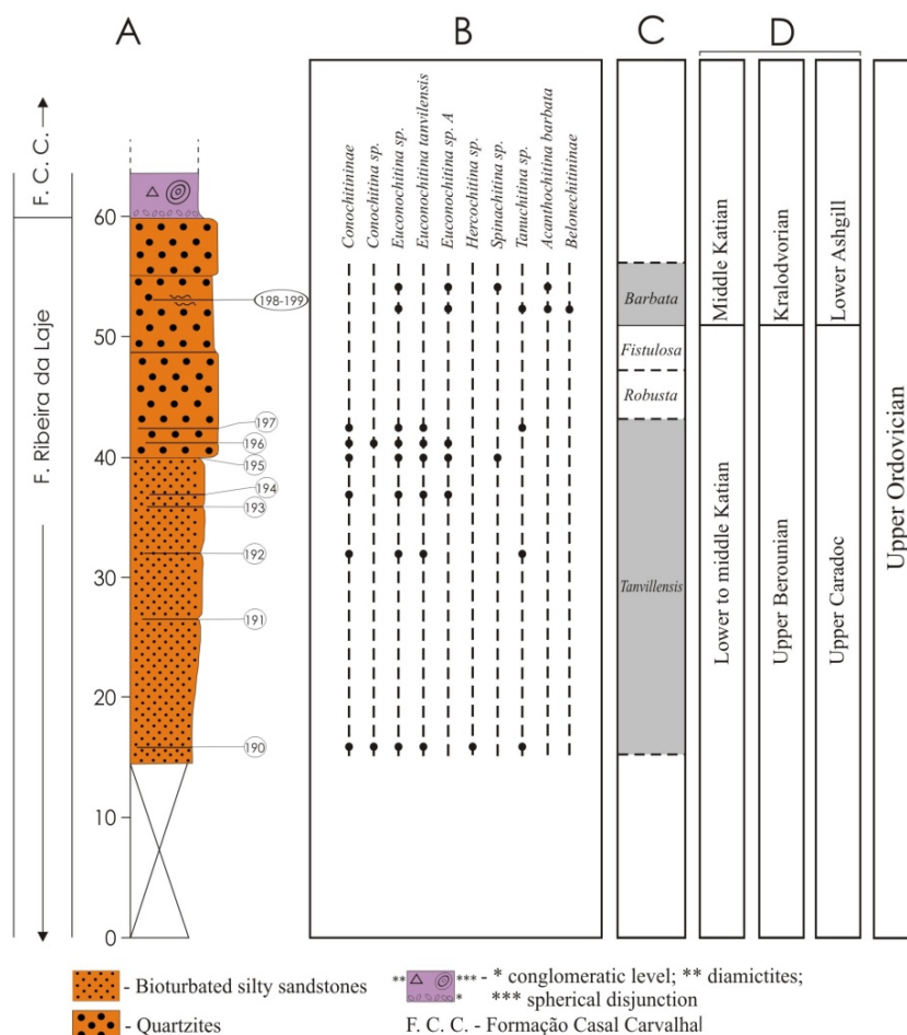
Figure 2. A. Stratigraphic log of the Ribeira da Laje Formation with the location of the studied samples (scale in meters). B. Palinostratigraphical results. C. Biozonation adapted for the North Gondwana domain (Paris, 1990, 1999; Paris and Verniers, 2005). D. Chronostratigraphic chart for the Upper Ordovician (Global Ordovician Stages, Mediterranean and North Gondwana Ordovician Stages and United Kingdom Ordovician Series (Bergström et al., 2009).
