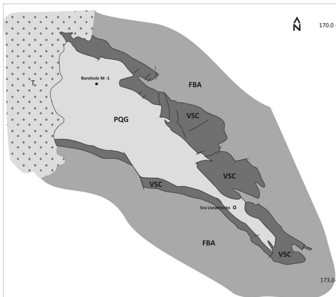
Figure 1. Simplified geology of the S. Francisco da Serra Anticline (adap. Alves et al., 1985). FBA - Mértola Formation (Flysch); VSC - Volcano-Sedimentary Complex; PQG - Phyllite-Quartzite Group; Tertiary sediments.
