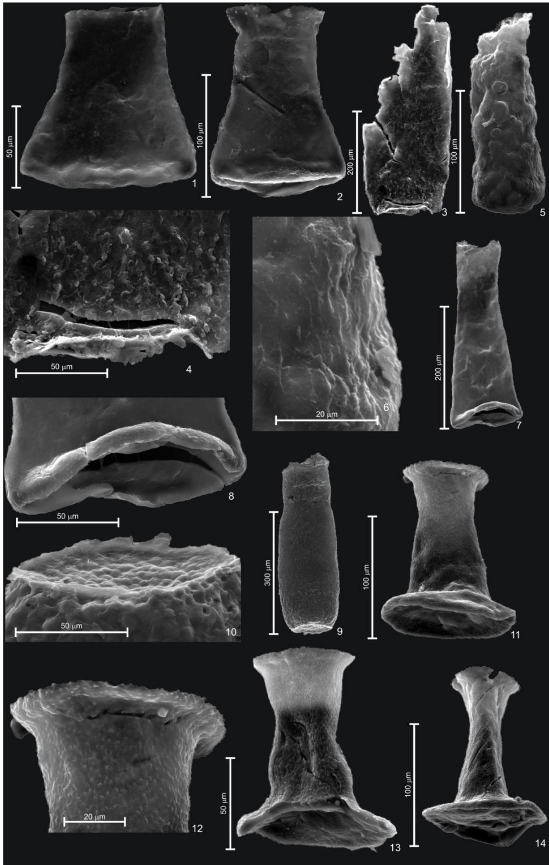
Figure 3. 1, 2. Euconochitina tanvillensis Paris in Robardet et al., 1972. 3, 4. Acanthochitina barbata Eisenack 1931. 5, 6. Hercochitina sp. 7, 8. Spinachitina sp. 9, 10. Tanuchitina sp. 11, 14. Euconochitina sp. A.
