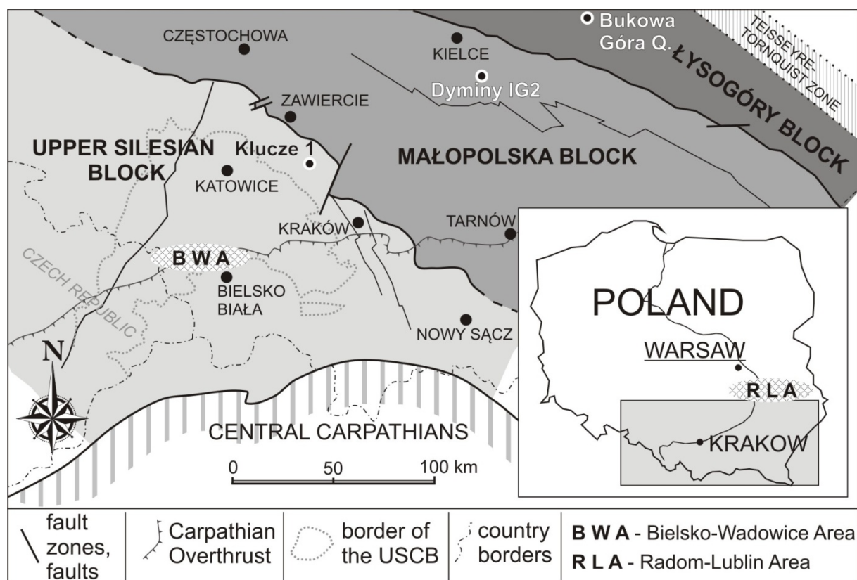
Figure 1. Localization of the investigated boreholes and previously investigated areas.
