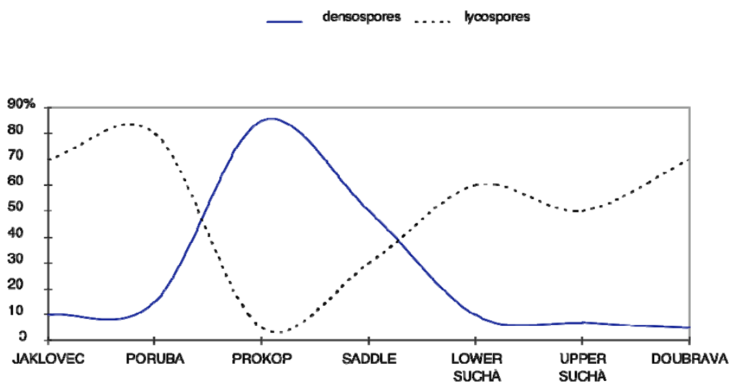
Figure 1. Percentage of two main spore groups in dispersed spore assemblages of the Czech part of the Upper Silesian Basin, Czech Republic (dash line represents lycospores and continuous line densospores with the maximum within the Prokop Seam).
