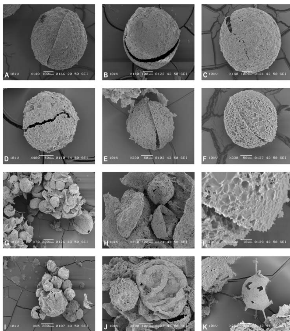
Figure 2. Palynomorphs of the Chotec Limestone. All specimens are from the prasinophyte horizon. A-J: Tasmanites/Leiosphaeridia ; K: Mazuelloid.
