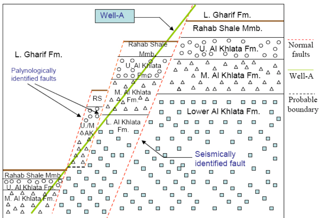
Figure 5. A schematic diagram of structural details of the shaded square in Fig 3. Note the difference of the of the Al Khlata Fm. Picked by poor seismic in Fig 3. and by palynology on this figure. Figures not to scale. (U=Upper; M=Middle; L=lower; AK=Al Khlata Formation; RS=Rahab Shale; Mmb=Member; Fm=Formation).
