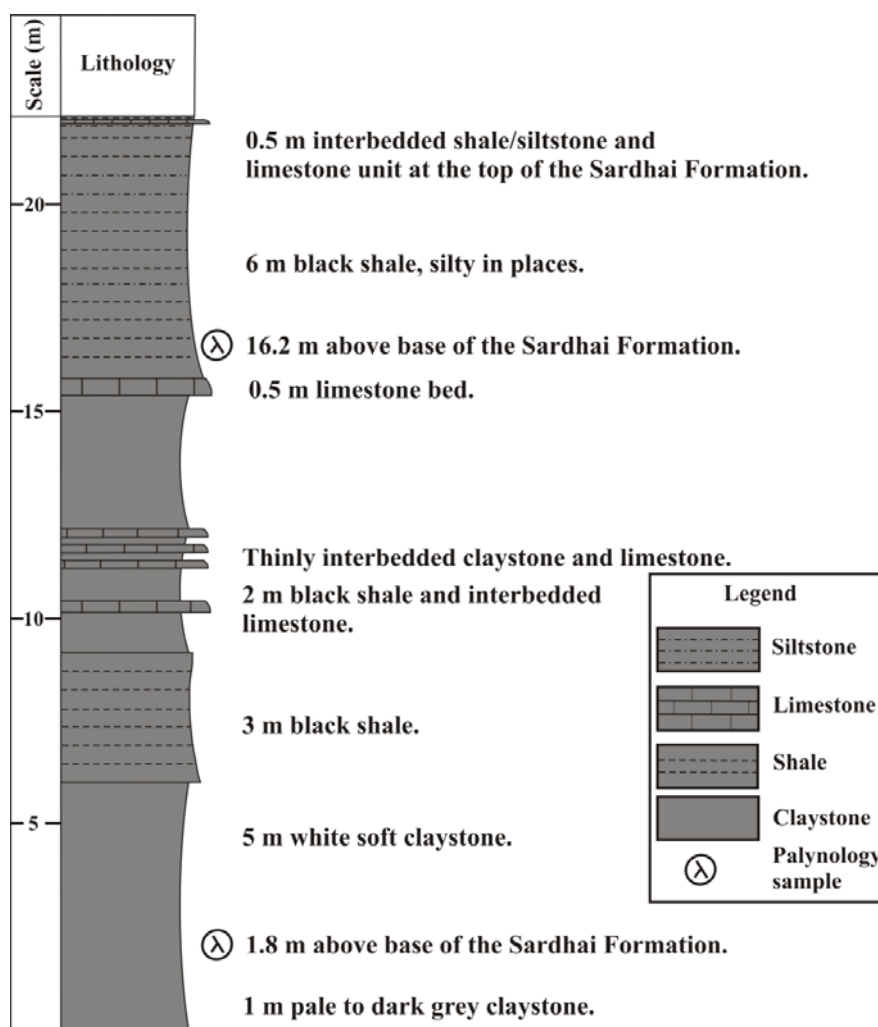
Figure 2. Measured section of the Sardhai Formation in the Khisor Range Pakistan.
