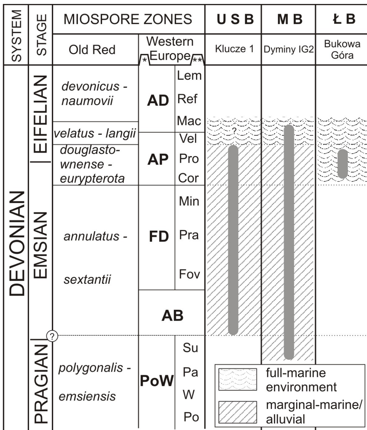
Figure 2. Palynostratigraphy and palynofacies of the investigated boreholes. *Oppel Zones; **Interval Zones ( sensu Streel et al., 1987).
