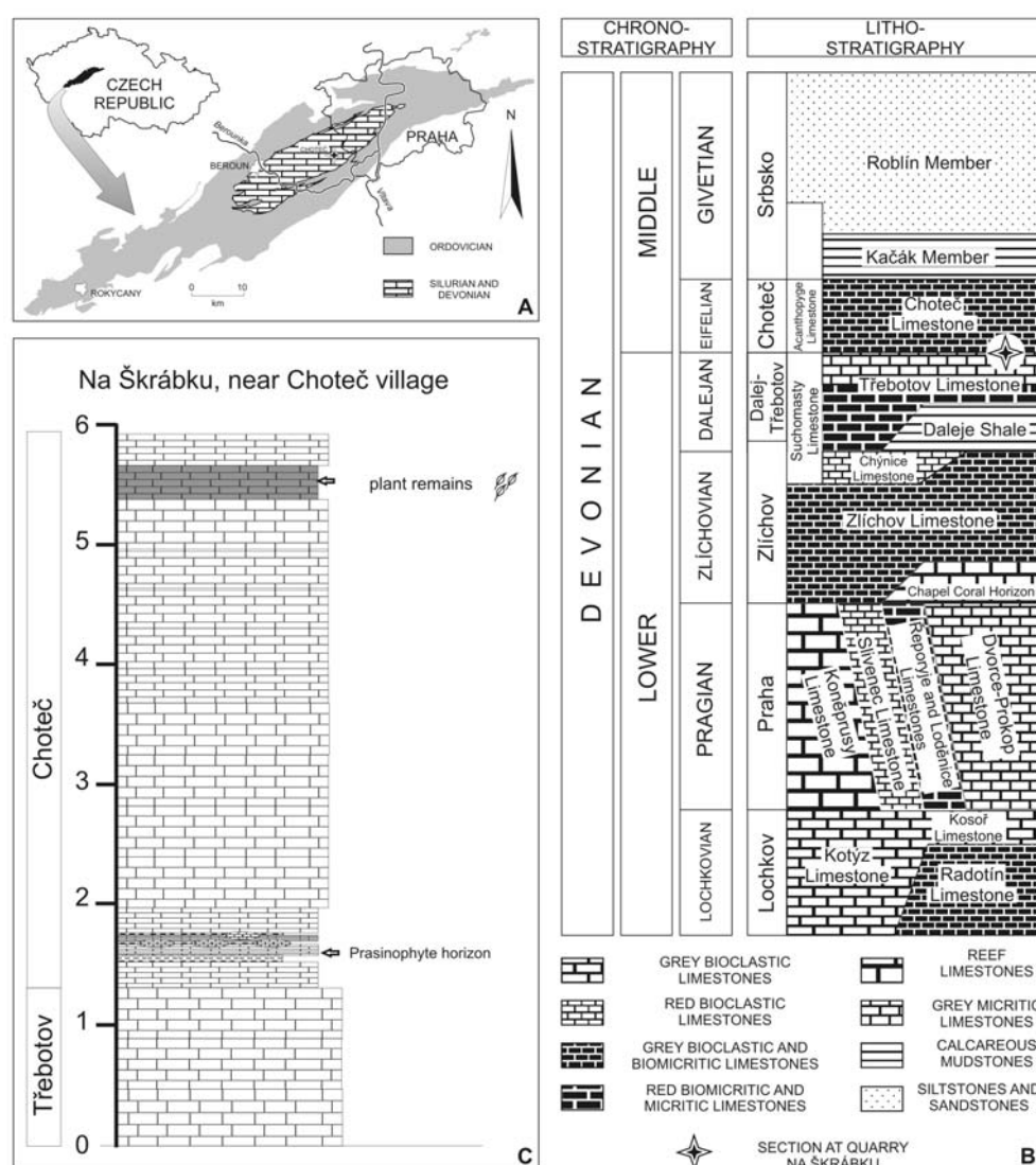
Figure 1. A: Simplified geological sketch map of the Prague Basin (Barrandian area) and the studied section in the Na Škrábku quarry near Chotec; B: Devonian stratigraphy of the Barrandian area (after Chlupáč et al., 1998); C: Stratigraphic section in the Na Škrábku quarry near Chotec.
