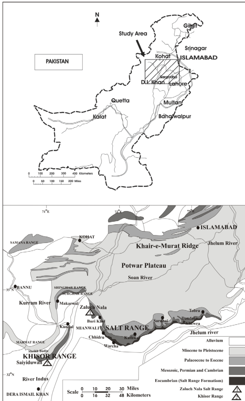
Figure 1. Location map of the study area. Showing Salt and Khisor ranges of Pakistan (Modified after Gee 1980, 1989).
