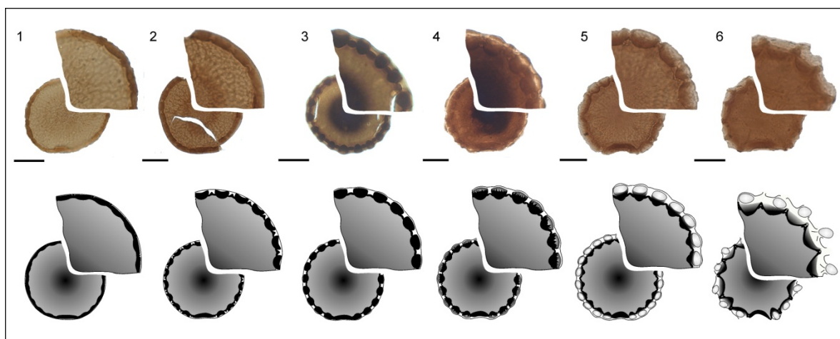
Plate 1. Photomicrographs and schematic diagrams of the six inferred growth stages of Maranhites mosesii (Sommer) Brito, 1967 emend. González 2009. Scale bar = 20 \mu m.
