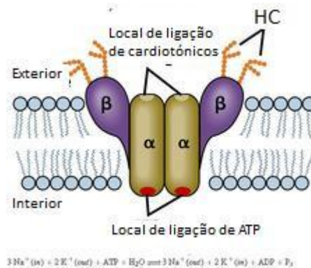
Figura 4.3: Heterodímeros da ATPase (adaptado de http://quizlet.com/15379006/membrane-transport-2-flash-cards/ )
