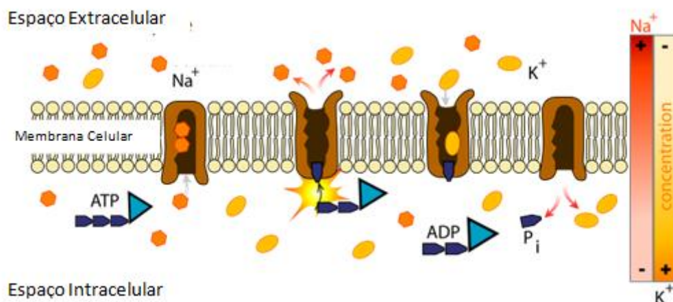
Figura 4.2: ATPase \text{Na}^+/\text{K}^+
