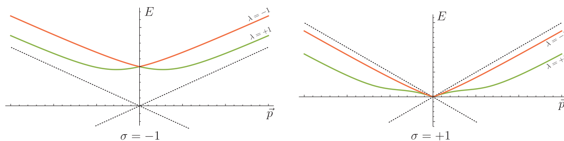
Figure 1. Plots of sample solutions to the \lambda = \pm dispersion relations for the Z boson (left) and photon (right). The size of the Lorentz-violating effects has been exaggerated for illustrational purposes.
