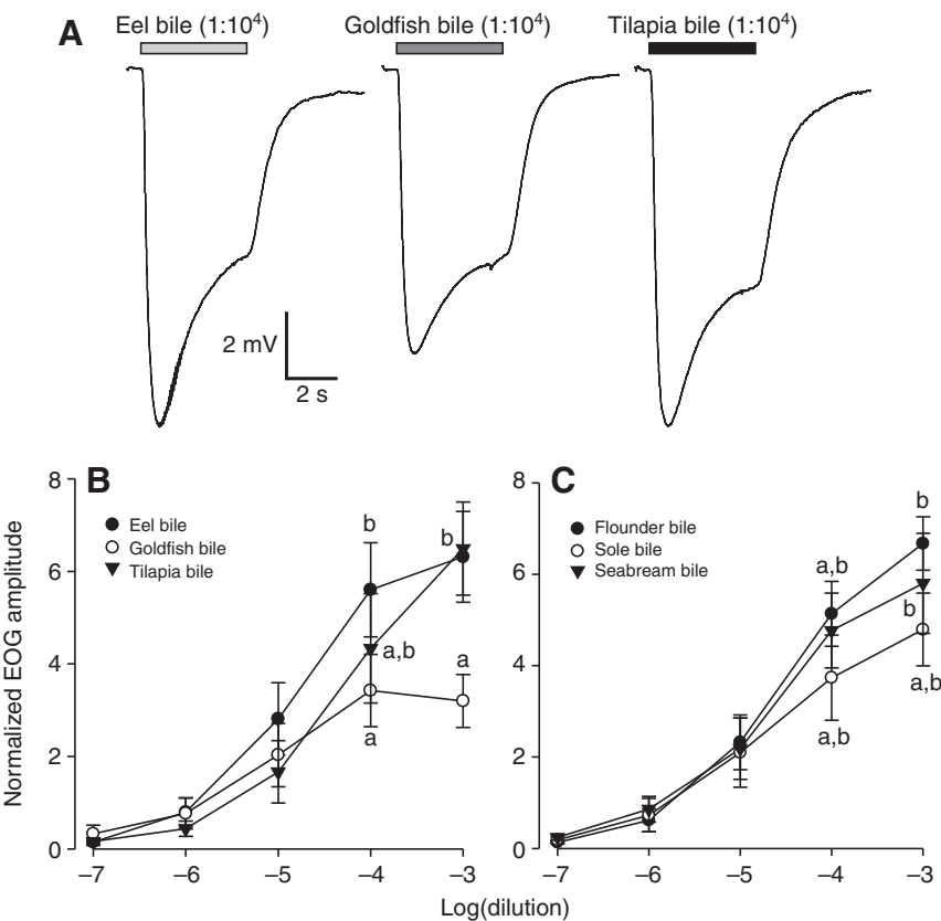
Fig. 3. Olfactory sensitivity to conspecific and heterospecific bile fluid in the tilapia. (A) Typical electro-olfactogram (EOG) traces recorded from a tilapia in response to bile fluid from eels, goldfish and tilapia (all diluted 1:10,000). A downward deflection of the trace is negative. Note the slight 'ringing' (high frequency oscillations) at the peak of the first trace; a common characteristic when recording large EOG responses (Suzuki et al., 2004). (B) Semi-logarithmic plot of pooled normalized EOG amplitudes recorded in tilapia in response to dilution of bile fluid from eels, goldfish and tilapia. (C) Semi-logarithmic plot of pooled normalized EOG amplitudes recorded in tilapia in response to dilution of bile fluid from flounder, sole and seabream. Data are mean \pm s.e.m. ( N=6 ). Values with different letters indicate significantly different response amplitudes to bile fluid (at the same dilution) among all six different types (ANOVA, P<0.05 ).
