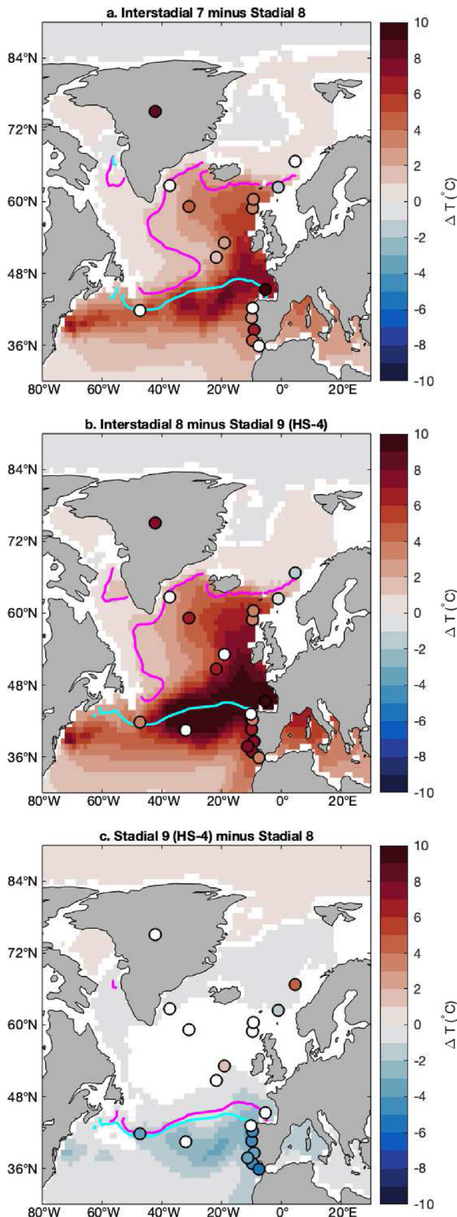
Fig. 5. Mapping the summer 10-m temperature differences between climate states in the D-O events in proxy data (points) and in the model (shading). a) Interstadial warming following a non-Heinrich stadial. b) Interstadial warming following a Heinrich stadial. c) The additional cooling in a Heinrich stadial compared to a non-Heinrich stadial. In each map, violet and cyan lines mark the model mean summer sea ice extent (15% contour) for the warmer and cooler states respectively. . Proxy data are only plotted where there are two or more data points per interval at the core site. Data and model anomalies that are not significant (according to a two-sided Student's t-test at the p < 0.05 level) are filled/shaded white. In calculating the temperature means at each site over the stadials and interstadials, we leave out the first and last 200 years of each interval to reduce sensitivity to dating uncertainty (changing the buffer between 0 and 500 years has little effect on the key patterns, though it does cause the significance of some anomalies to drop from the 95%–90% level). Although proxy data are nominally calibrated to 10-m water depth, the reconstructed temperatures may be representative of greater depths in some locations (see discussion of Nordic Seas sites in the main text). (For interpretation of the references to colour in this figure legend, the reader is referred to the Web version of this article.)
