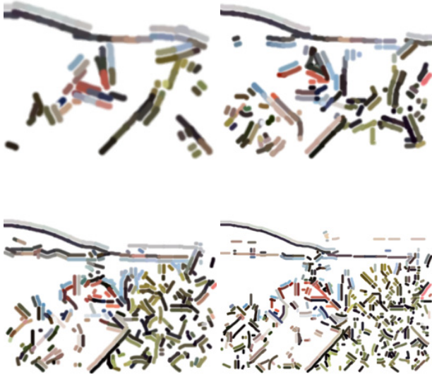
Figure 10. Discrete strokes at the four scales.
