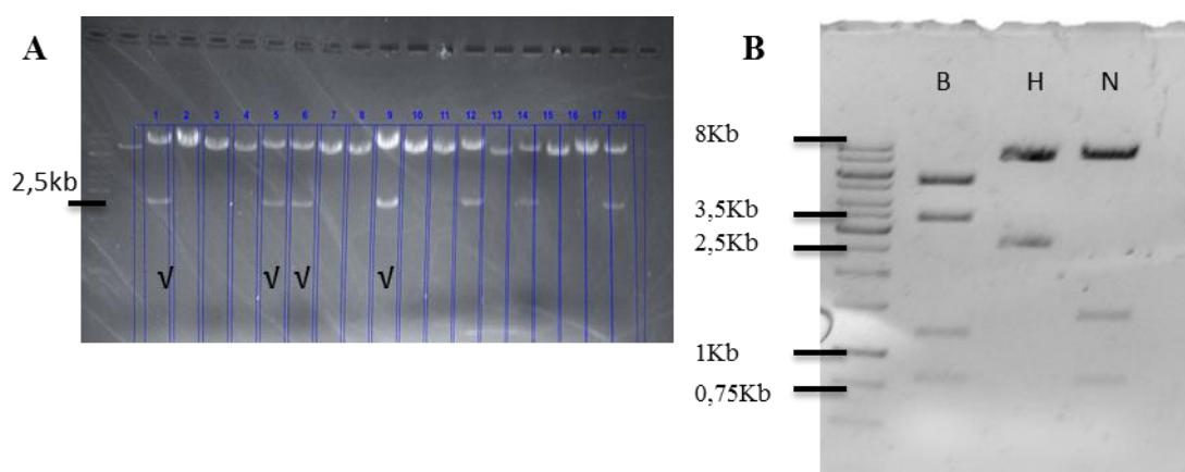
Fig. 6. A: Restriction digest of the 18 ENEAS clones with HindIII. Seven of the 18 clones presented the expected band of 2,5Kb. The marked clones were expanded and saved for further analysis.. B: Diagnostic restriction, cuts of Eneas with BamHI (B), HindIII (H) and NcoI (N). All the bands correspond to the expected sizes: B- 5,47Kb, 3,36Kb 1,19Kb and 0,796Kb; H- 8,22Kb and 2,2Kb; N- 8,6Kb, 1,39Kb and 0,798Kb.
