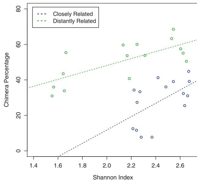
Figure 1. Chimera percentage and Shannon Index of closely and distantly related pools of nematodes.
