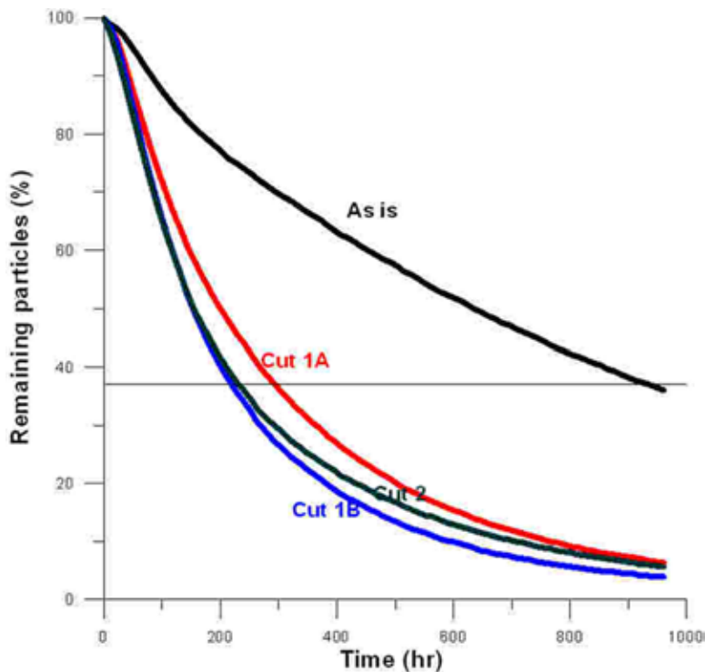
Figure 11. Time-series plot of the number of particles seeded in the shallows remaining in the shallows. Where the line intersects the 37% line is the Residence Time (RT) in the oceanographic convention. 'As is' is the present condition (RT = 37.5 days), Cuts (1A, 1B and 2) refer to the situation following channel dredging at the sites shown in Figure 7. Cut 1A consists of a dredged channel, 61 m wide and 2 m deep below LAT, and extending 130 m into the shallows (RT = 250 hours, 10.41 days). Cut 1B, is located at the same site but it is 86 m wide, and it extends 413 m into the shallows on a straight line (RT = 9.17 days). Cut 2 is a dredged channel just north of the marina, it is 86 m wide, 2 m deep below LAT, and extending 600 m into the shallows (RT = 9.58 days).
