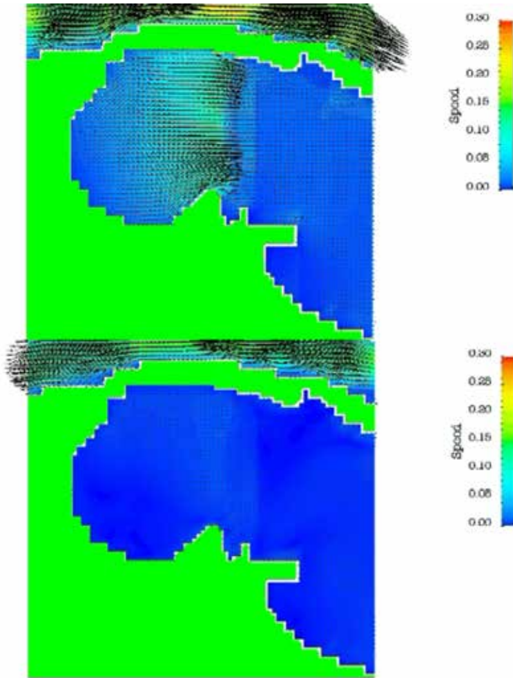
Figure 9. Snapshots of the currents over the shallows and Upper Luanda Bay and coastal waters at two different times of the tidal cycle in calm weather. The colour bar shows the speed in \text{m s}^{-1} .
