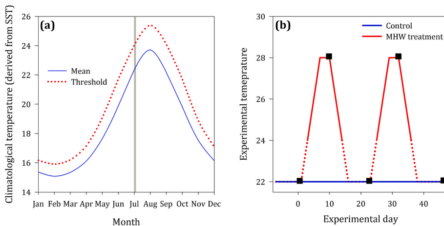
Fig. 3. Environmental and experimental temperature conditions. (a) Annual variation of long-term climatological daily mean and threshold temperatures in Punta de la Mona (southern Spain), retrieved from the Marine Heatwave Tracker, using the shifting baseline (1991–2020) (Schlegel, 2018). The starting point of the experiment is indicated by the grey line. (b) Experimental treatments (target temperatures), including a Control at 22 °C and a MHW treatment, simulating two consecutive summer MHWs (highlighted by a solid red line that indicate temperature above long-term climatological threshold), with a maximum intensity of 4 °C above threshold (i.e., strong event), a duration of 10 days each, and 12 days between MHW events. Black squares indicate time points at which physiological measurements were taken. (For interpretation of the references to colour in this figure legend, the reader is referred to the Web version of this article.)
