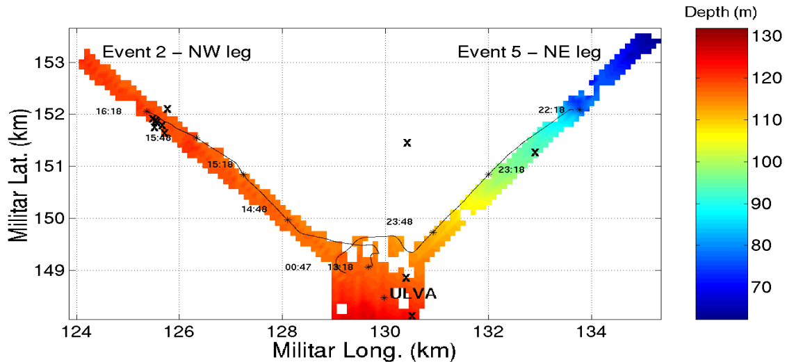
Figure 1: INTIFANTE'00 sea trial site bathymetry with XBT locations (marked \times ) and acoustic tracks for events 2 and 5.
