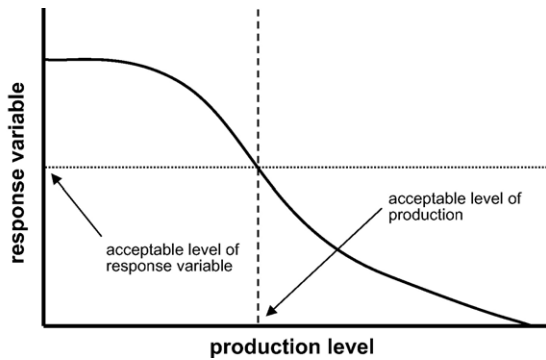
Fig. 2. Hypothetical response curve of an environmental variable under the influence of varying levels of bivalve culture production. The dotted line indicates the level of the indicator that has been determined to be acceptable by managers and the dashed line the corresponding level of production (i.e., the social carrying capacity ).
