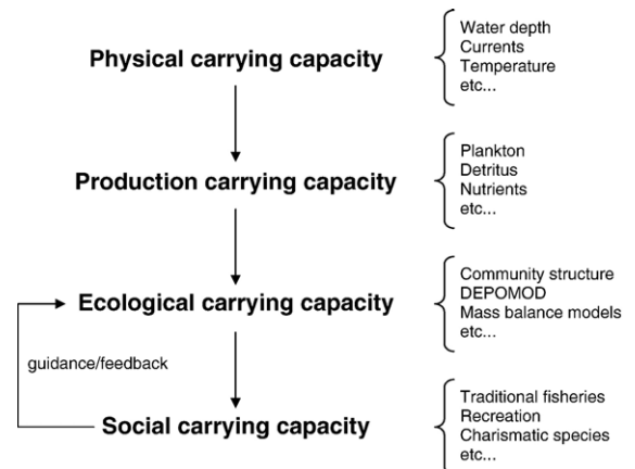
Fig. 1. Hierarchical structure to determine carrying capacity of a given area. Note that social carrying capacity feeds back directly to ecological carrying capacity to provide guidance to choose pertinent response variables to measure.
