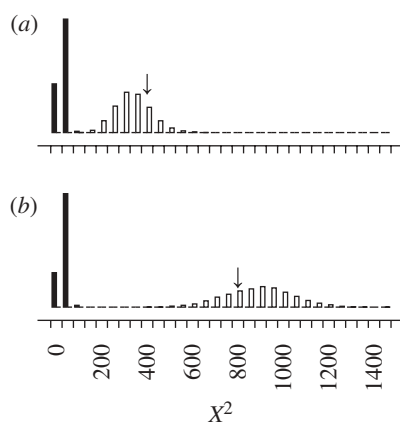
Figure 3. Assessment of model composition fit by posterior predictive simulation for the rRNA analysis. The test quantity was \chi^2 ( sensu Sokal & Rohlf 1981), the statistic used in \chi^2 tests. Data sets were simulated based on samples from the posterior distribution and for each the \chi^2 was calculated. Black bars show the distribution for a tree-homogeneous model, and white bars show the distribution for a tree-heterogeneous NDCH model with two composition vectors on each data partition. Panel (a) shows distributions for the SSU partition and panel (b) shows distributions for the LSU partition. Arrows show the \chi^2 for the original data, showing that by this test two composition vectors for each data partition are needed to adequately model the data.
