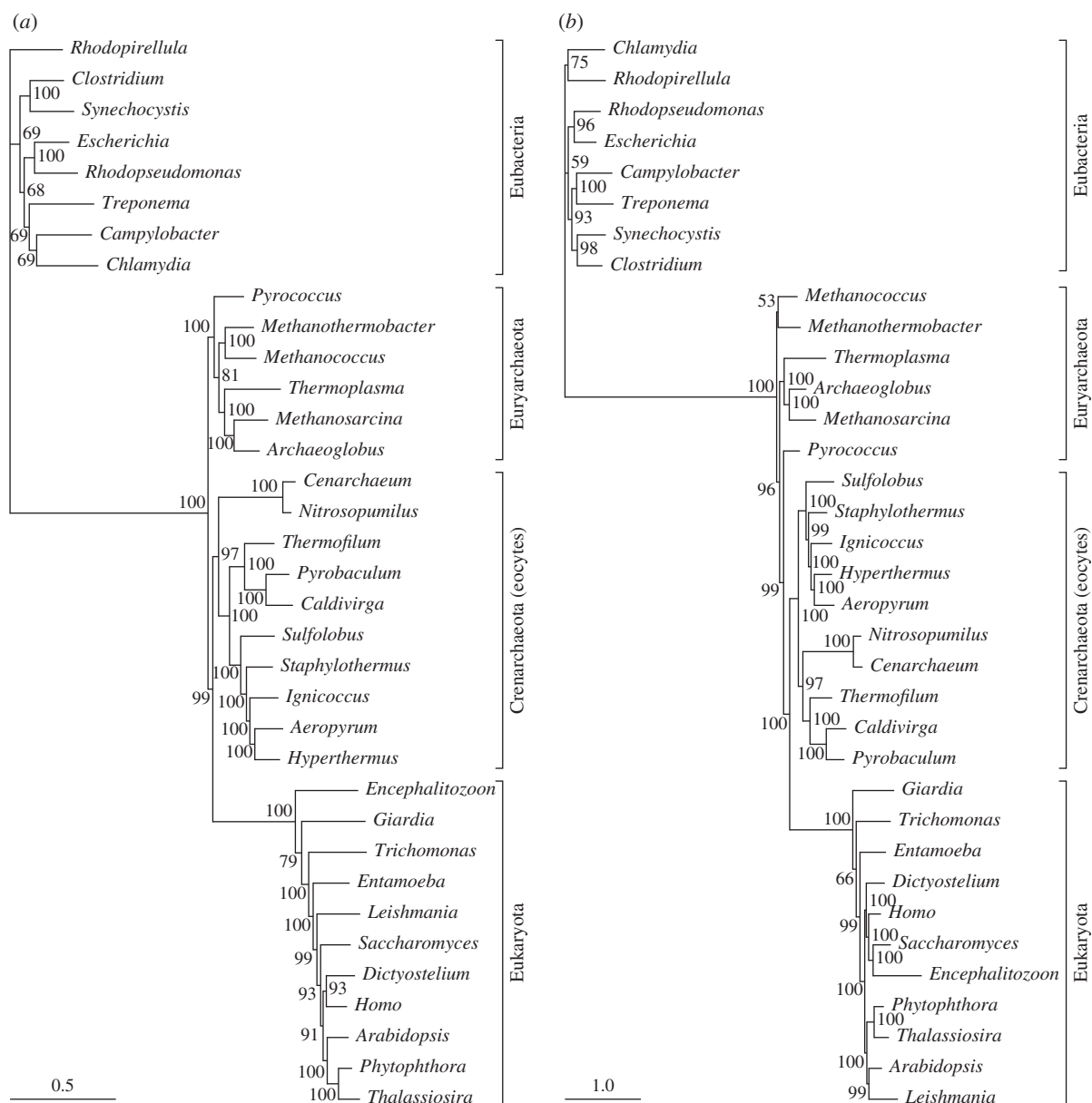
Figure 4. Bayesian phylogenetic analyses of concatenated amino acid data. The analysis in panel (a) used Dayhoff-recoded data with a GTR + \Gamma + NDCH(14) tree-heterogeneous substitution model in p4 . This is the analysis summarized in table 3, row I. The analysis shown in panel (b) used standard amino acid-coded data with a CAT-Poisson + \Gamma substitution model in PHYLOBAYES . This is the analysis summarized in table 3, row F.
